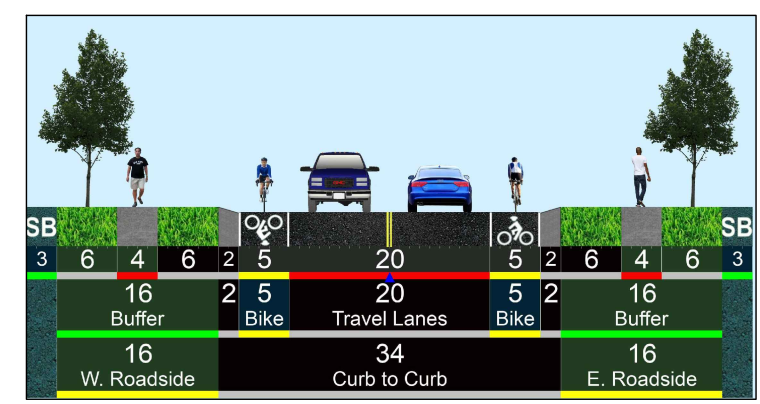
PROPOSED TYPICAL STREET LAYOUT STATION 12+32 TO 24+77
