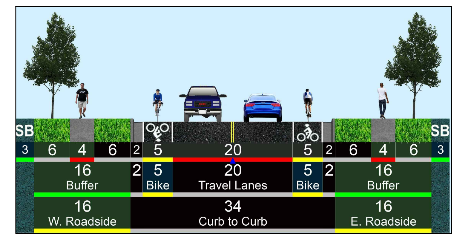
PROPOSED TYPICAL STREET LAYOUT STATION 12+32 TO 24+77
