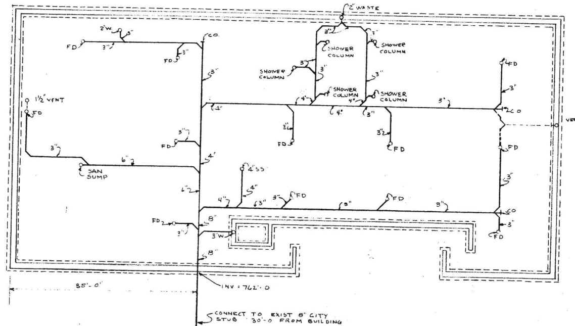
FOUNDATION PLAN-REVISED PLUMBING PLAN
