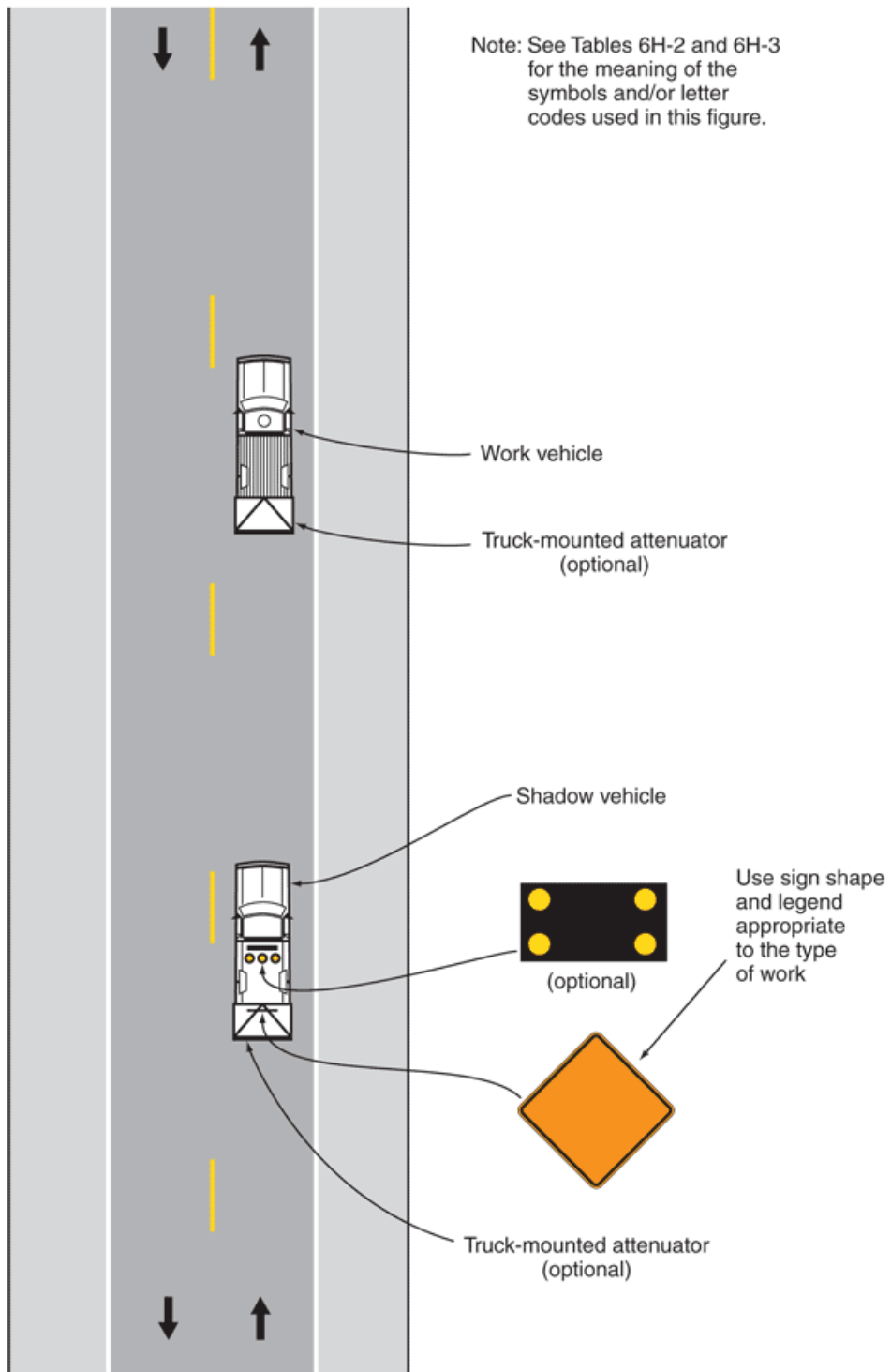
Typical Application 17
