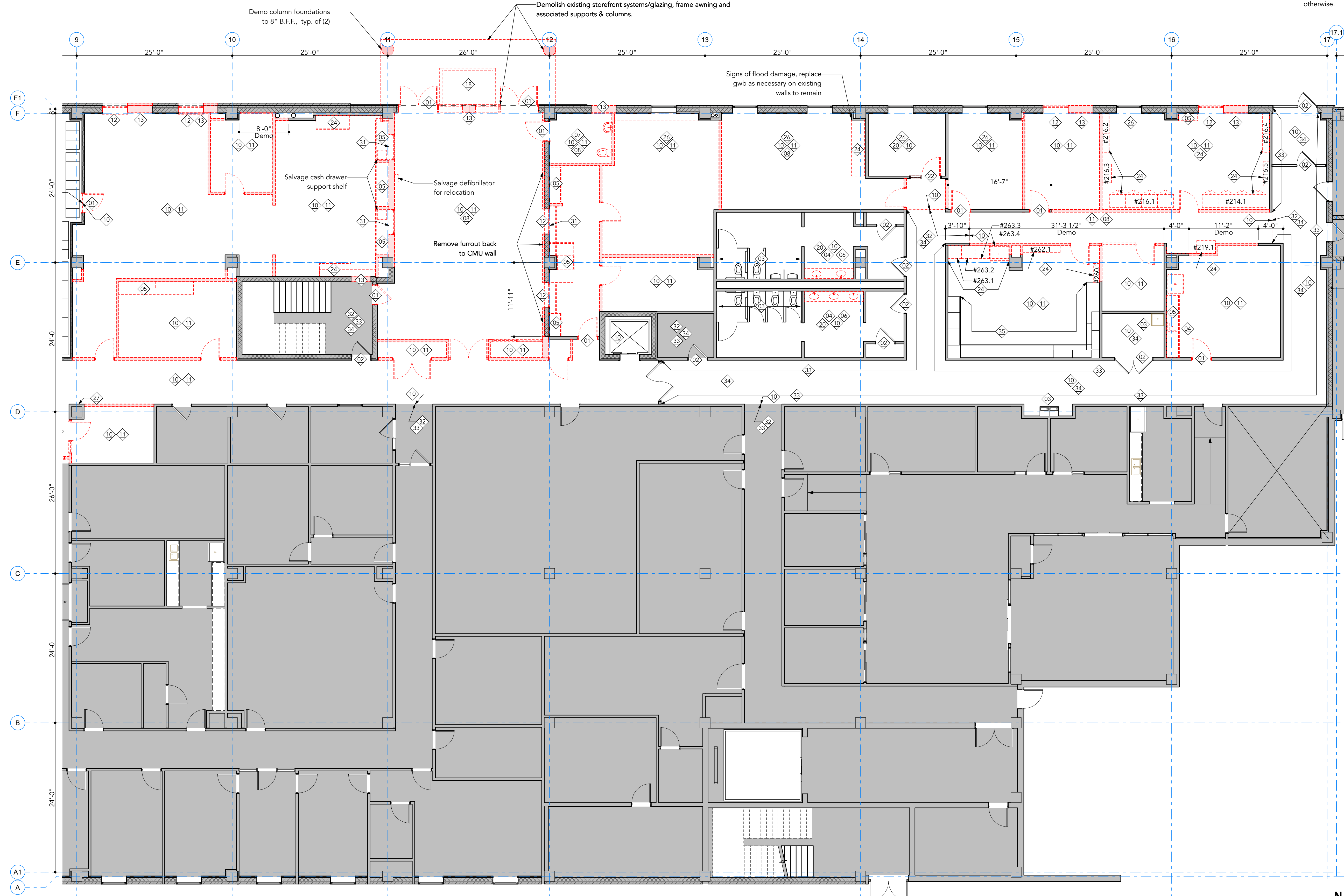
1 Demolition Main Level Plan SCALE: 1/8" = 1'-0"
