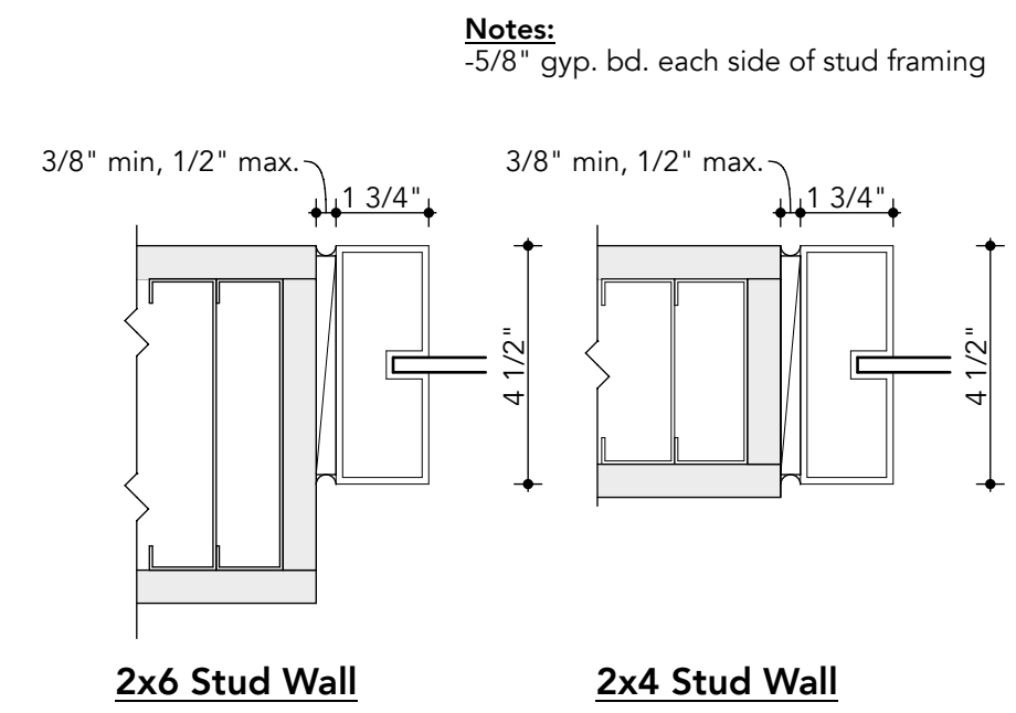
9 Typical Aluminum Window Jamb Interior A403 SCALE: 3" = 1'-0"
