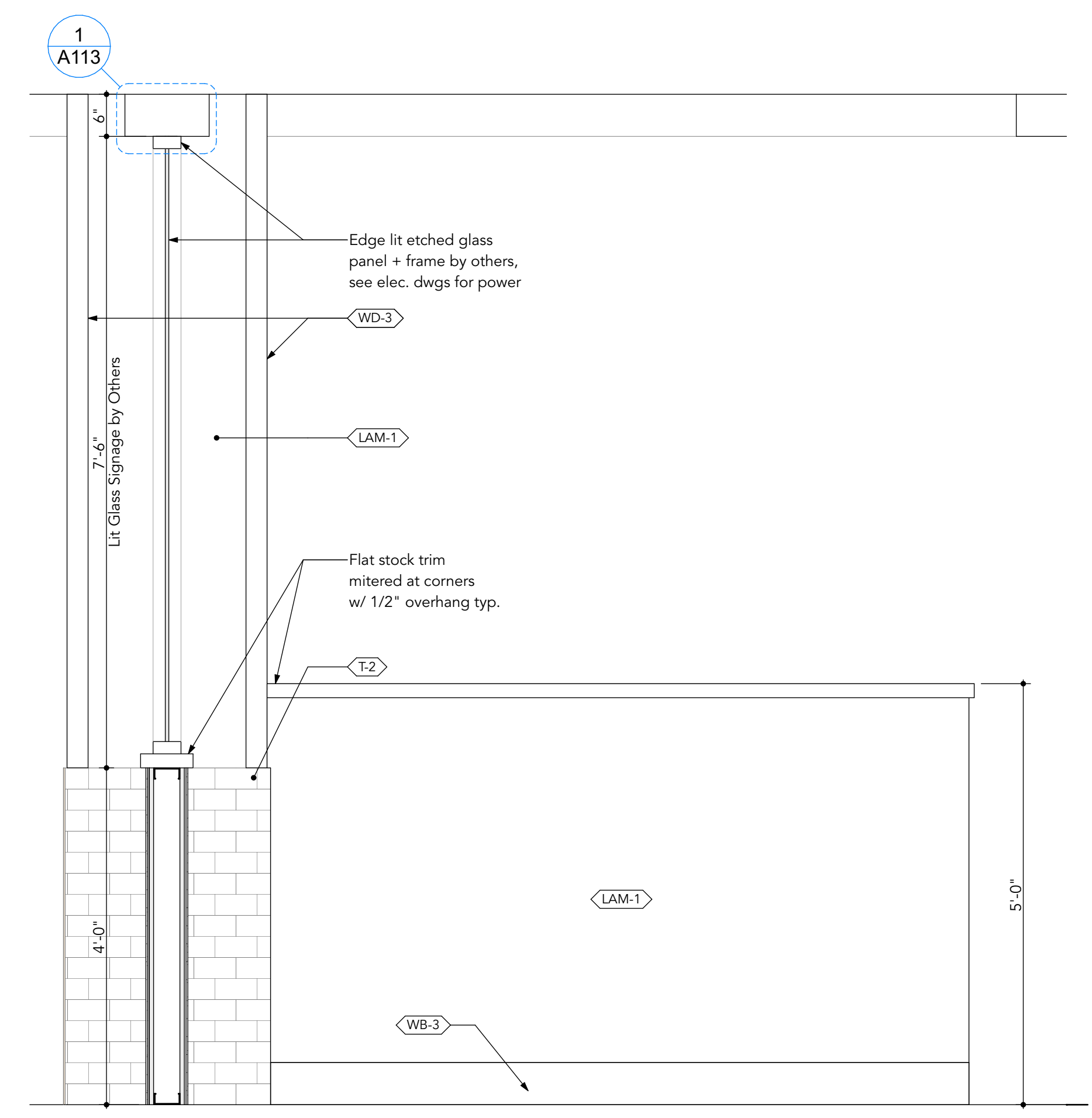
1 Lobby Wall Section A308 SCALE: 3/4" = 1'-0"
