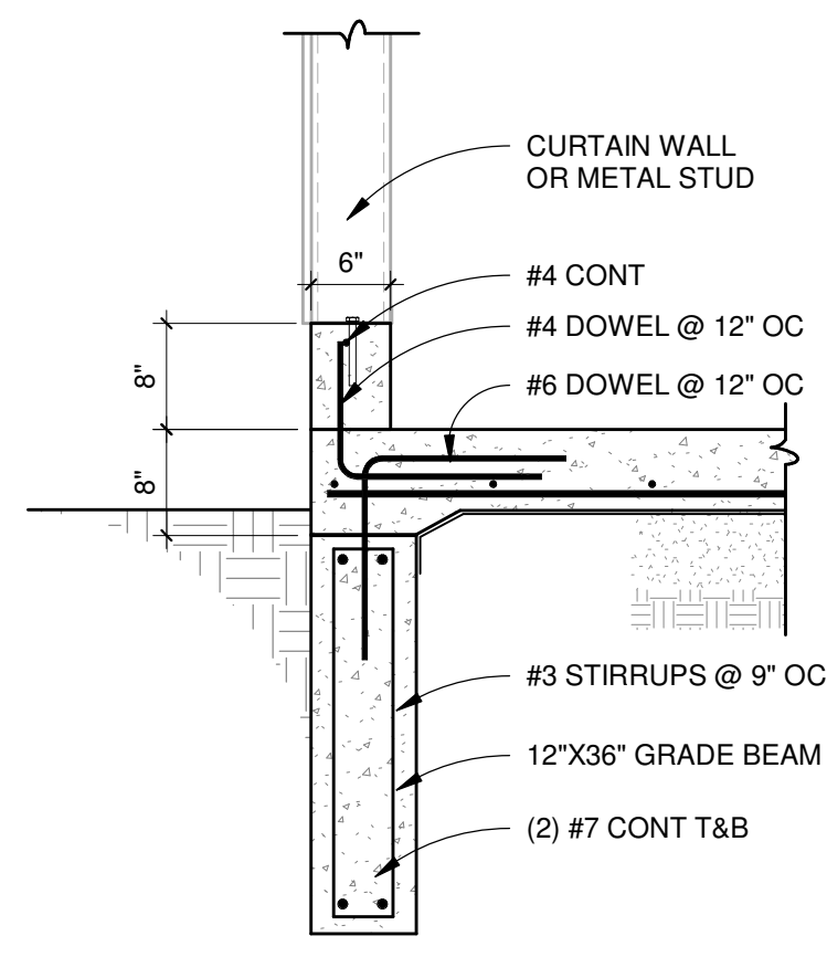
8 S201 TYPICAL EXTERIOR GRADE BEAM SCALE: 3/4" = 1'-0"
