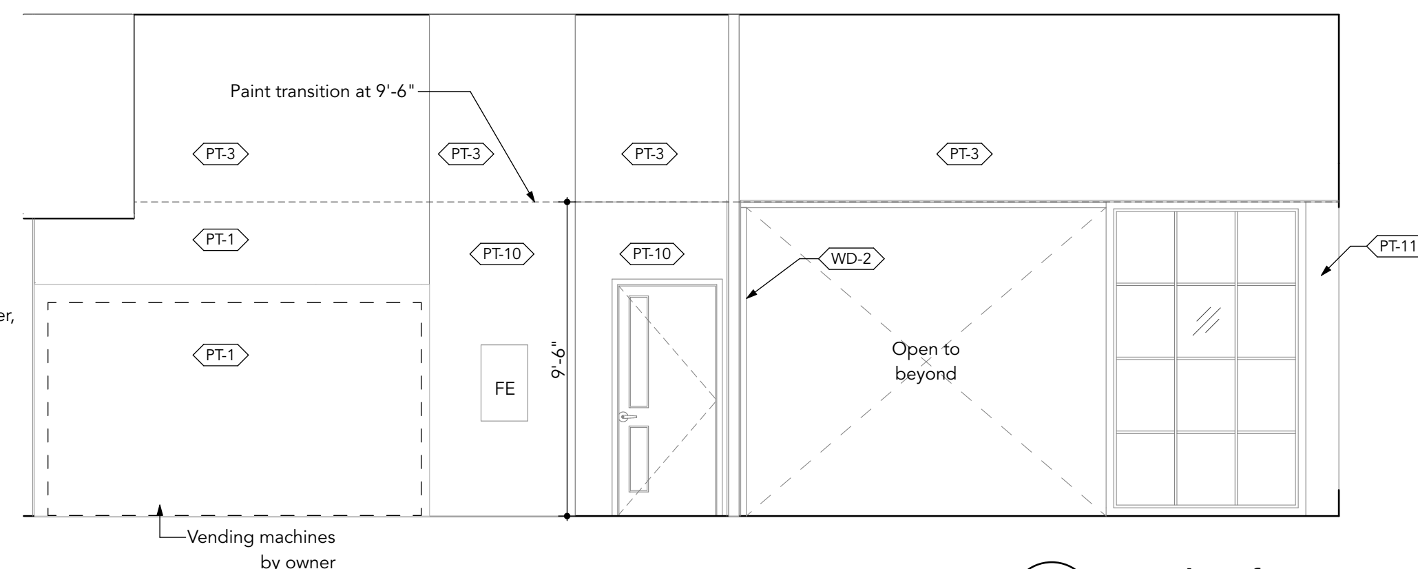
1 Work Cafe 195 West 1203 SCALE: 1/4" = 1'-0"
