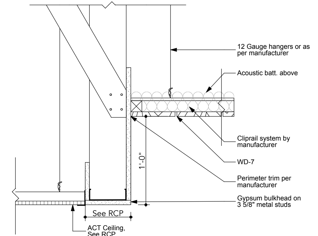
5 Connect 182 Wood Ceiling Detail A113 SCALE: 1 1/2" = 1'-0"
