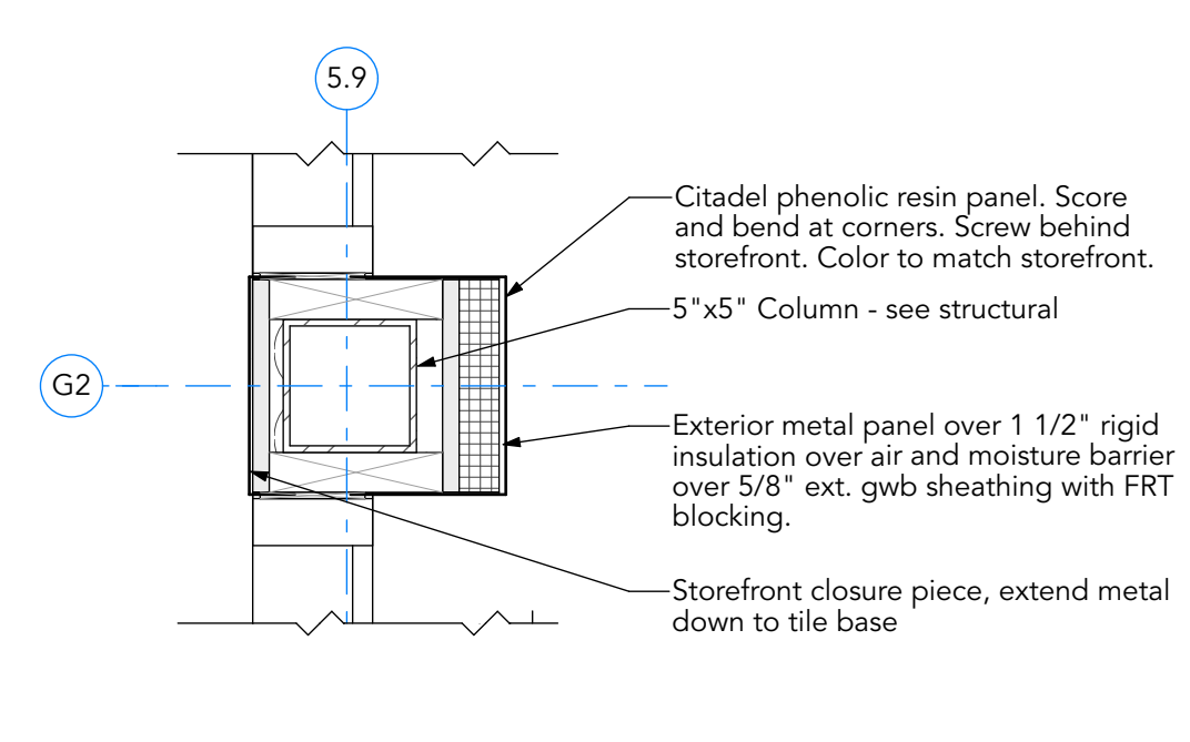
1 Entry Canopy Wall @ Column Plan A307 SCALE: 1 1/2" = 1'-0"
