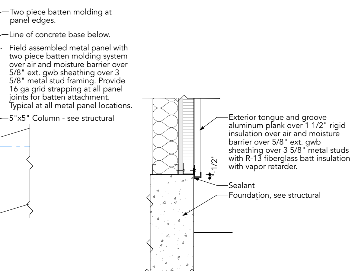
4 Entry to Existing Wall Section Detail A307 SCALE: 1 1/2" = 1'-0"
