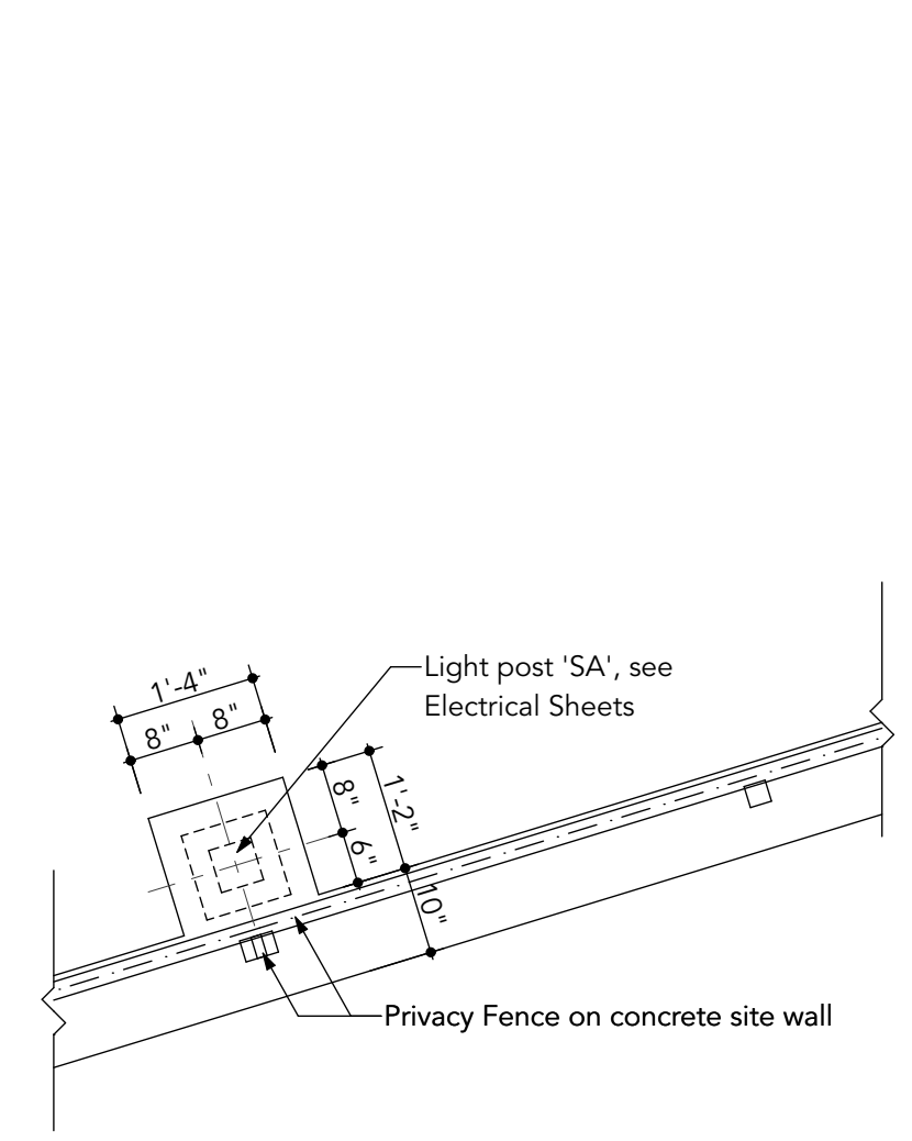
5 Site Wall Plan Detail AS01 SCALE: 1/2" = 1'-0"
