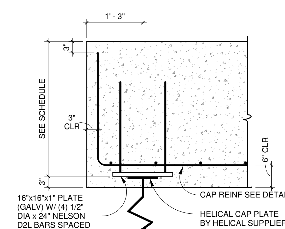
14 S201 PIER WELD PLATE DETAIL SCALE: 3/4" = 1'-0"
