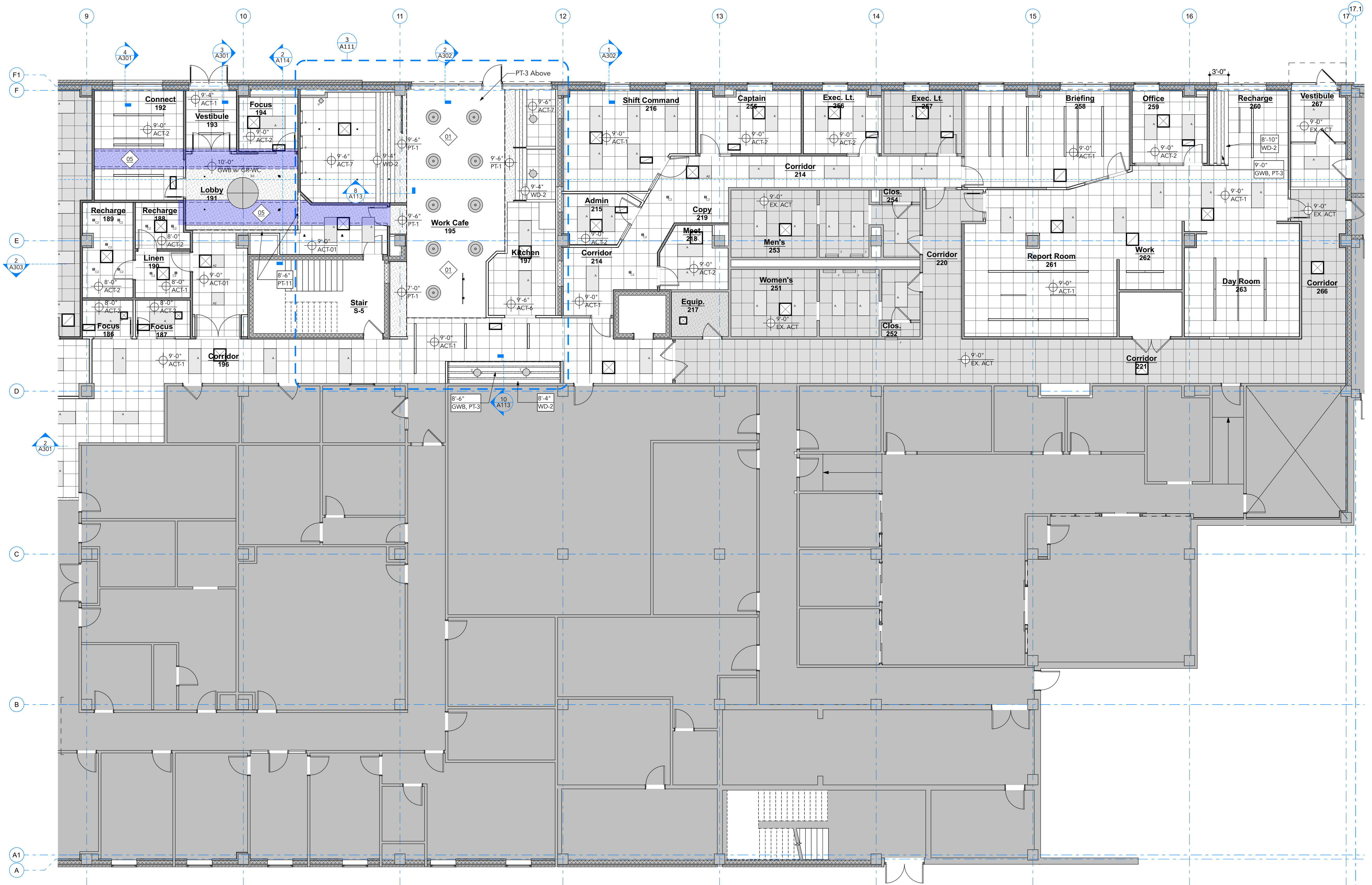
1 Reflected Ceiling Main Level Plan A108 SCALE: 1/8" = 1'-0"
