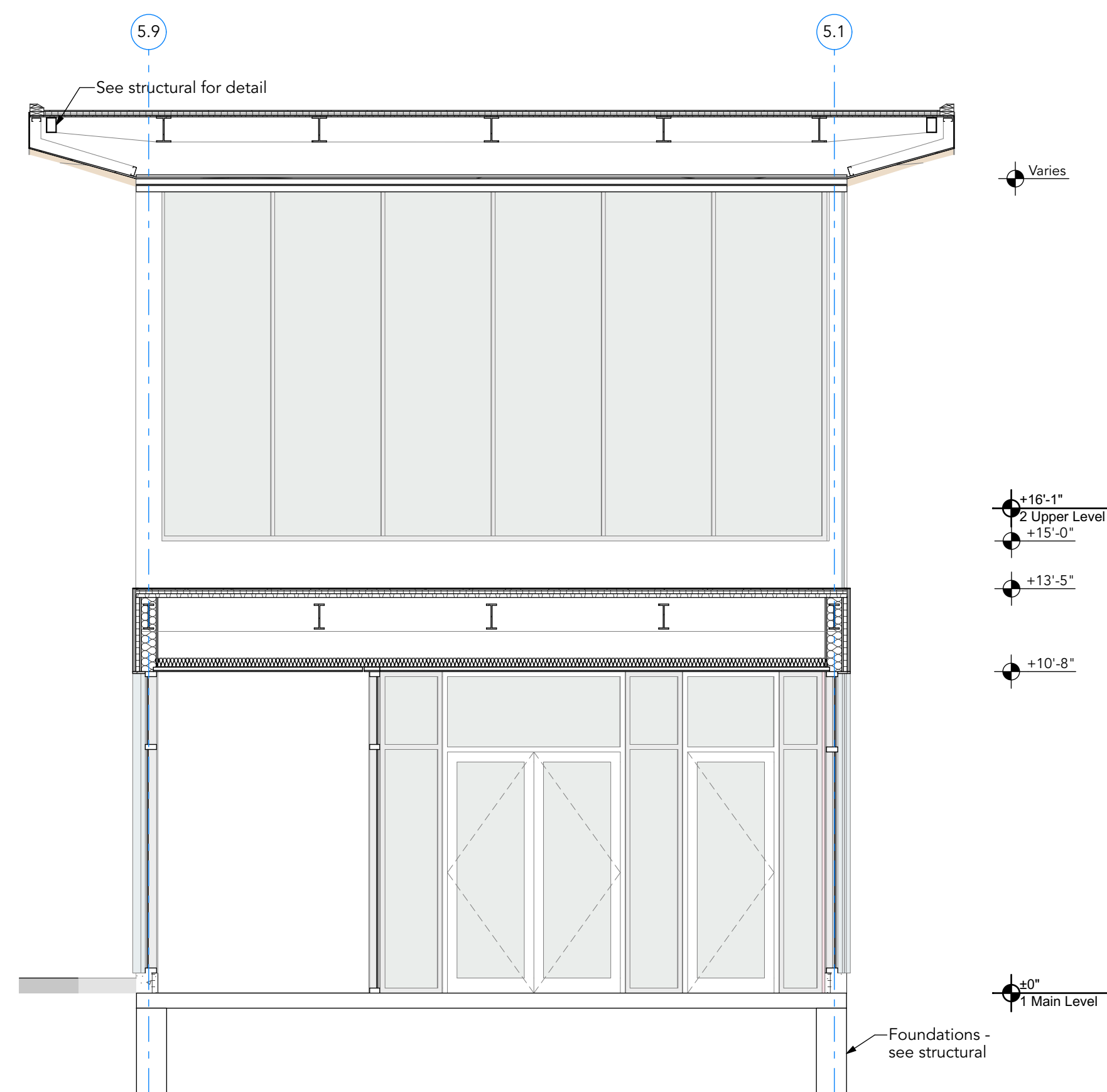
2 Building Section
