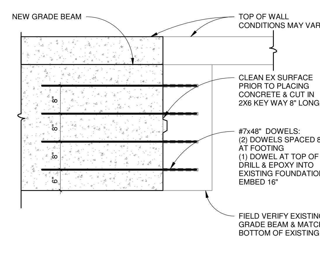
9 S201 FOUNDATION DETAIL AT EXISTING GRADE BEAM SCALE: 3/4" = 1'-0"
