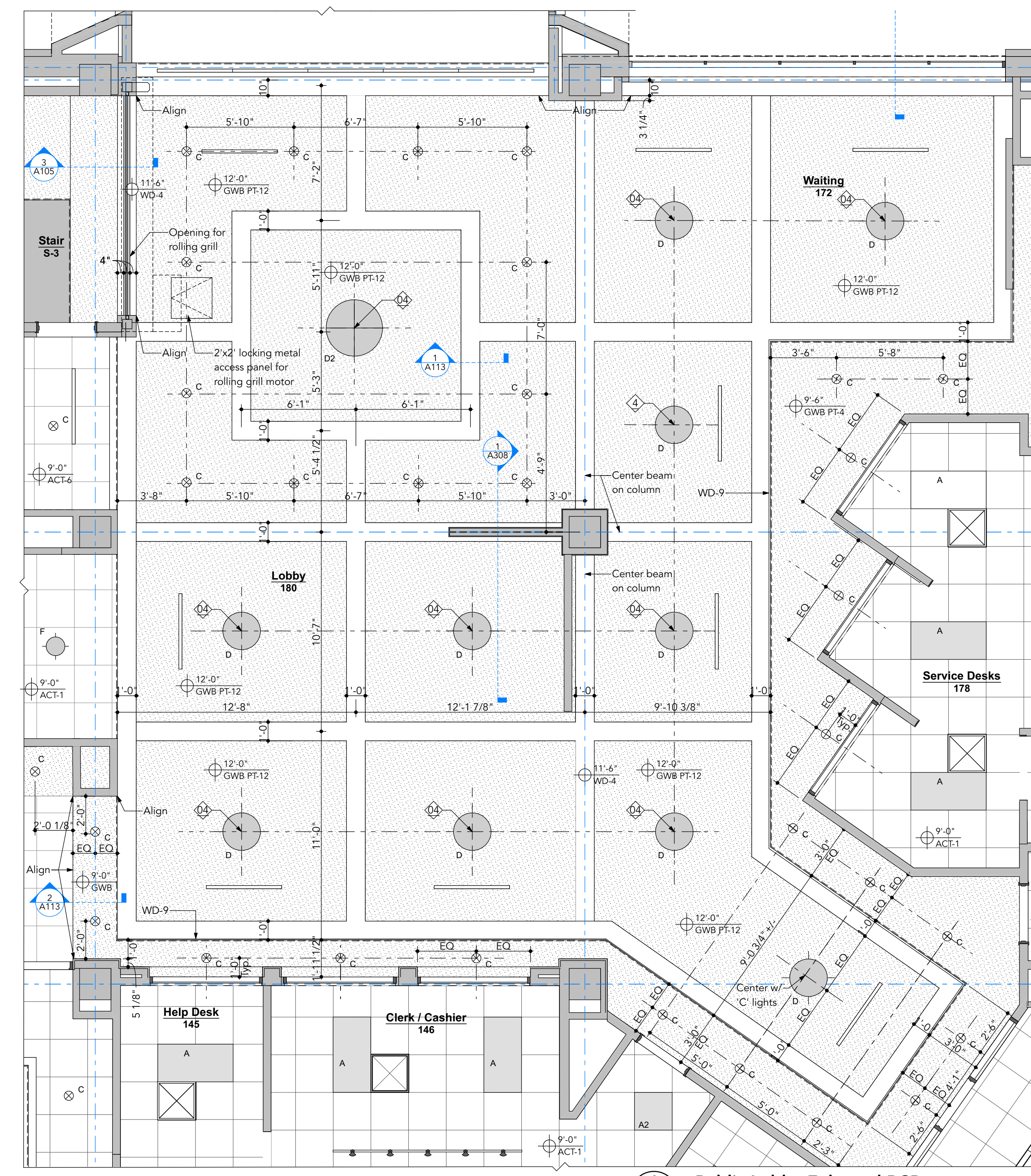
1 Public Lobby Enlarged RCP A111 SCALE: 1/4" = 1'-0"
