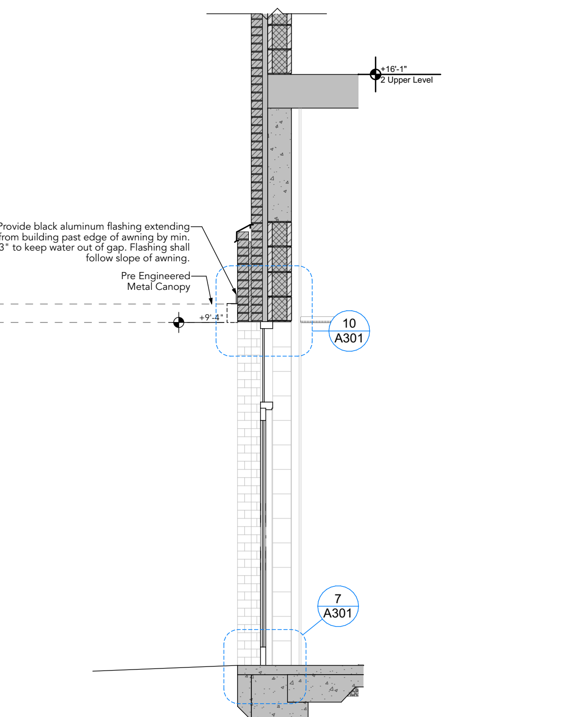
3 Storefront Door @ Awning & Metal Panel A301 SCALE: 3/8" = 1'-0"
