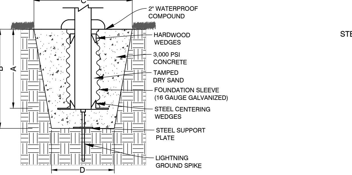
FLAG POLE DETAIL C3.0 NOT TO SCALE
