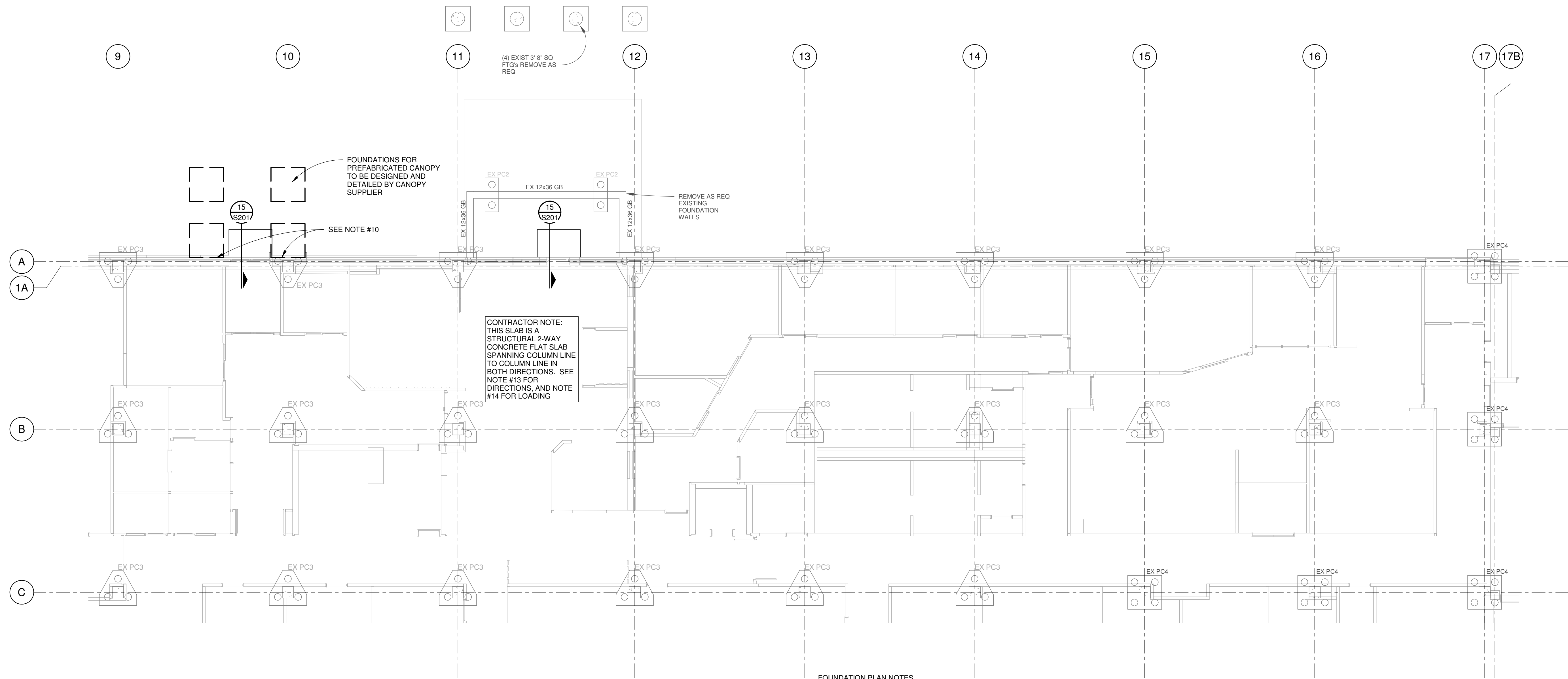
FOUNDATION PLAN - ZONE B SCALE: 1/8" = 1'-0"
