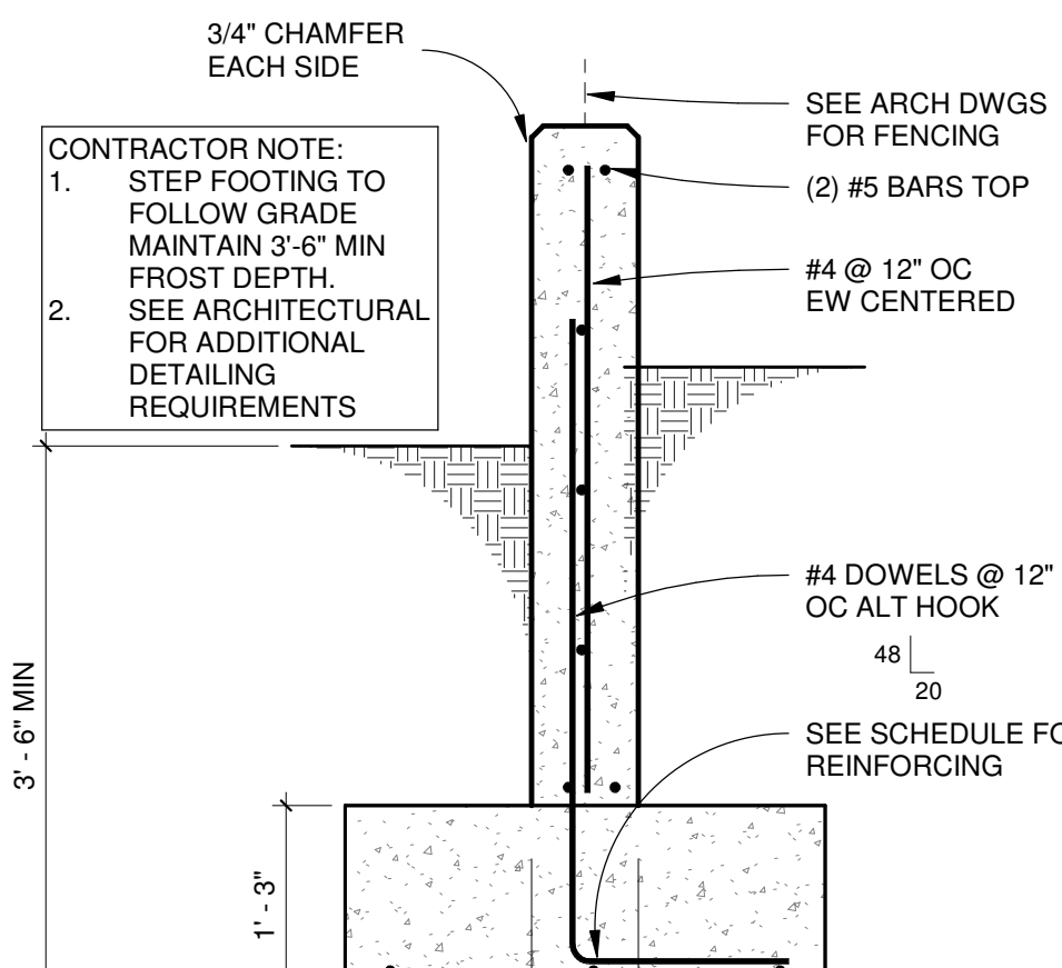
13 S201 TYPICAL RETAINING WALL SCALE: 3/4" = 1'-0"
