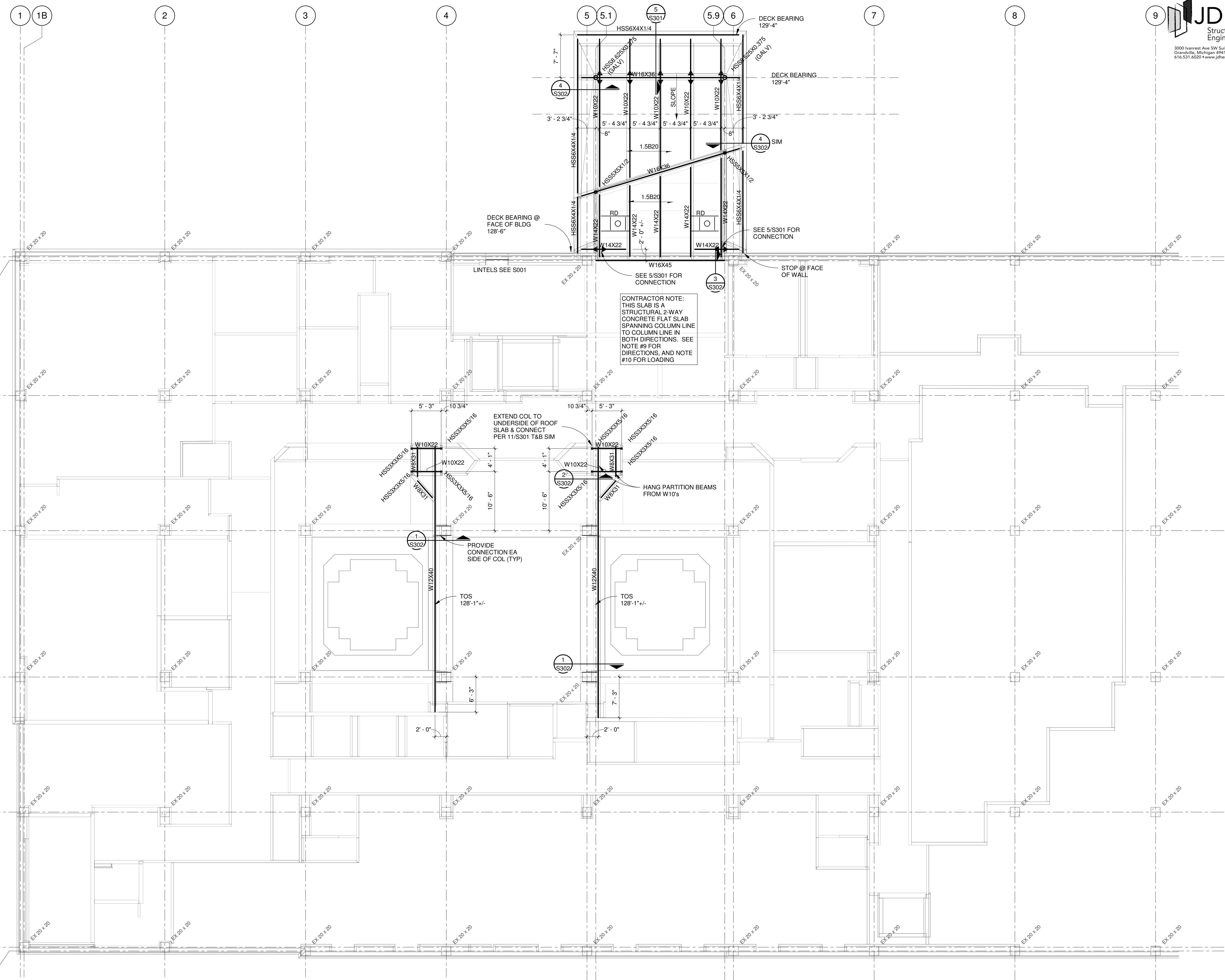
ROOF FRAMING PLAN - ZONE A SCALE: 1/8" = 1'-0"
