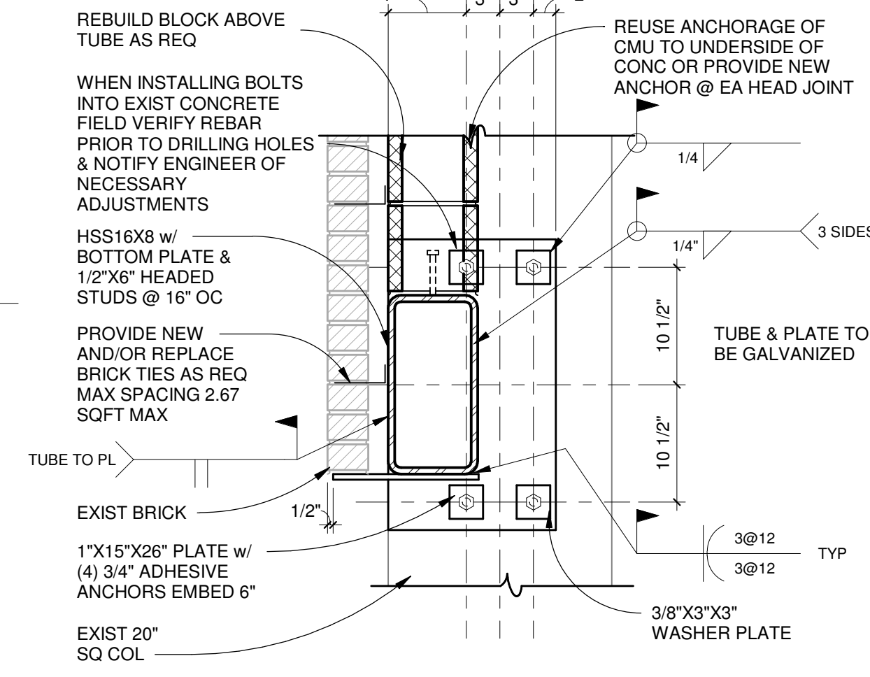
5 S302 FRAMING DETAIL SCALE: 1" = 1'-0"
