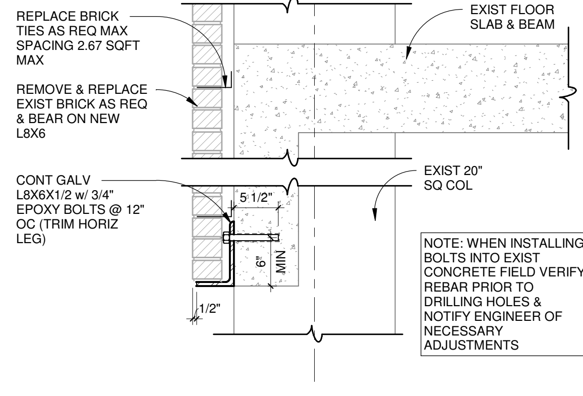
6 S302 FRAMING DETAIL SCALE: 1" = 1'-0"
