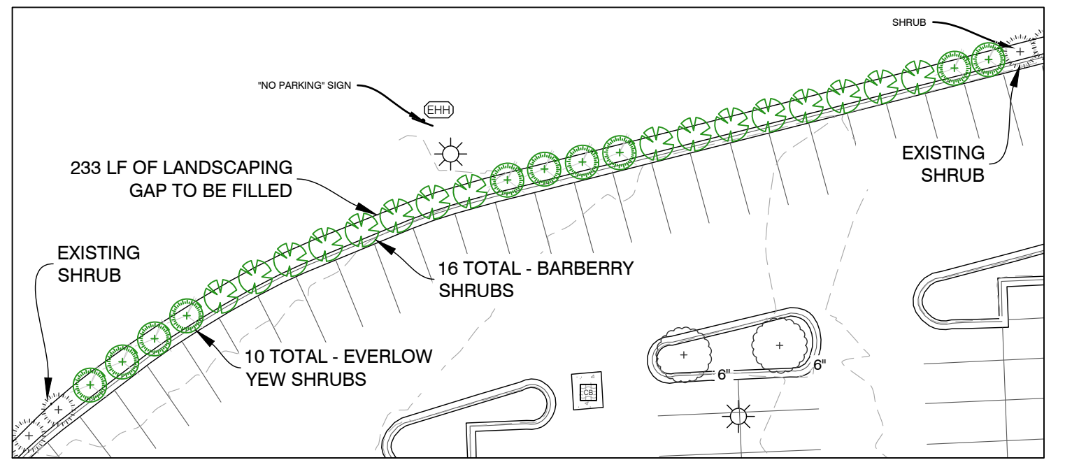
CROSSTOWN PKWY FRONTAGE LANDSCAPING DETAIL C3.0 1 INCH = 30 FEET
