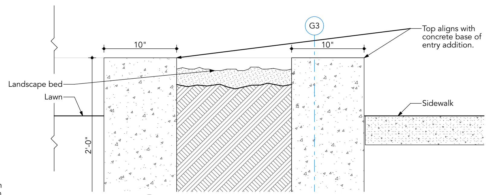
10 Entry Canopy Arm Section Detail A307 SCALE: 1 1/2" = 1'-0"
