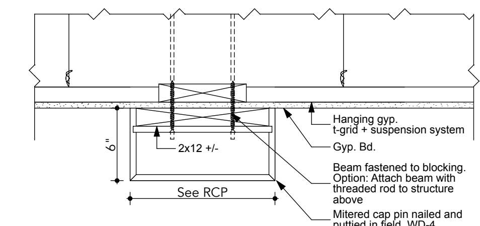
1 Lobby Ceiling Detail A113 SCALE: 1 1/2" = 1'-0"
