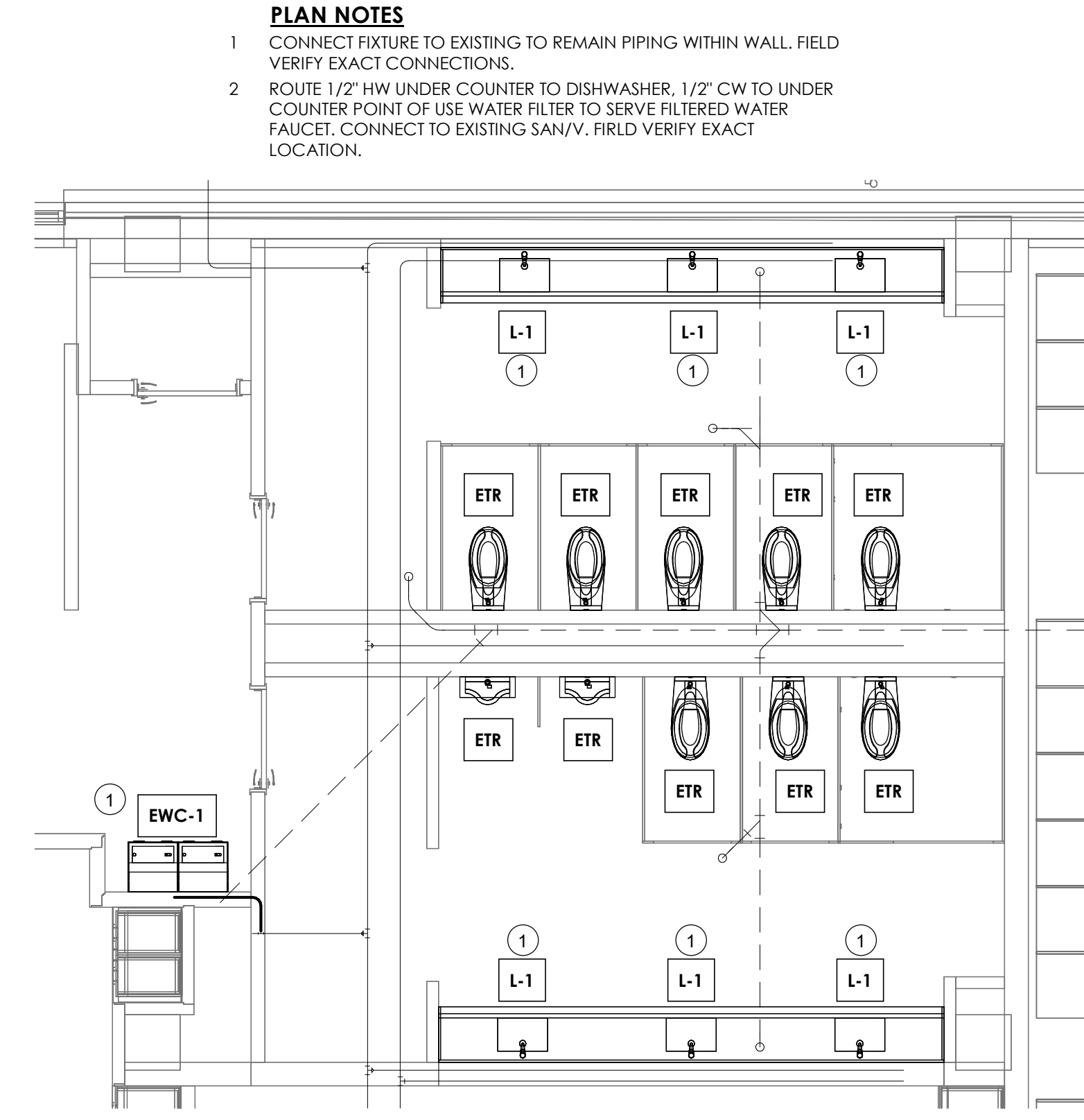
2 MAIN LEVEL CPED NORTH RESTROOM P401 1/4" = 1'-0"
