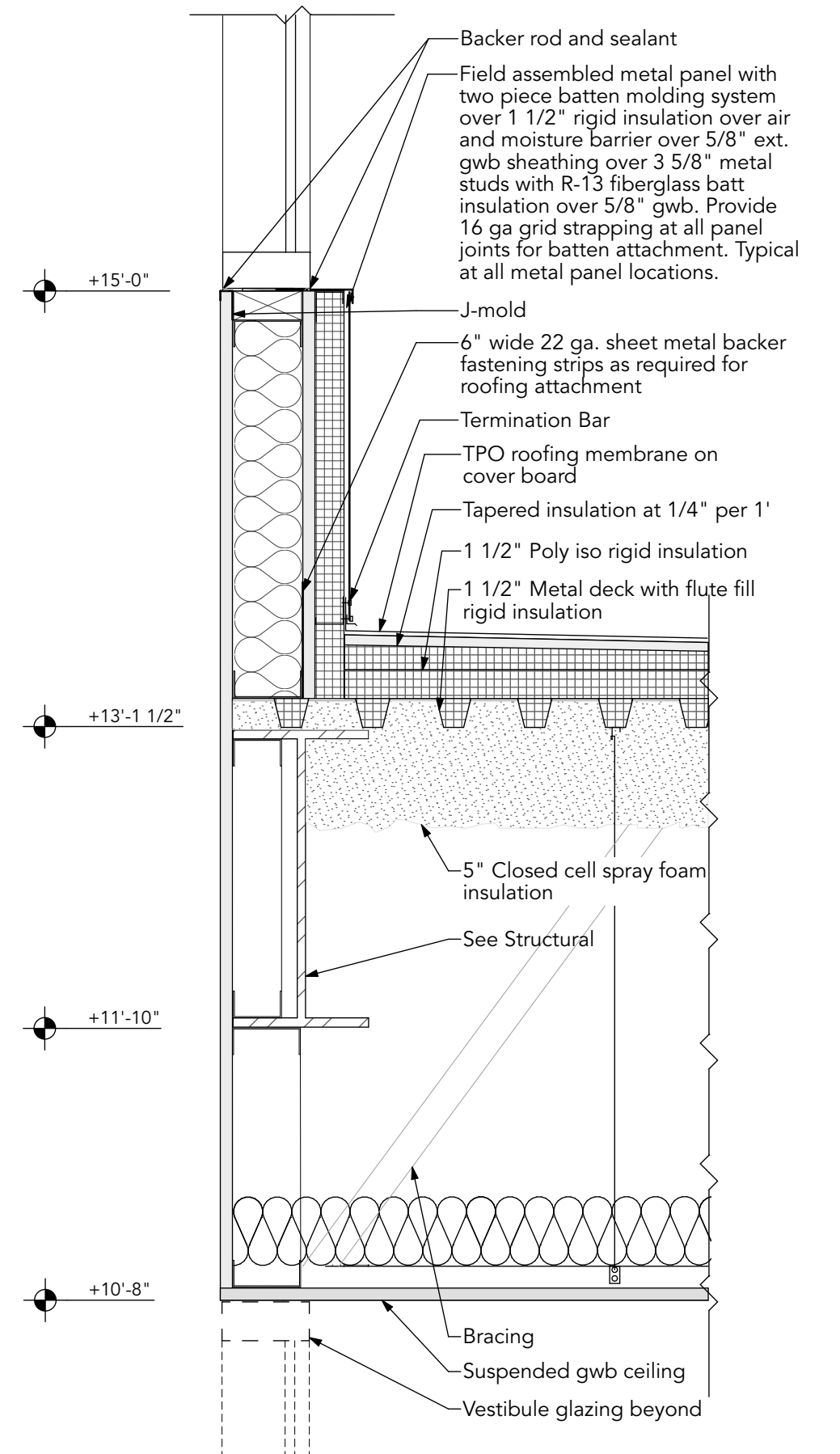
4 Entry Canopy @ Lower Roof to Wall Detail A306 SCALE: 1 1/2" = 1'-0"
