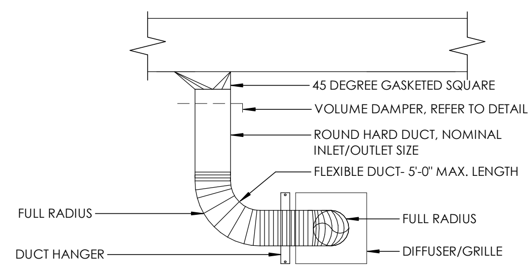
12 DUCT DIFFUSER CONNECTION M501 NOT TO SCALE
