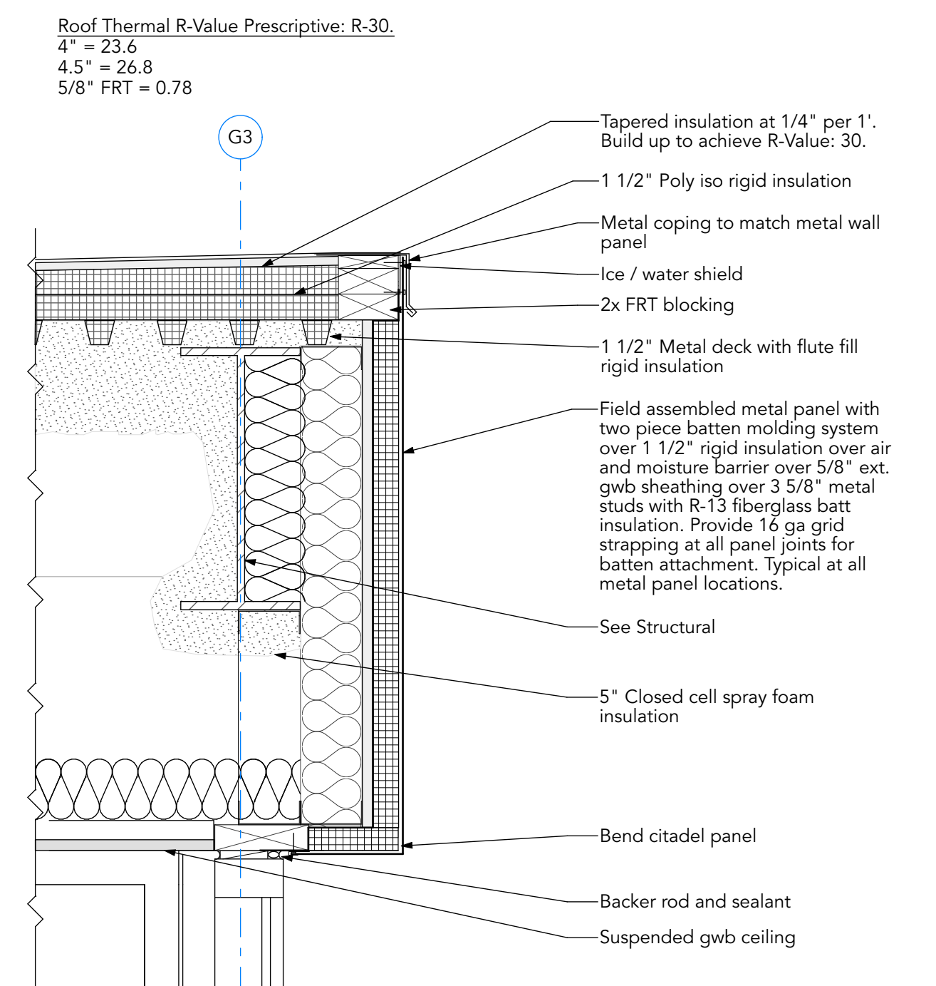
3 Entry Canopy @ Lower Roof Edge Detail A306 SCALE: 1 1/2" = 1'-0"
