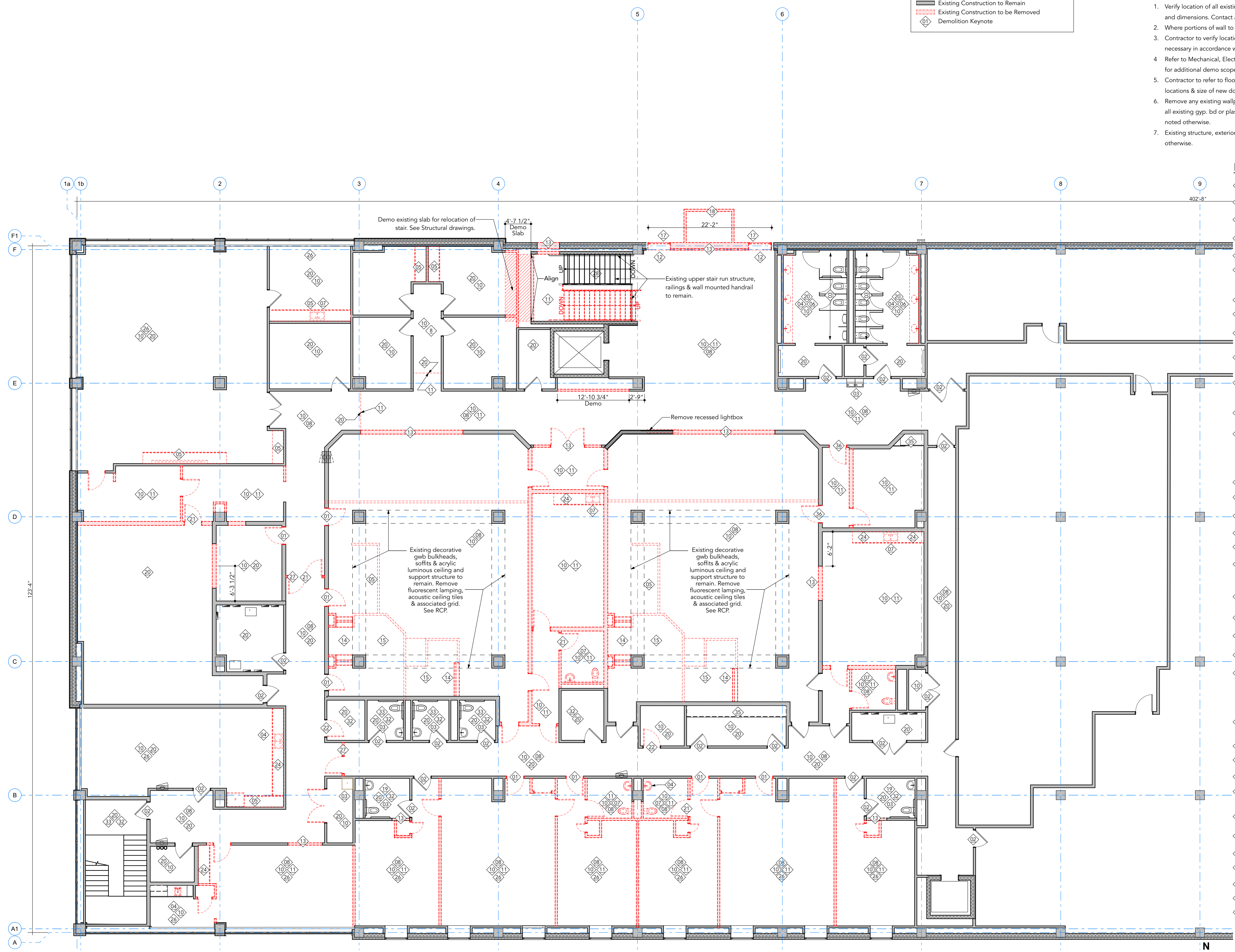
1 Demolition Upper Level Plan A003 SCALE: 1/8" = 1'-0"
