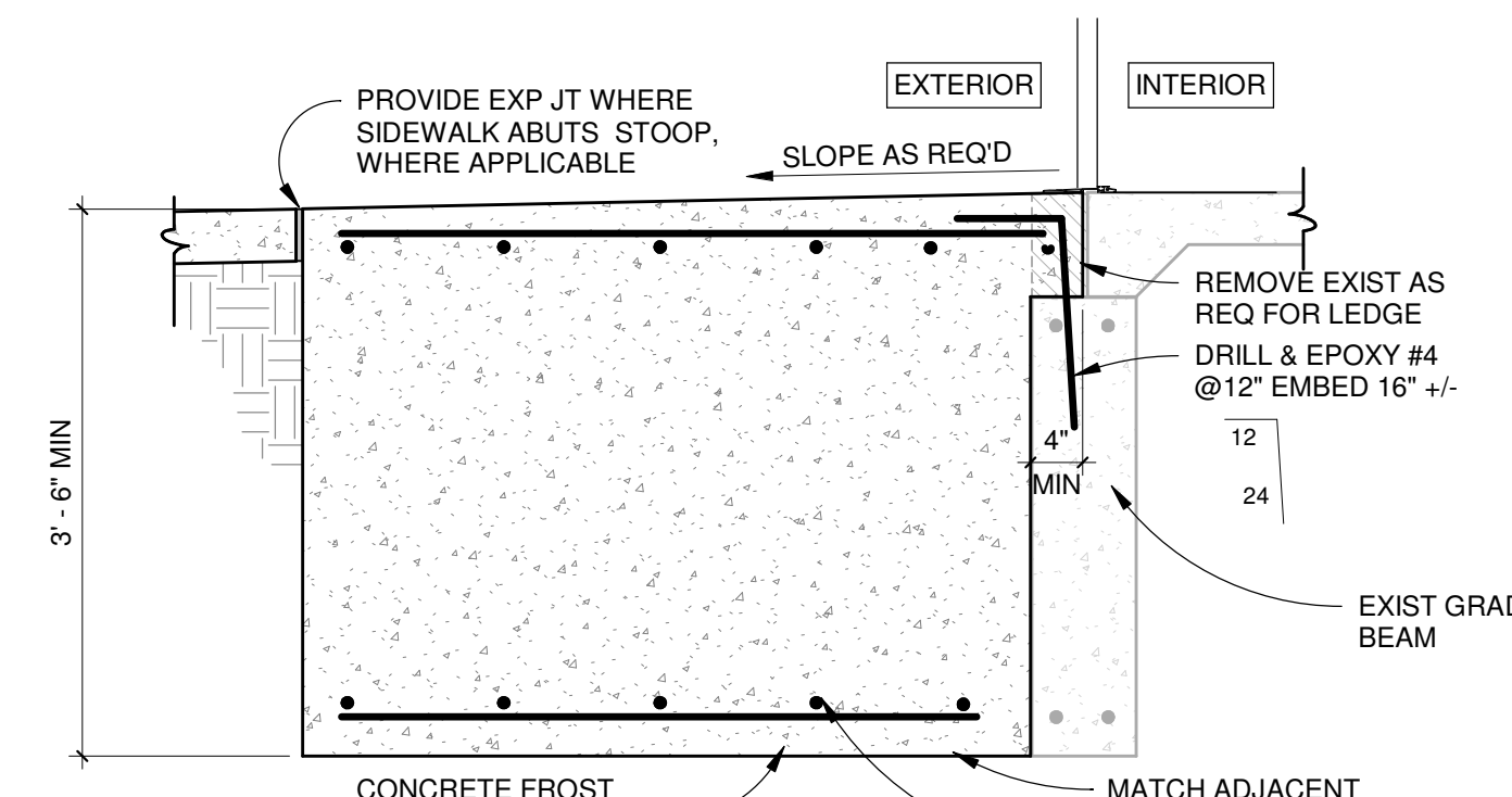
15 S201 FROST PROTECTED DOOR THRESHOLD DETAIL SCALE: 3/4" = 1'-0"
