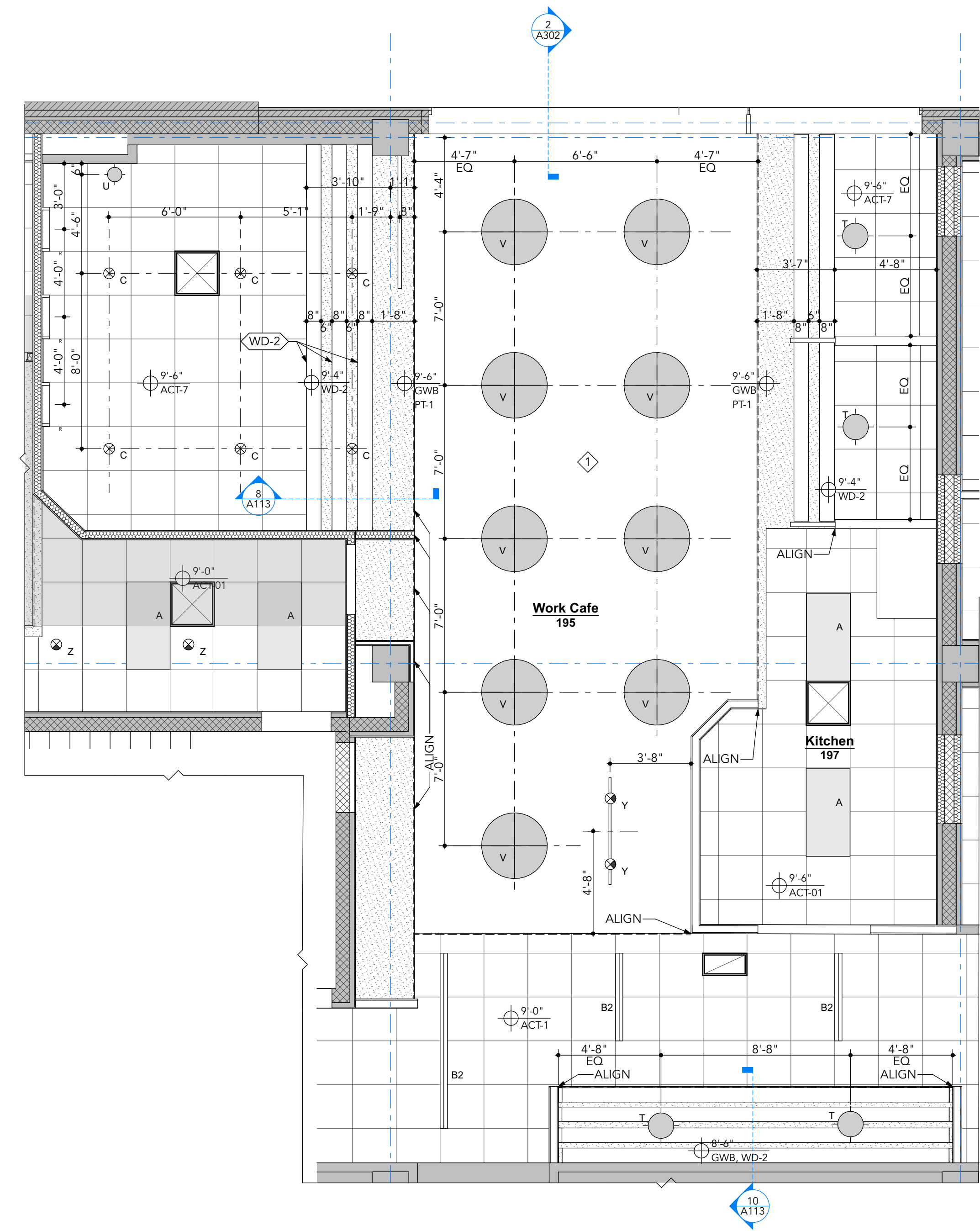
3 Work Cafe Enlarged RCP A111 SCALE: 1/4" = 1'-0"
