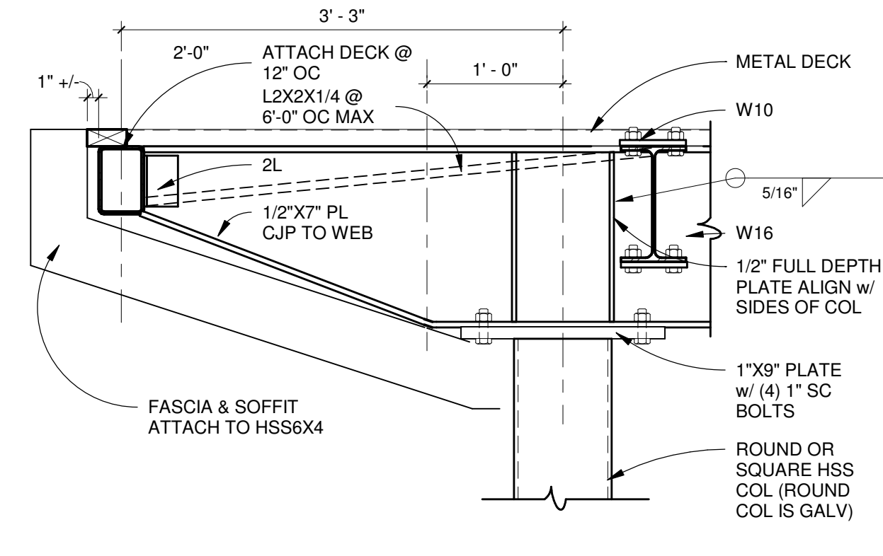
4 S302 FRAMING DETAIL SCALE: 1" = 1'-0"
