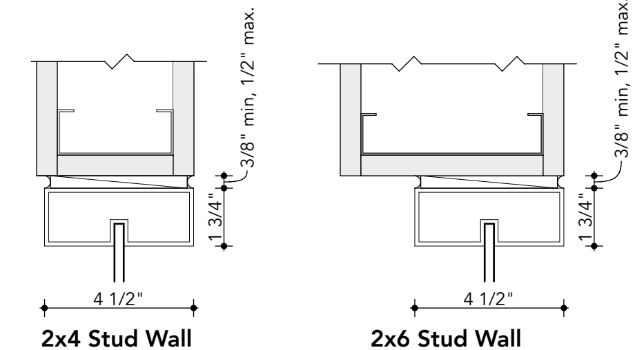
8 Typical Aluminum Window Head Interior A403 SCALE: 3" = 1'-0"
