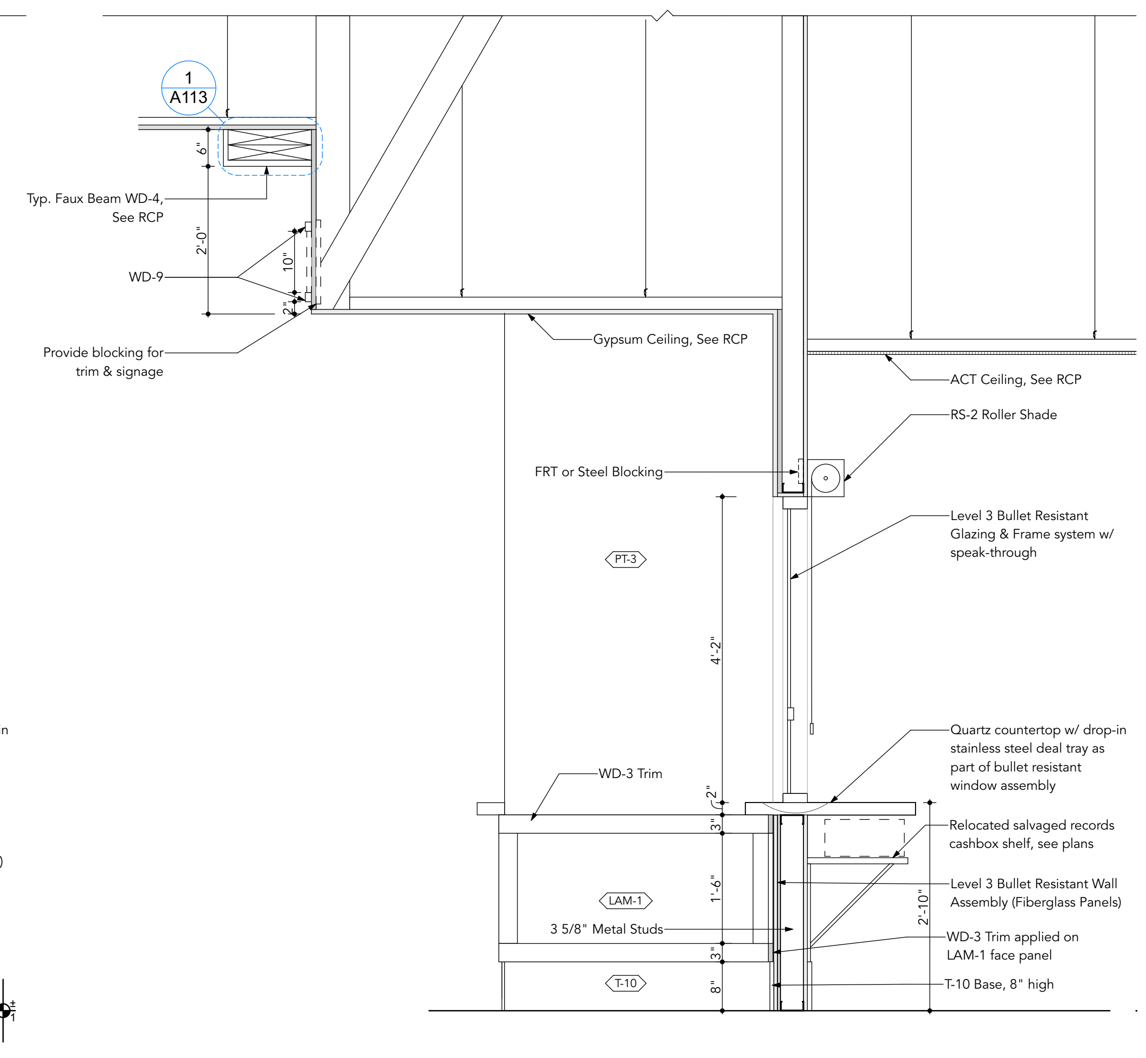
2 Service Desk Section - Records A308 SCALE: 3/4" = 1'-0"
