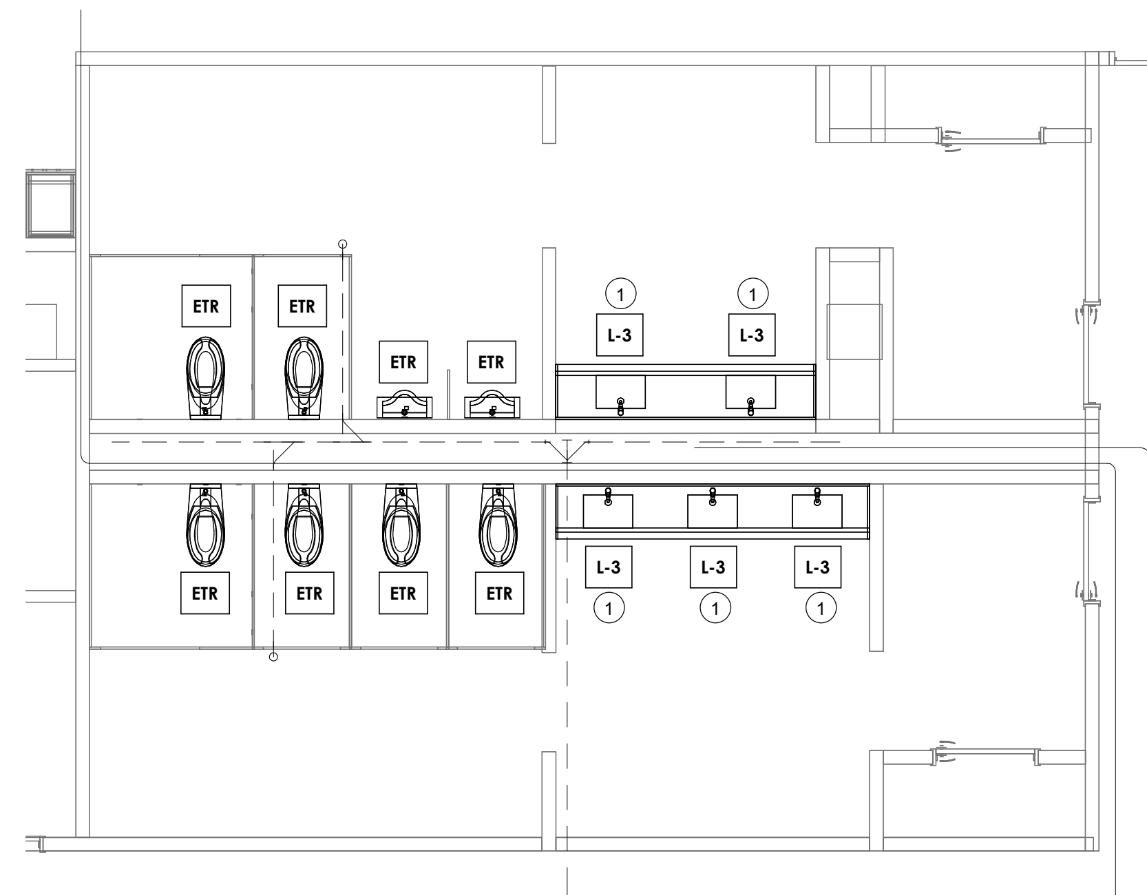
3 MAIN LEVEL KDPS RESTROOM P401 1/4" = 1'-0"
