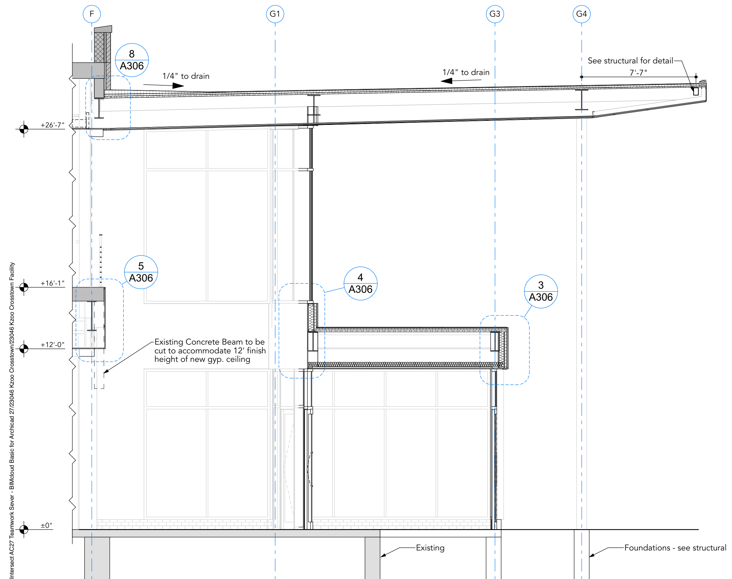
3 Canopy Section - Transverse
