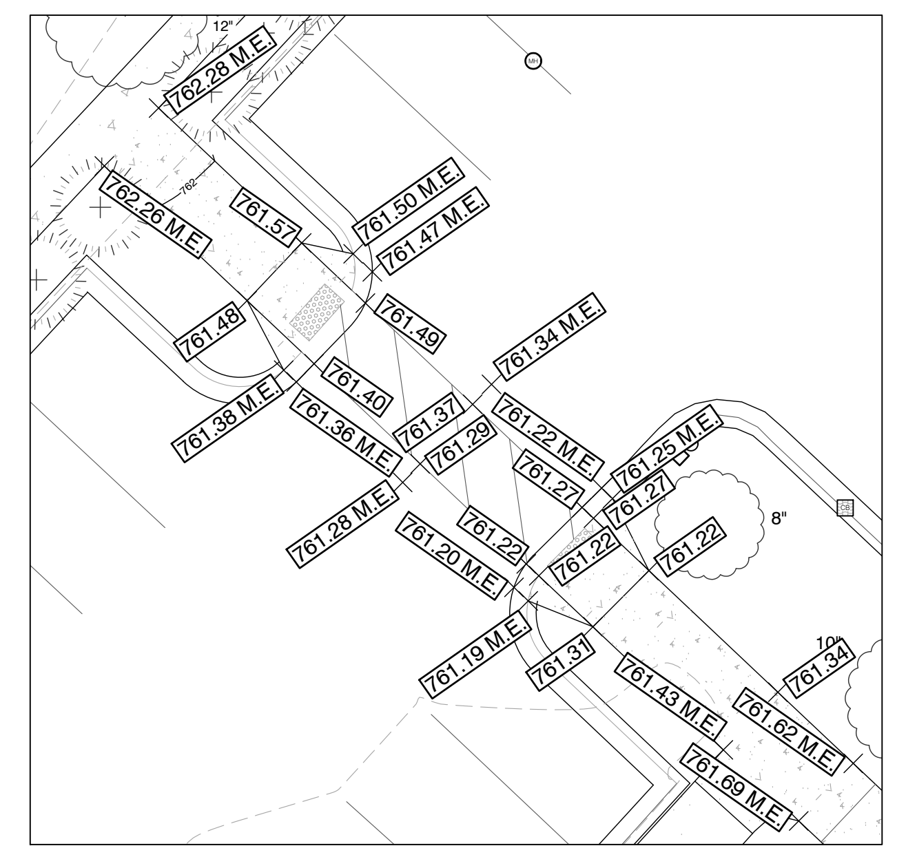
ADA CROSSWALK GRADING DETAIL C3.0 1 INCH = 10 FEET
