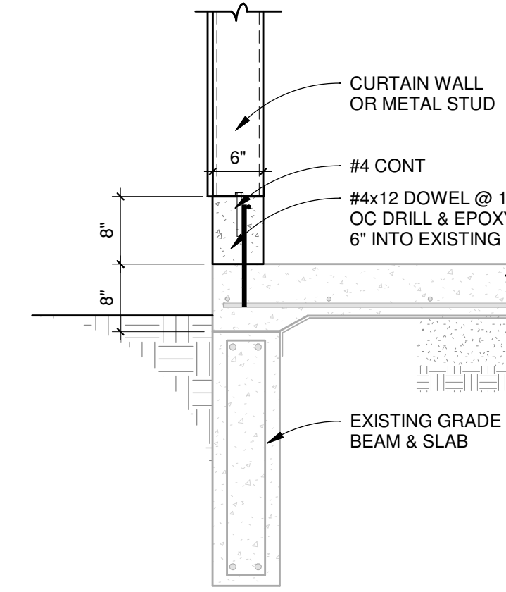
2 CURB AT EXISTING CONSTRUCTION SCALE: 3/4" = 1'-0"
