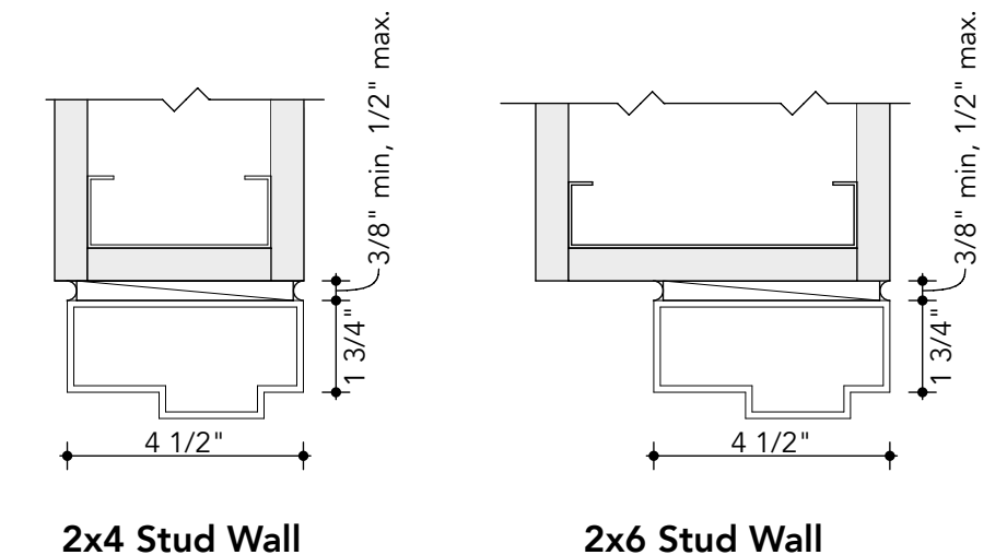
3 Typical Aluminum Frame Head Interior A403 SCALE: 3" = 1'-0"
