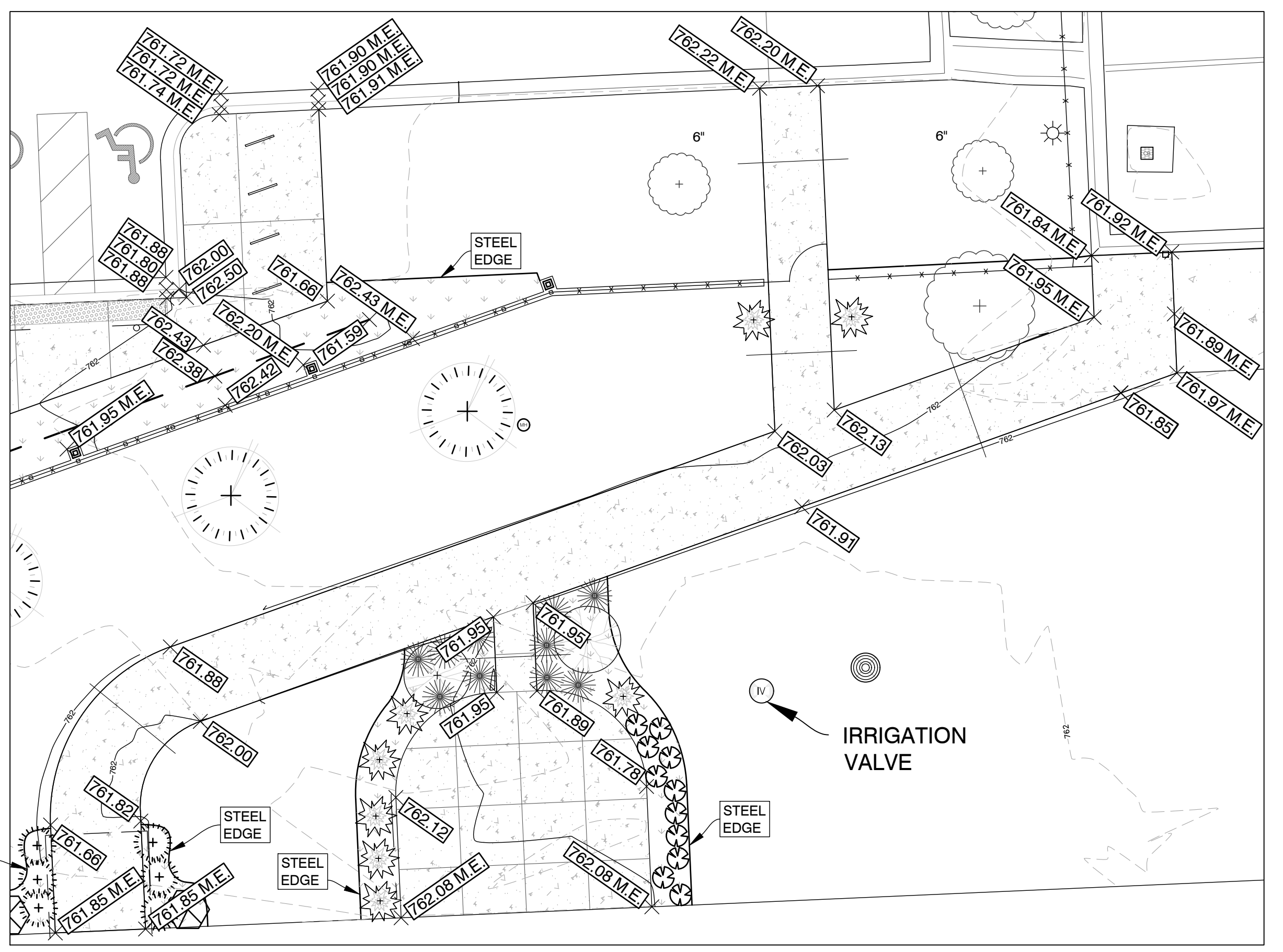
PATIO GRADING DETAIL C3.0 1 INCH = 10 FEET
