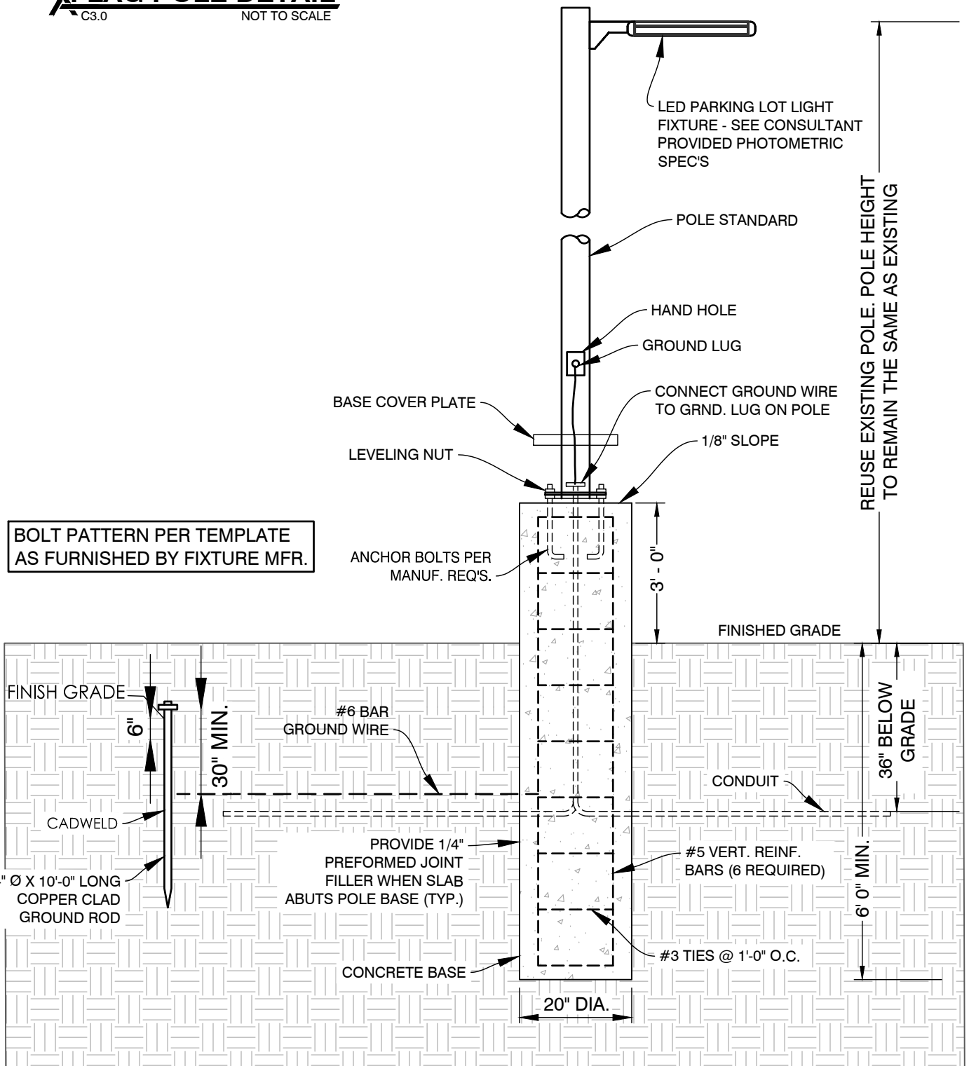
LIGHT POST DETAIL C3.0 - 09/0110 NOT TO SCALE
