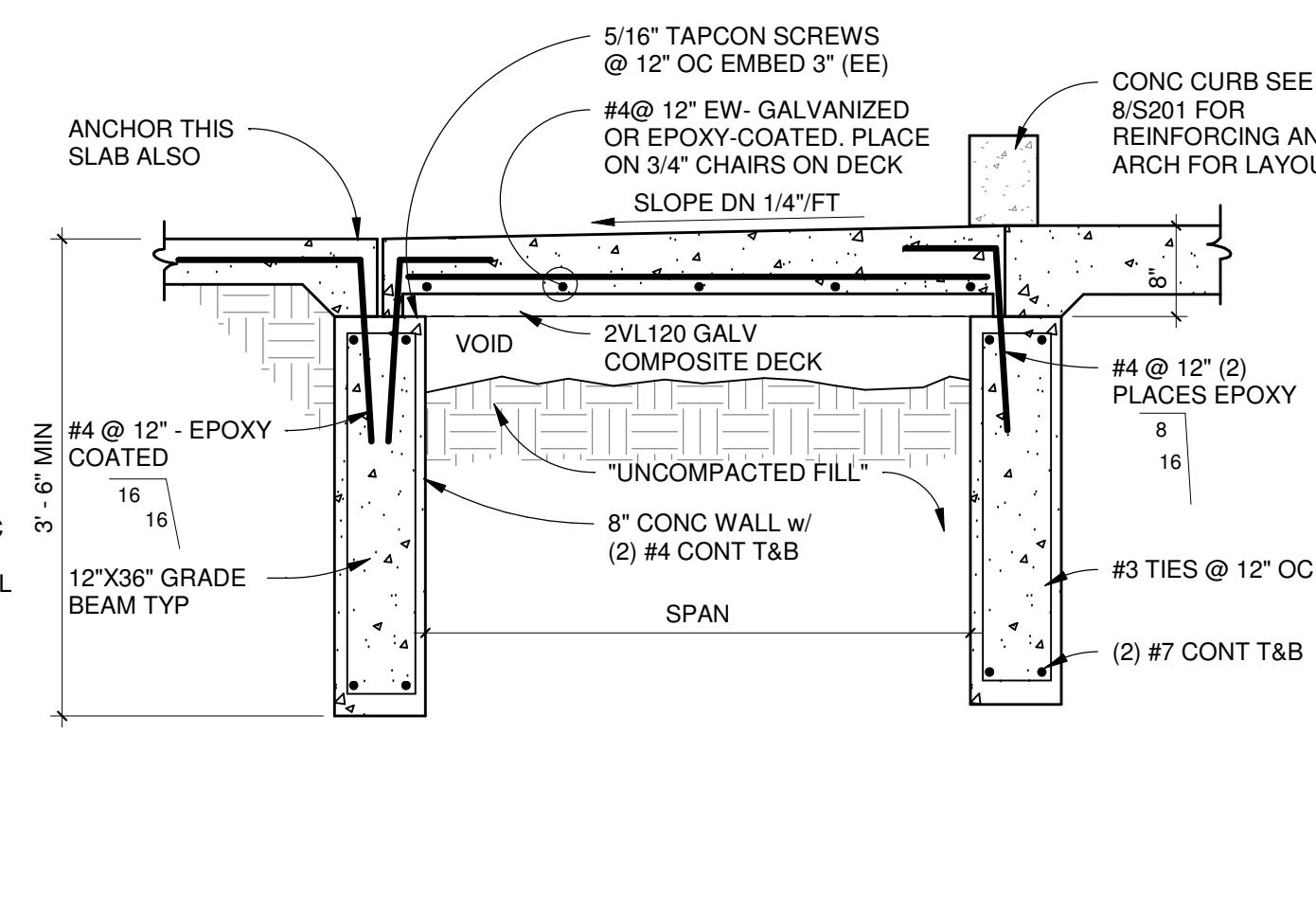
10 S201 THRESHOLD DETAIL SCALE: 3/4" = 1'-0"
