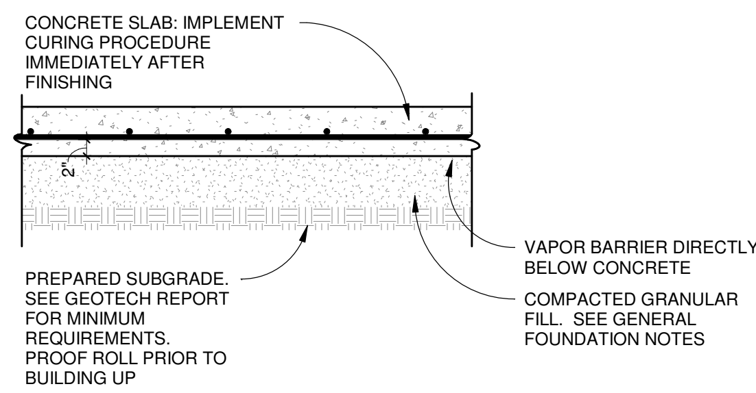
1 S201 TYPICAL SLAB ON GRADE CONSTRUCTION SCALE: 3/4" = 1'-0"
