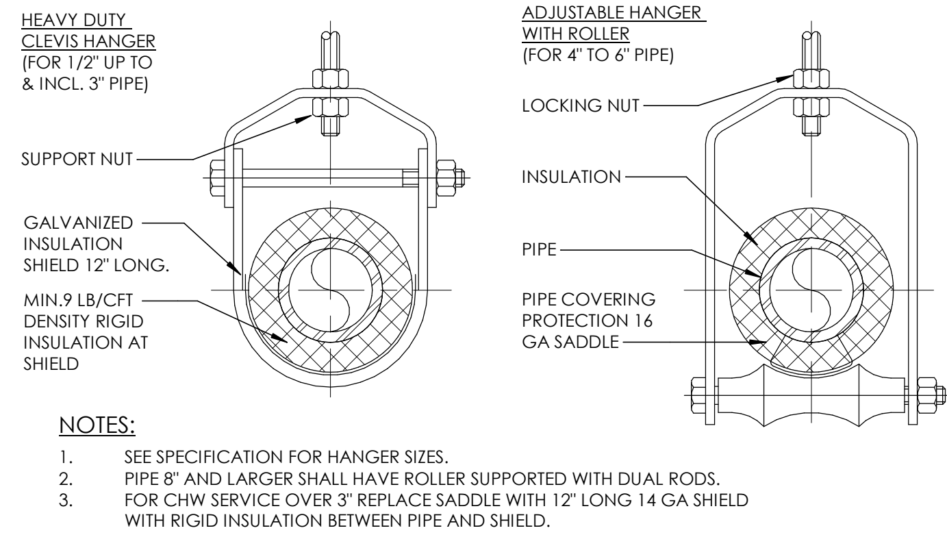
2 PIPE HANGER SUPPORT DETAIL M501 NOT TO SCALE
