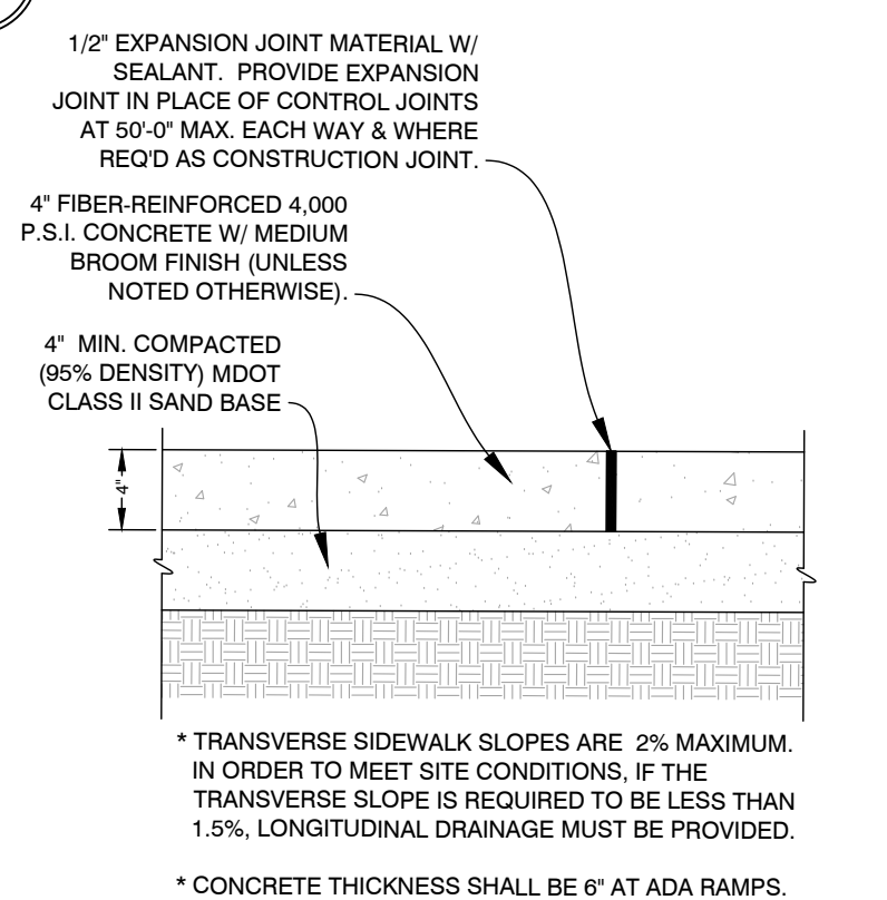
CONCRETE WALK DETAIL C3.0 NOT TO SCALE
