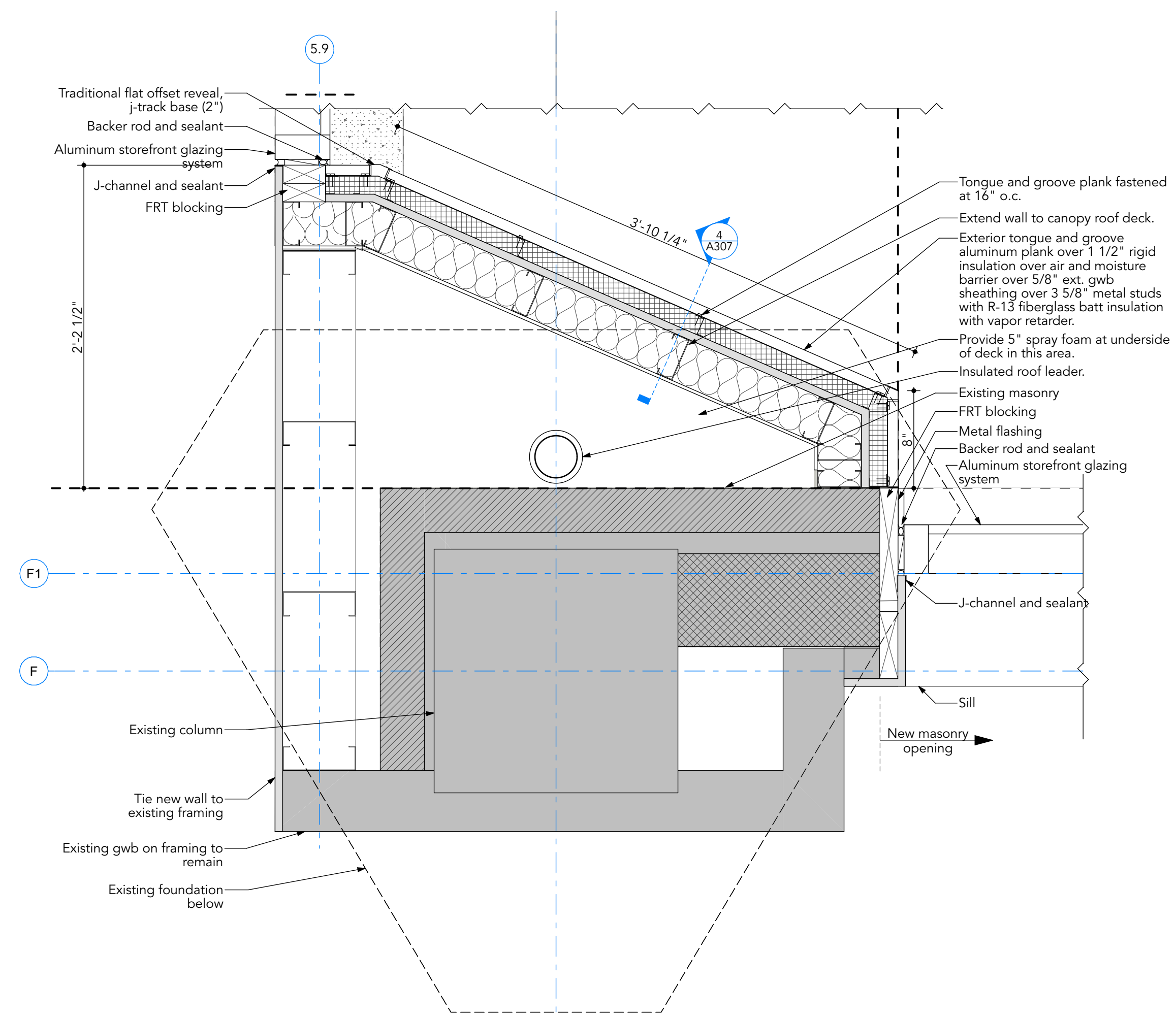
11 Entry to Existing Wall Plan Detail A307 SCALE: 1 1/2" = 1'-0"
