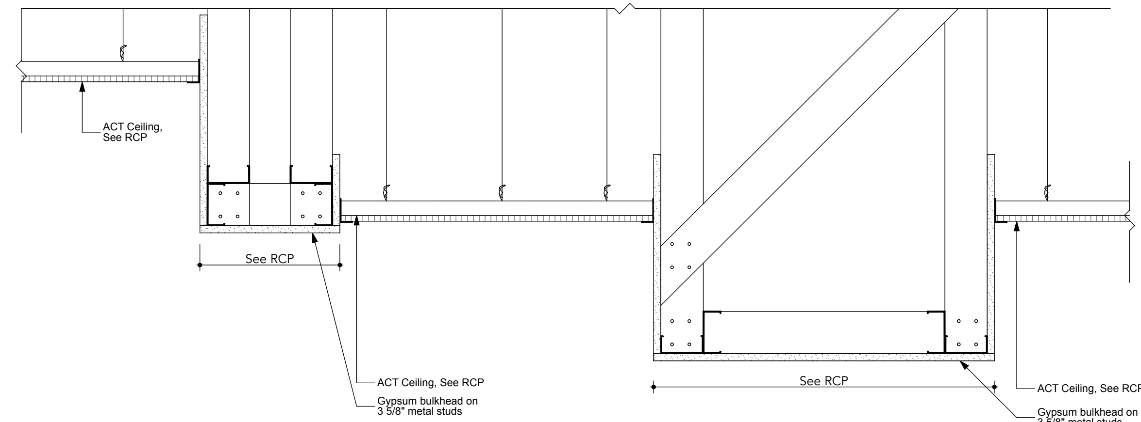
6 Town Square Ceiling Detail at Entry A113 SCALE: 1 1/2" = 1'-0"
