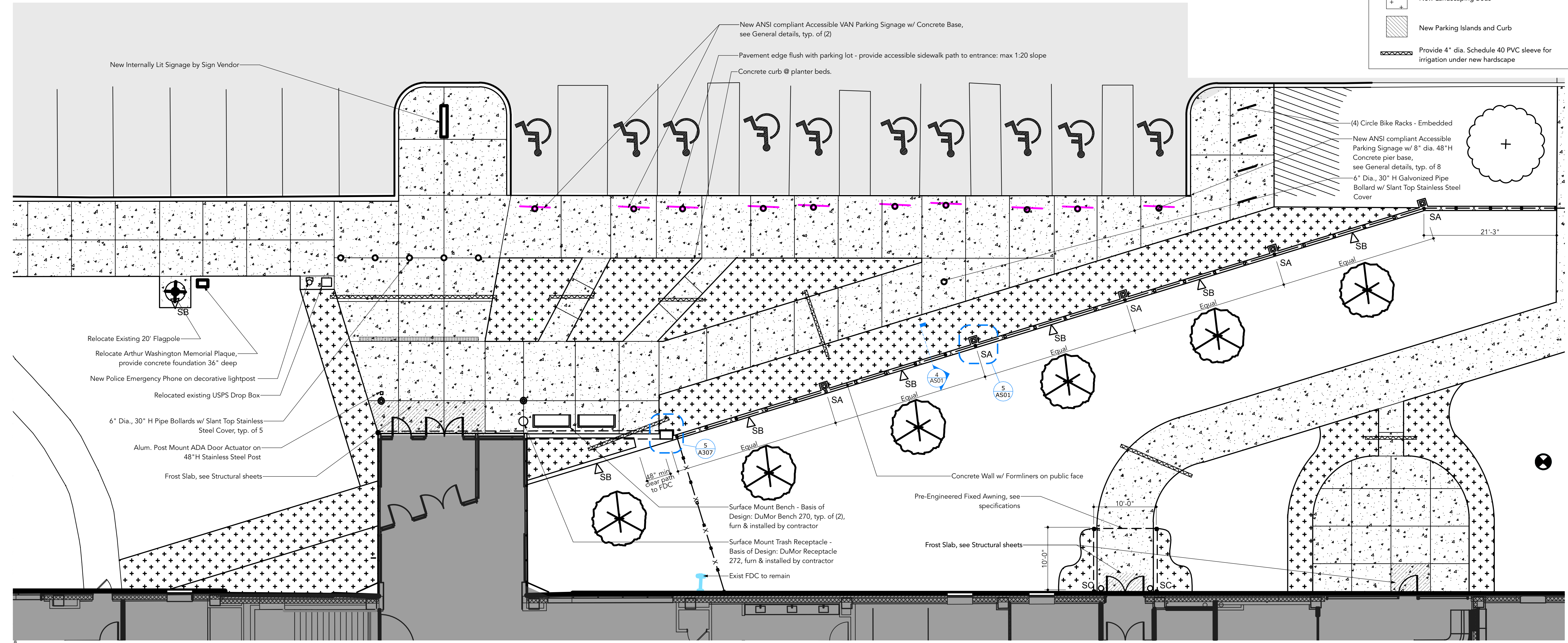
1 Enlarged Site Plan AS01 SCALE: 1/8" = 1'-0"
