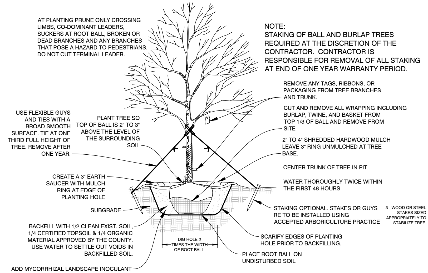
TYPICAL DECIDUOUS TREE PLANTING DETAIL C3.0 NOT TO SCALE
