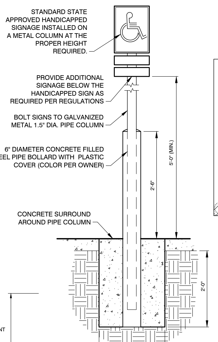
HANDICAP PARKING SIGN DETAIL C3.0 NOT TO SCALE
