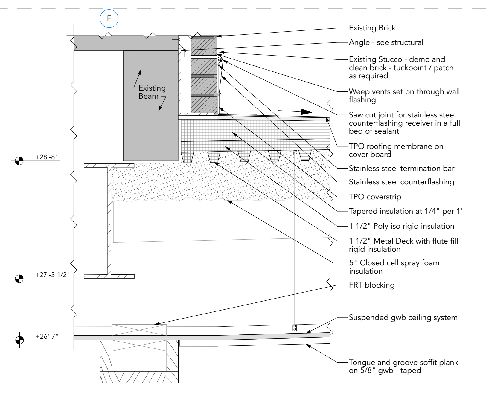
8 Entry Canopy Roof @ Existing Wall Detail A306 SCALE: 1 1/2" = 1'-0"
