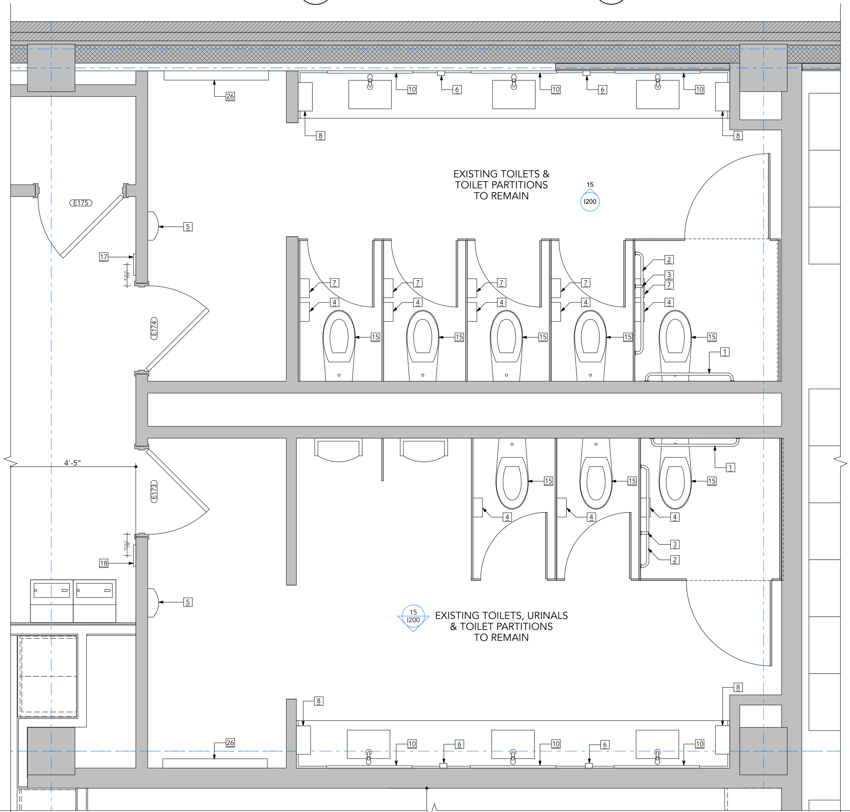
See Floor Plans for Fixture Qty & Layout of other multi-user toilet rooms 1 Typical Toilet Room Renovation Plans A106 SCALE: 1/2" = 1'-0"
