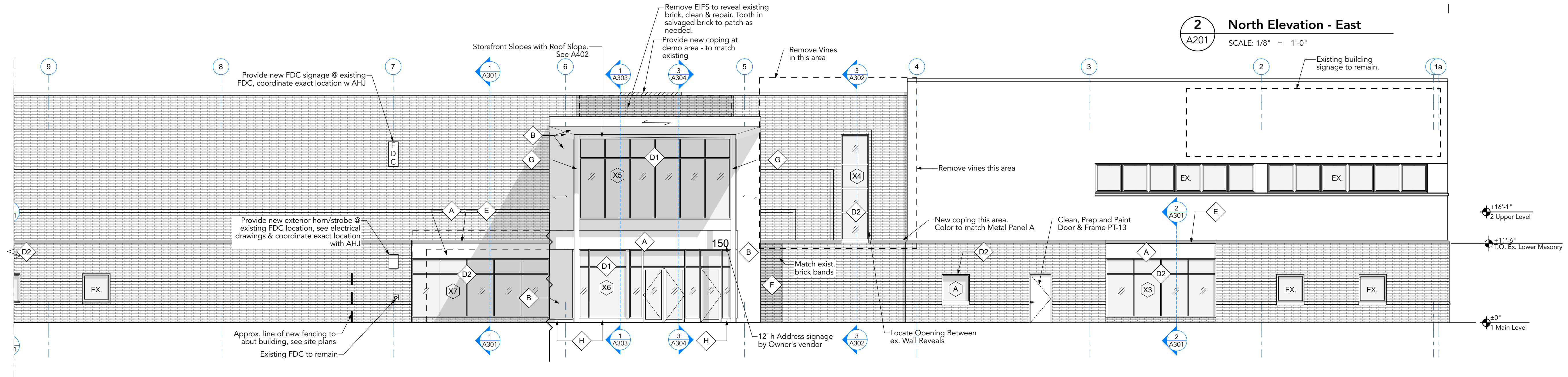
1 North Elevation - West A201 SCALE: 1/8" = 1'-0"
