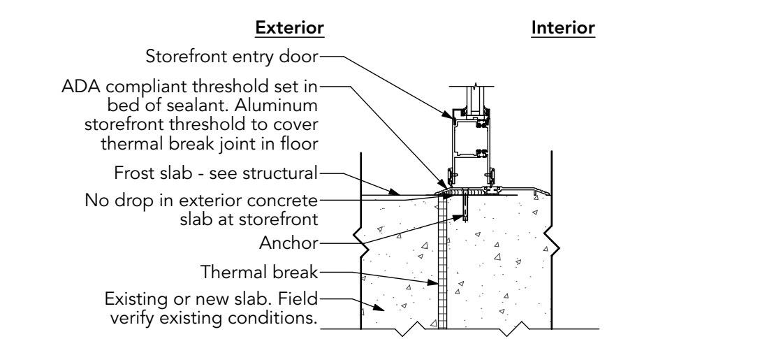
7 Aluminum SF Door Threshold A301 SCALE: 1 1/2" = 1'-0"
