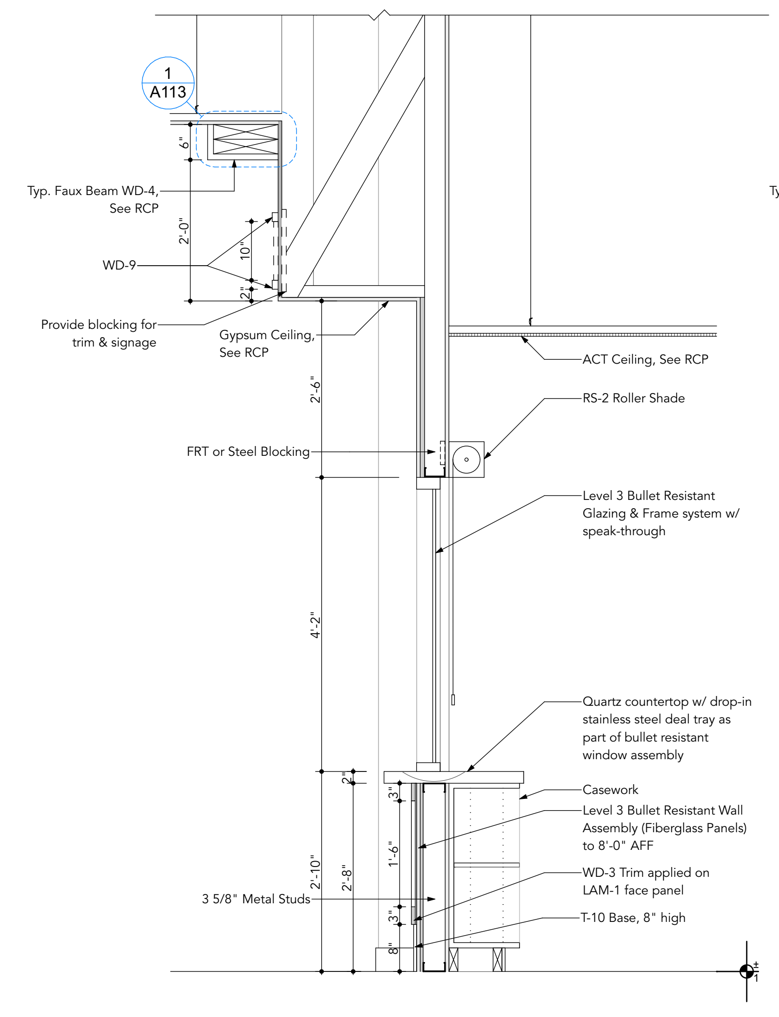
3 Service Desk Section - Clerk A308 SCALE: 3/4" = 1'-0"
