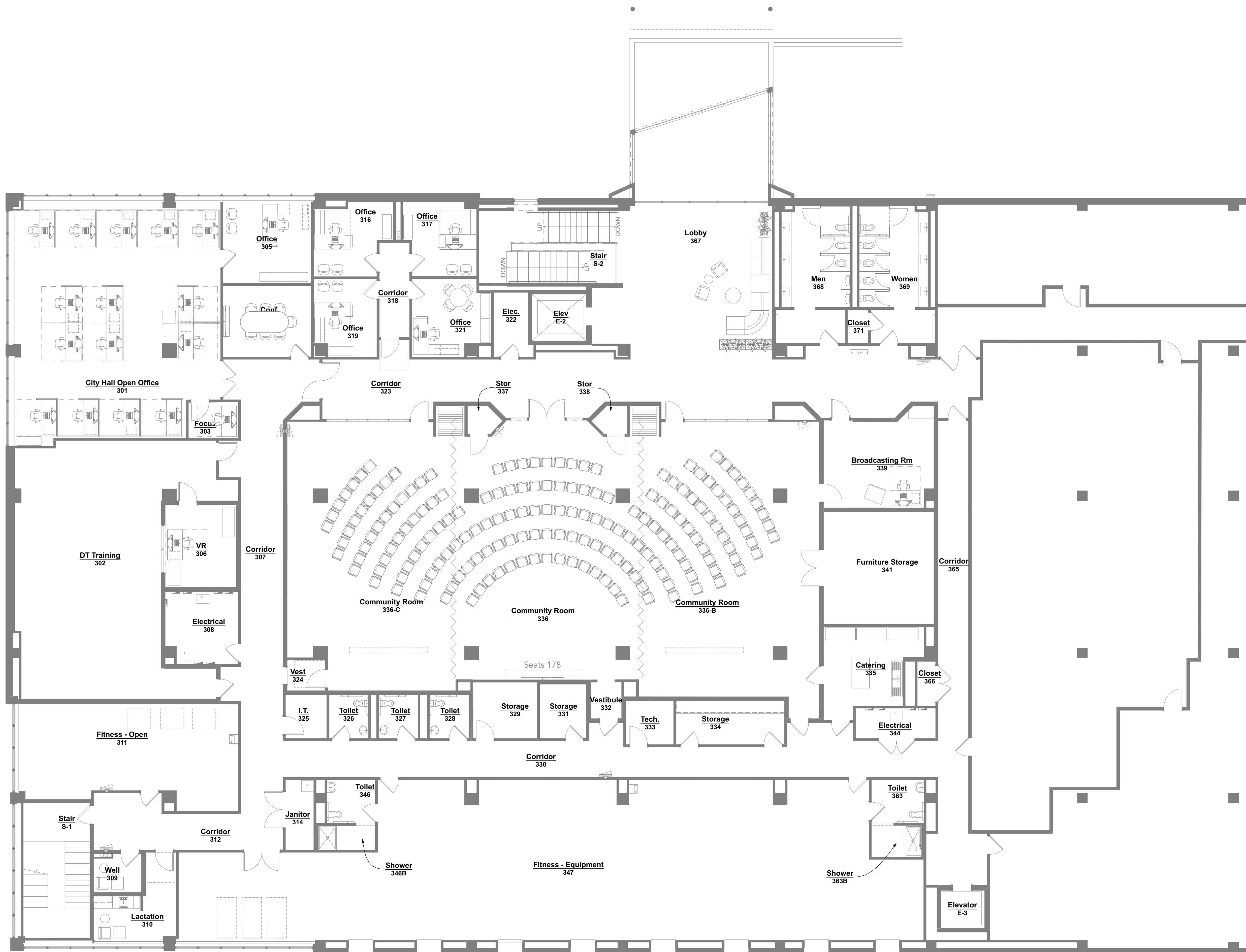
1 Furniture Upper Level Plan 1106 SCALE: 1/8" = 1'-0"
