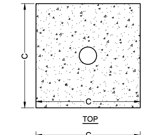
INLET PROTECTION - SILT SACK C3.0 NOT TO SCALE
