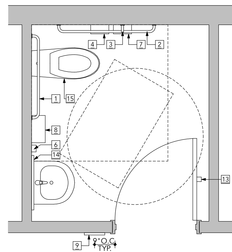
3 Toilet Room #326, #327, #328, Typ. A106 SCALE: 1/2" = 1'-0"
