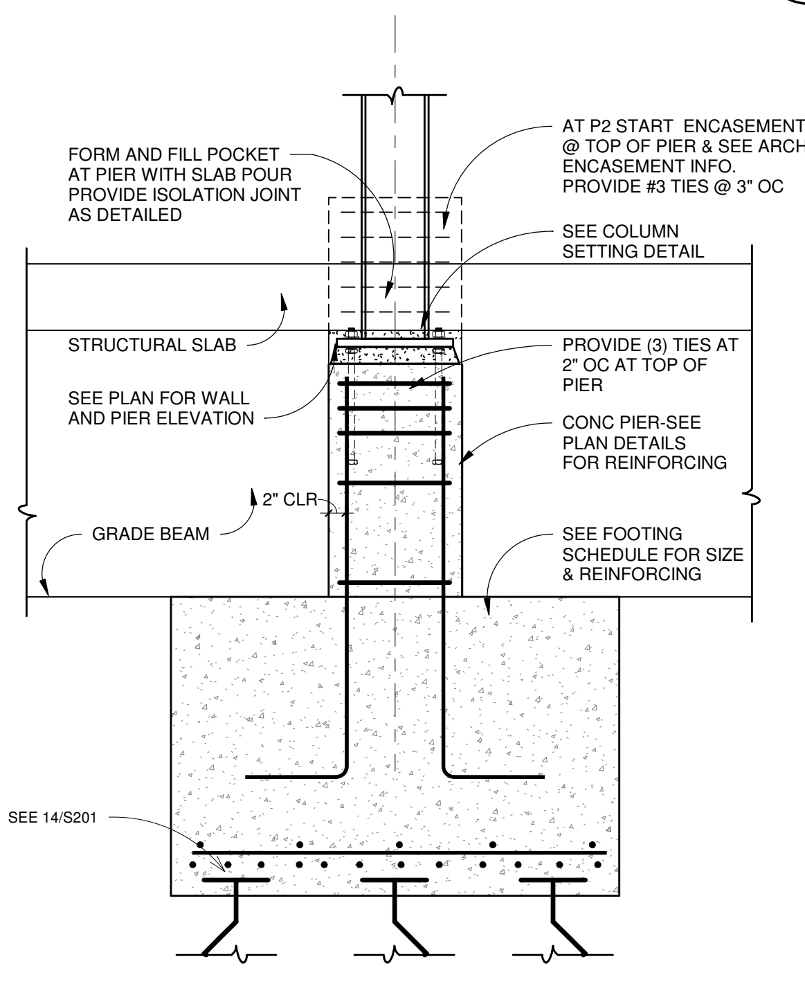
7 S201 TYPICAL EXTERIOR COLUMN PIER SCALE: 3/4" = 1'-0"
