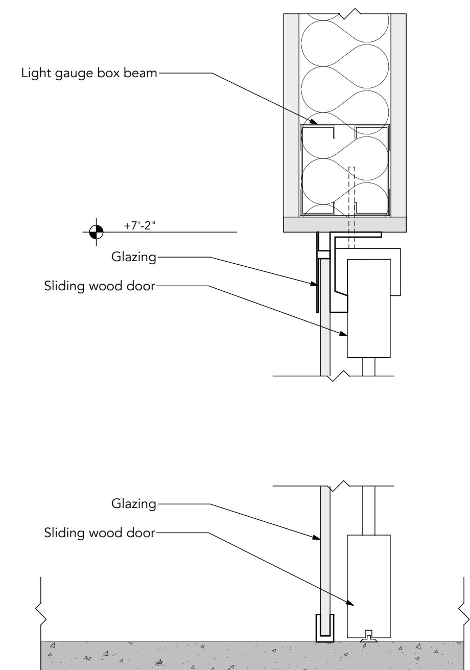
6 Ceiling Mount Sliding Door Detail A403 SCALE: 3" = 1'-0"
