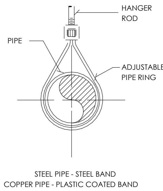
4 P501 UNINSULATED PIPE HANGER DETAIL NOT TO SCALE
