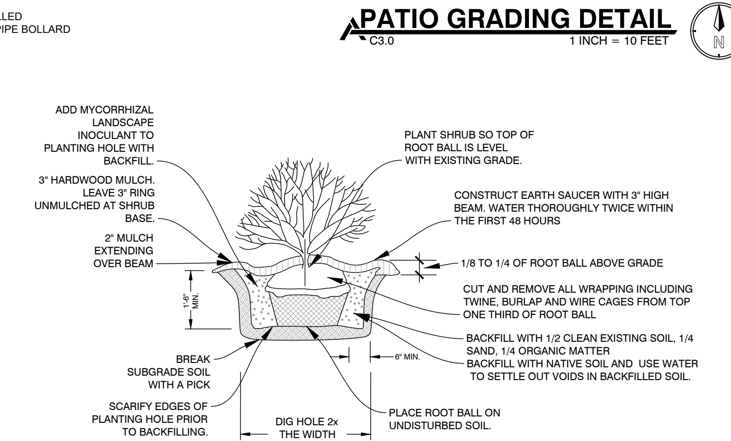
TYPICAL SHRUB PLANTING DETAIL C3.0 NOT TO SCALE
