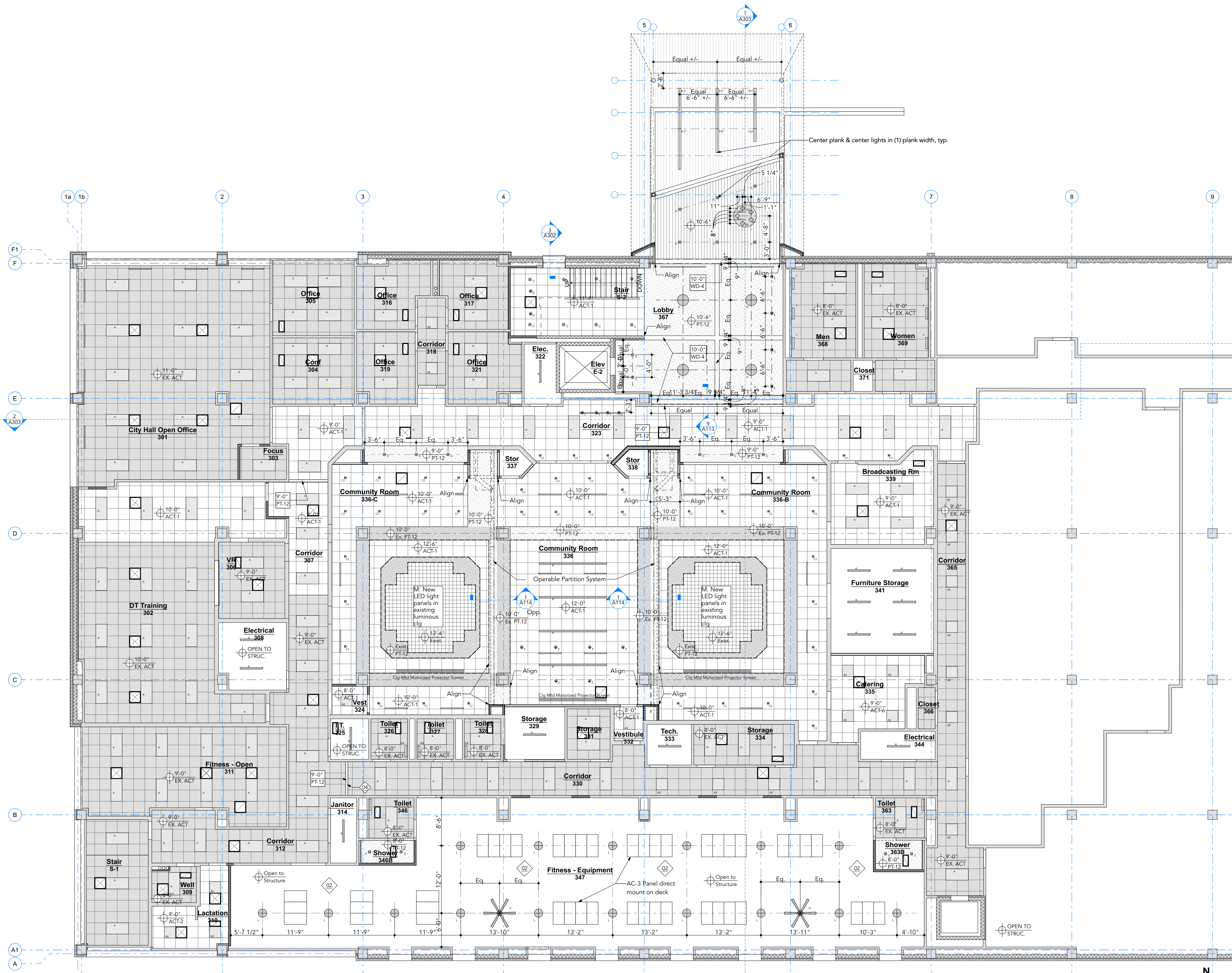
1 Reflected Ceiling Upper Level Plan A109 SCALE: 1/8" = 1'-0"
