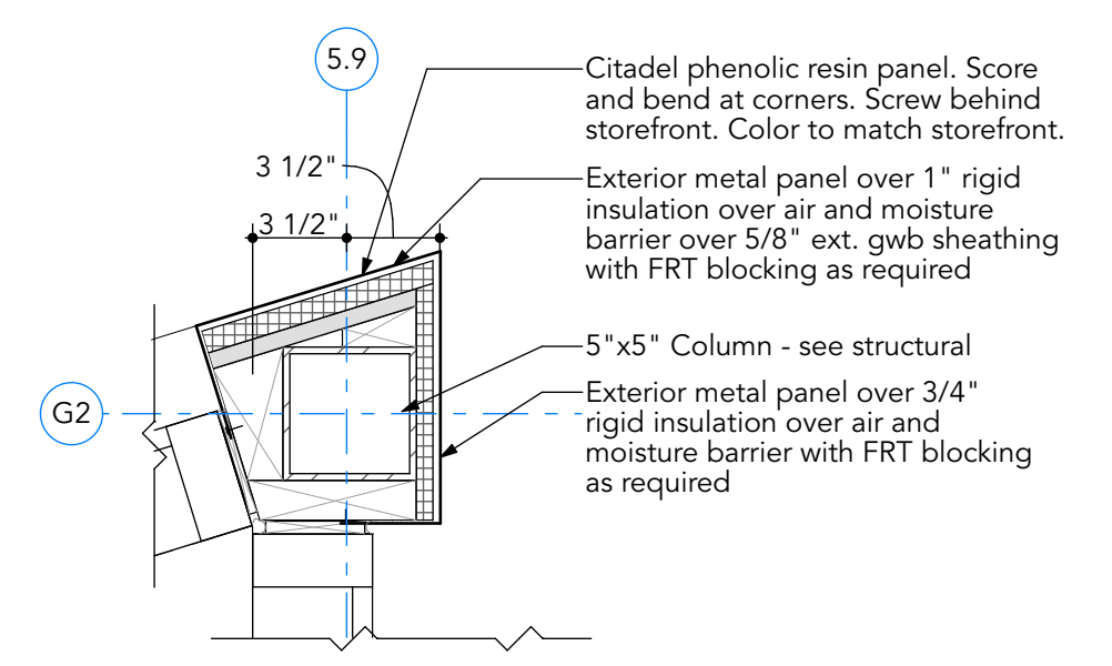
7 Entry Canopy Wall 2nd Fl @ Column Plan A307 SCALE: 1 1/2" = 1'-0"
