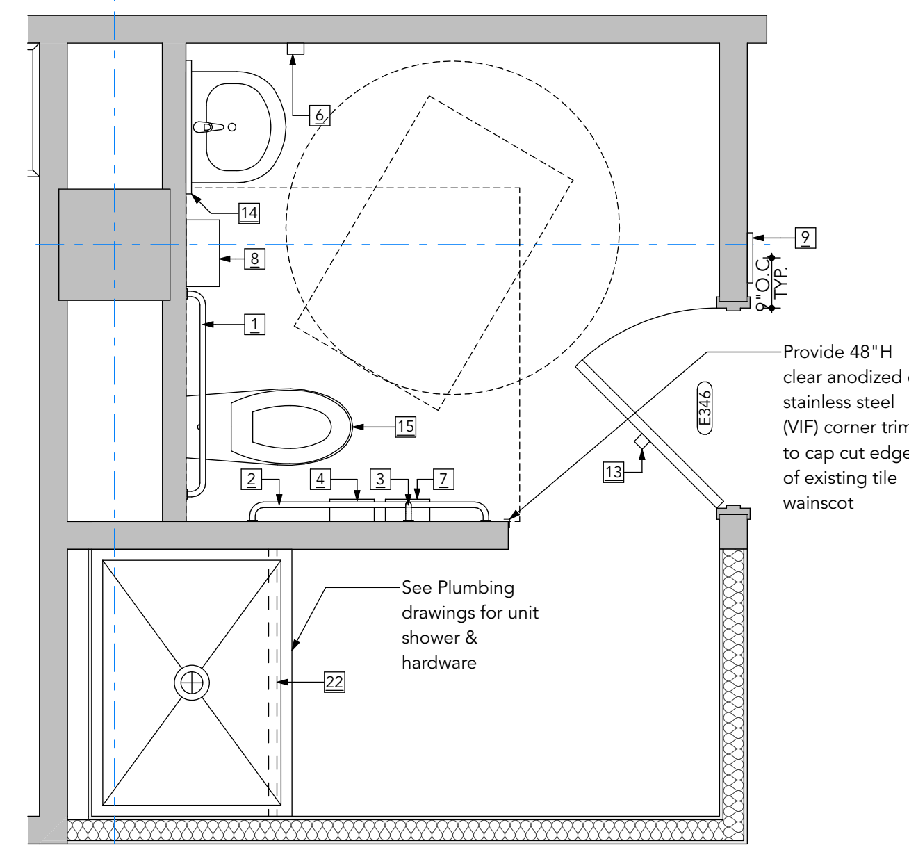
5 Shower Plan #346 A106 SCALE: 1/2" = 1'-0"
