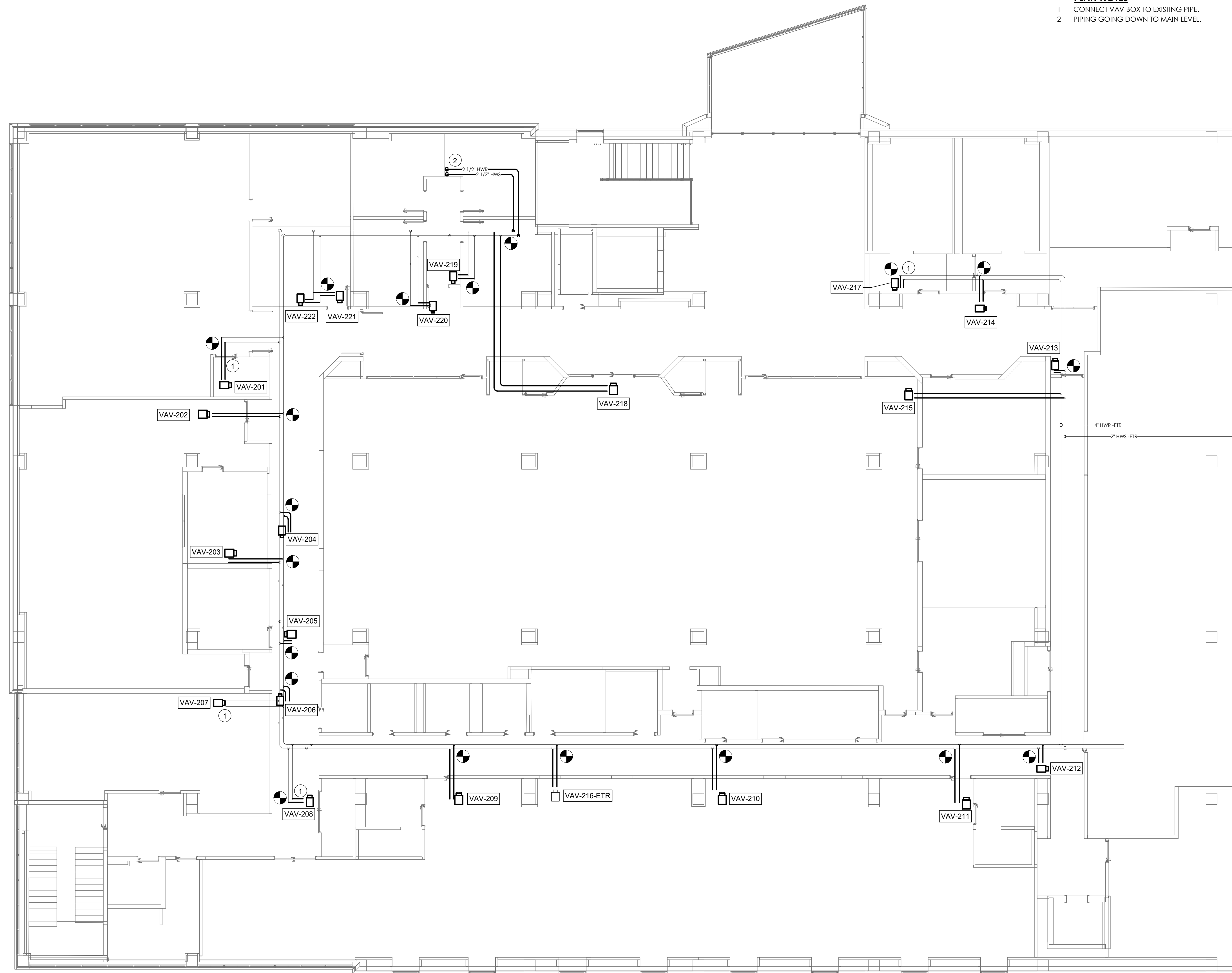
1 UPPER LEVEL CPED HVAC PIPING PLAN M202 1/8" = 1'-0"
