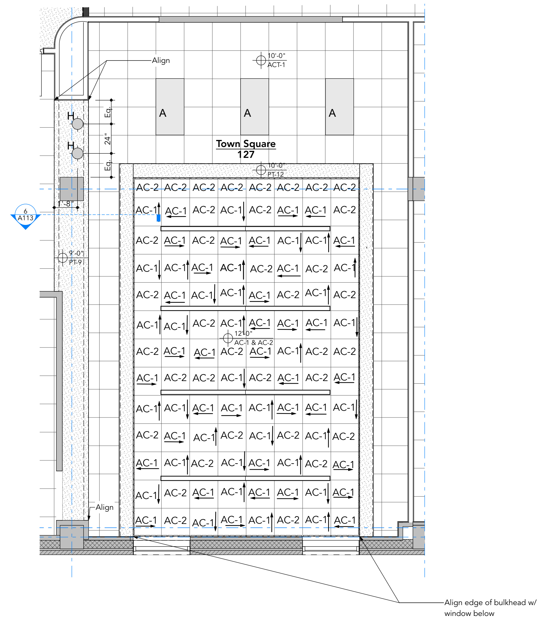
1 A112 Town Square Enlarged Ceiling Plan SCALE: 1/4" = 1'-0"
