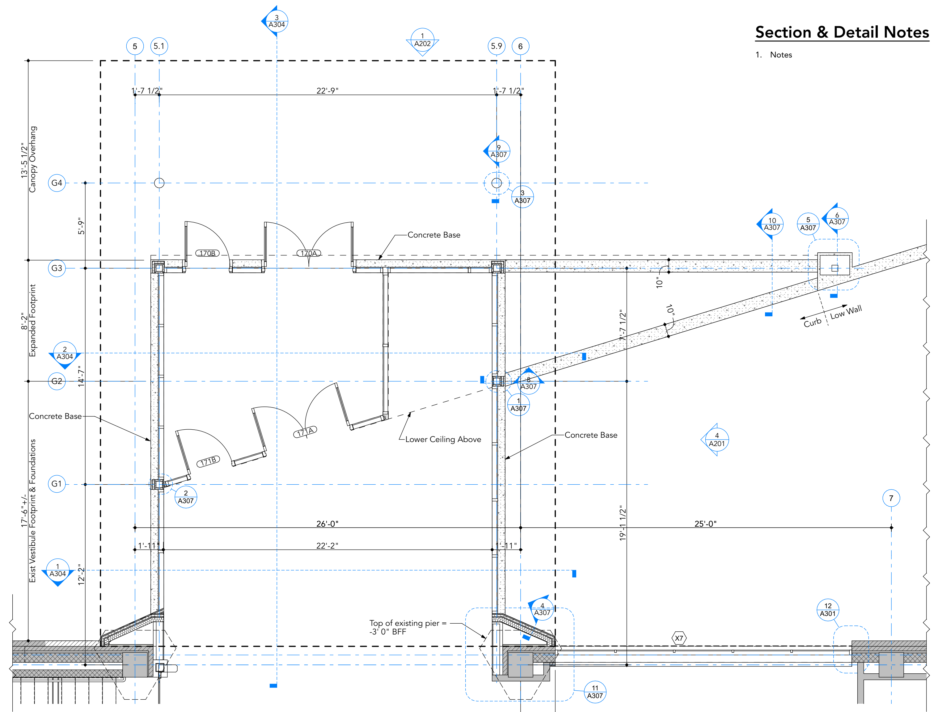
6 Entry and Canopy Plan
