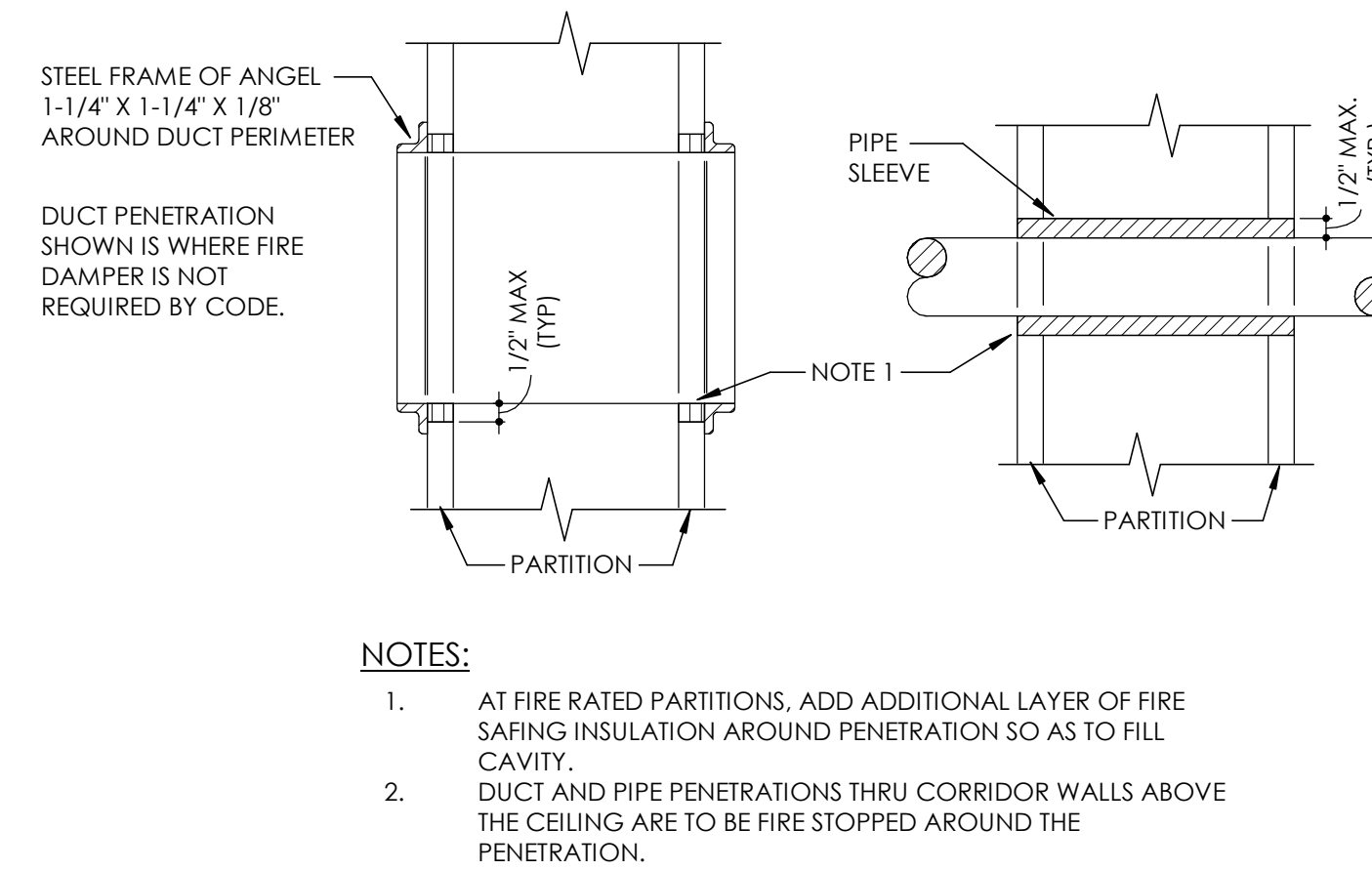
4 DUCT AND PIPE PENETRATIONS M501 NOT TO SCALE
