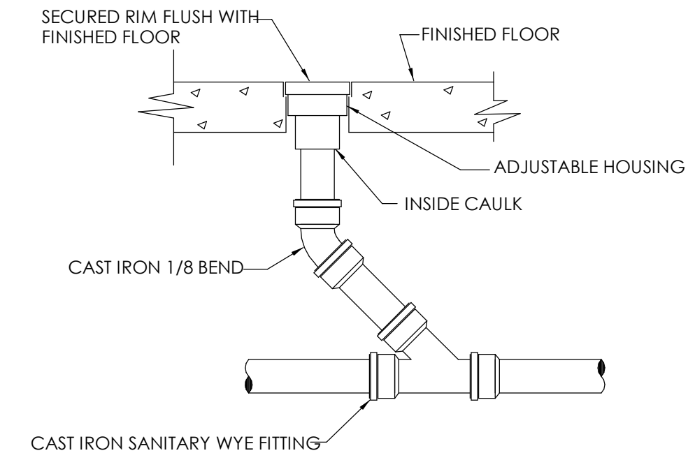
1 P501 FLOOR CLEANOUT DETAIL NOT TO SCALE
