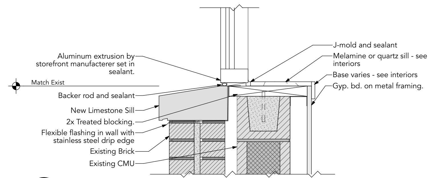
8 FG Fixed Window Sill at Double Wythe Brick A301 SCALE: 1 1/2" = 1'-0"
