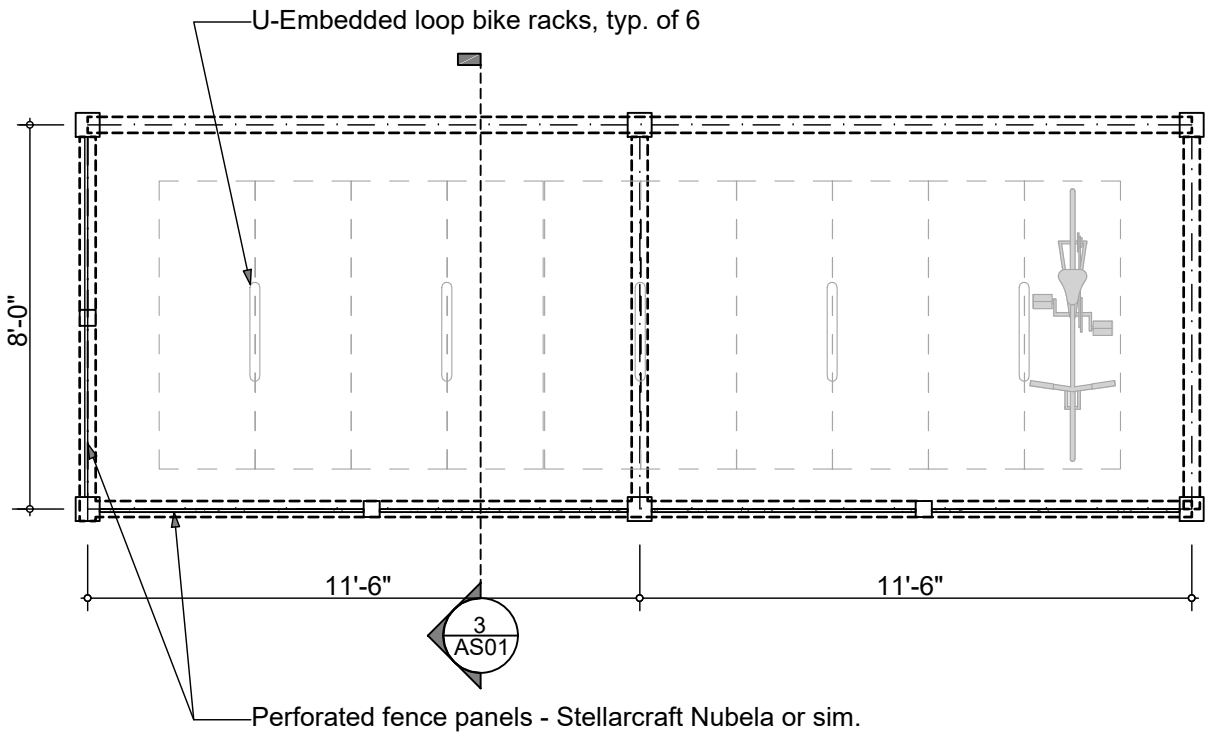
BIKE SHELTER ENLARGED PLAN CS.1 NOT TO SCALE
