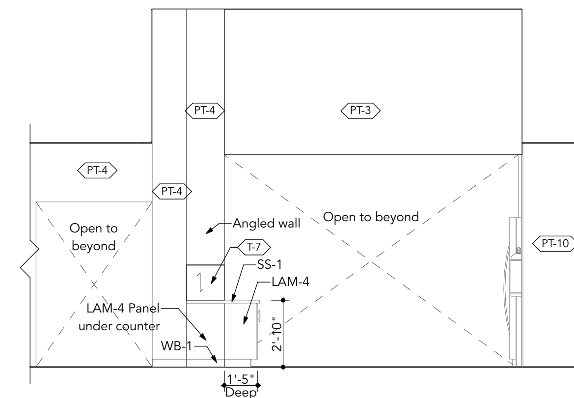
6 Corridor Looking South 1203 SCALE: 1/4" = 1'-0"
