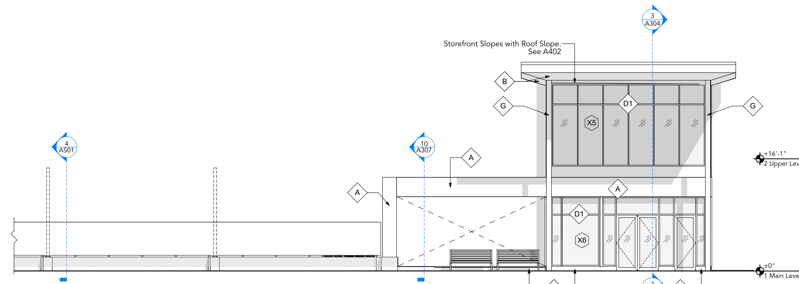
1 Entry - North Elevation A202 SCALE: 1/8" = 1'-0"
