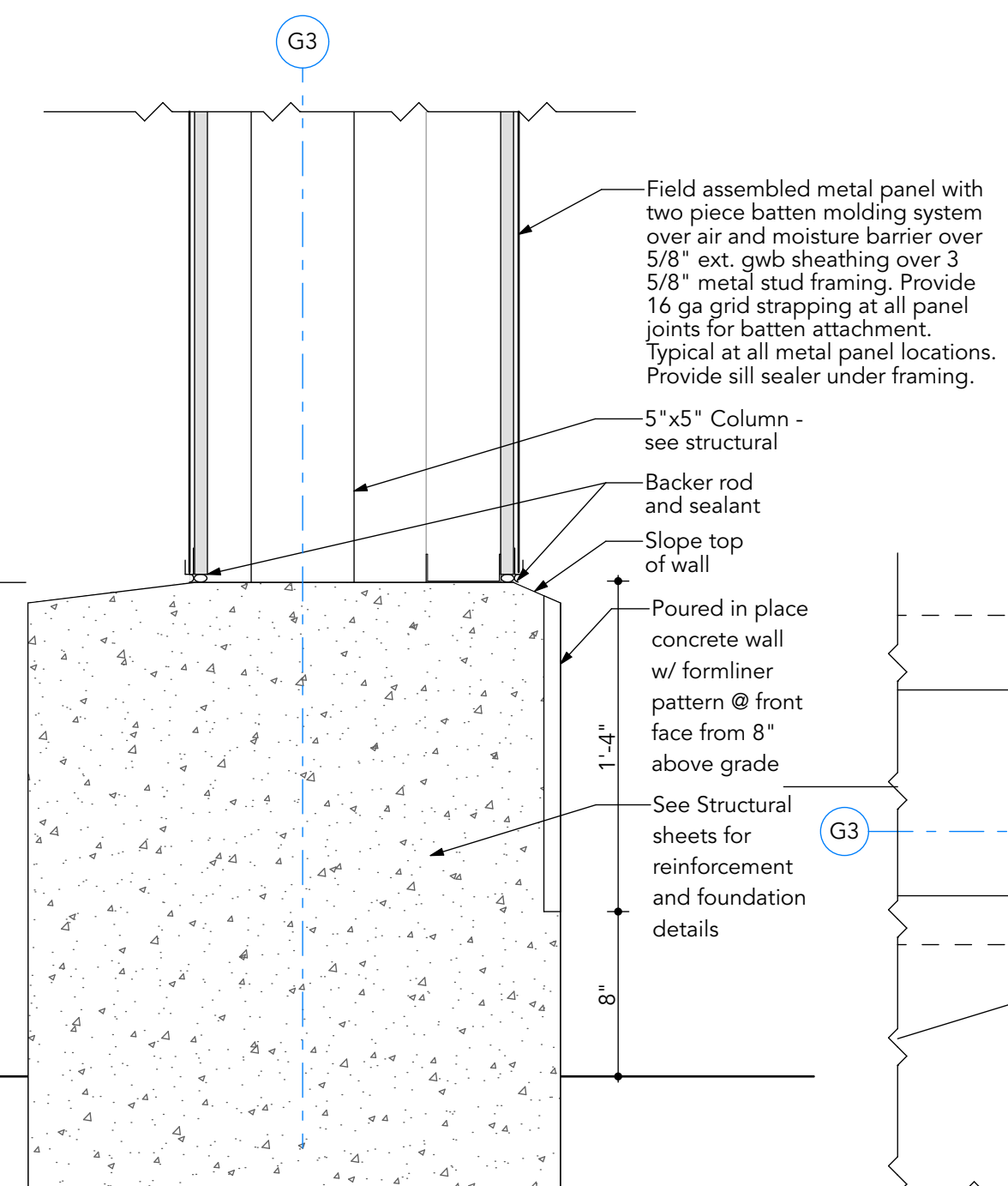
6 Entry Canopy Arm @ Column Section Detail A307 SCALE: 1 1/2" = 1'-0"
