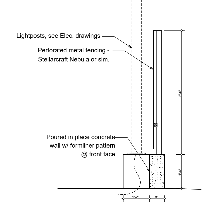
SITE WALL SECTION DETAIL CS.1 NOT TO SCALE
