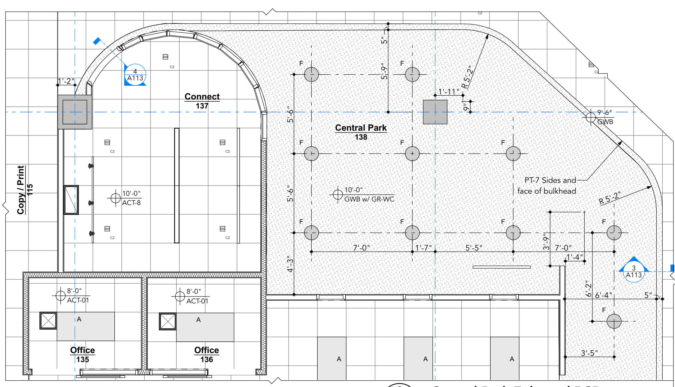
2 Central Park Enlarged RCP A111 SCALE: 1/4" = 1'-0"
