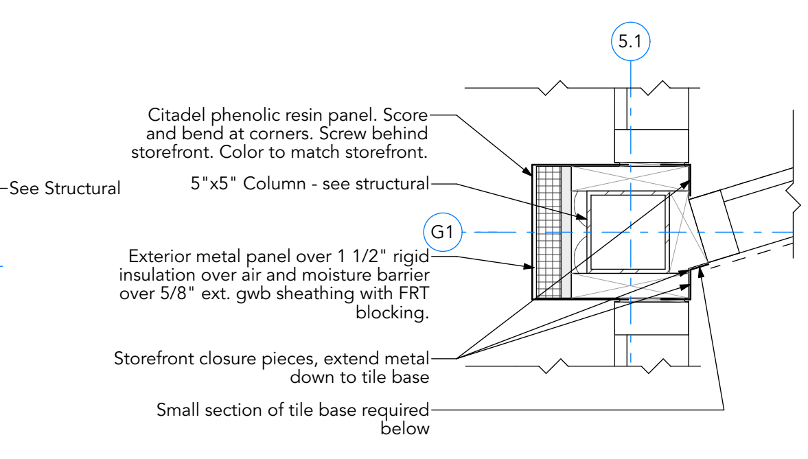
2 Entry Canopy Wall @ Column Plan A307 SCALE: 1 1/2" = 1'-0"
