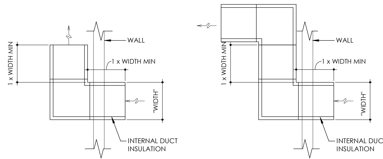
17 DUCT- \"L\" & \"Z\" SHAPED TRANSFER M501 NOT TO SCALE
