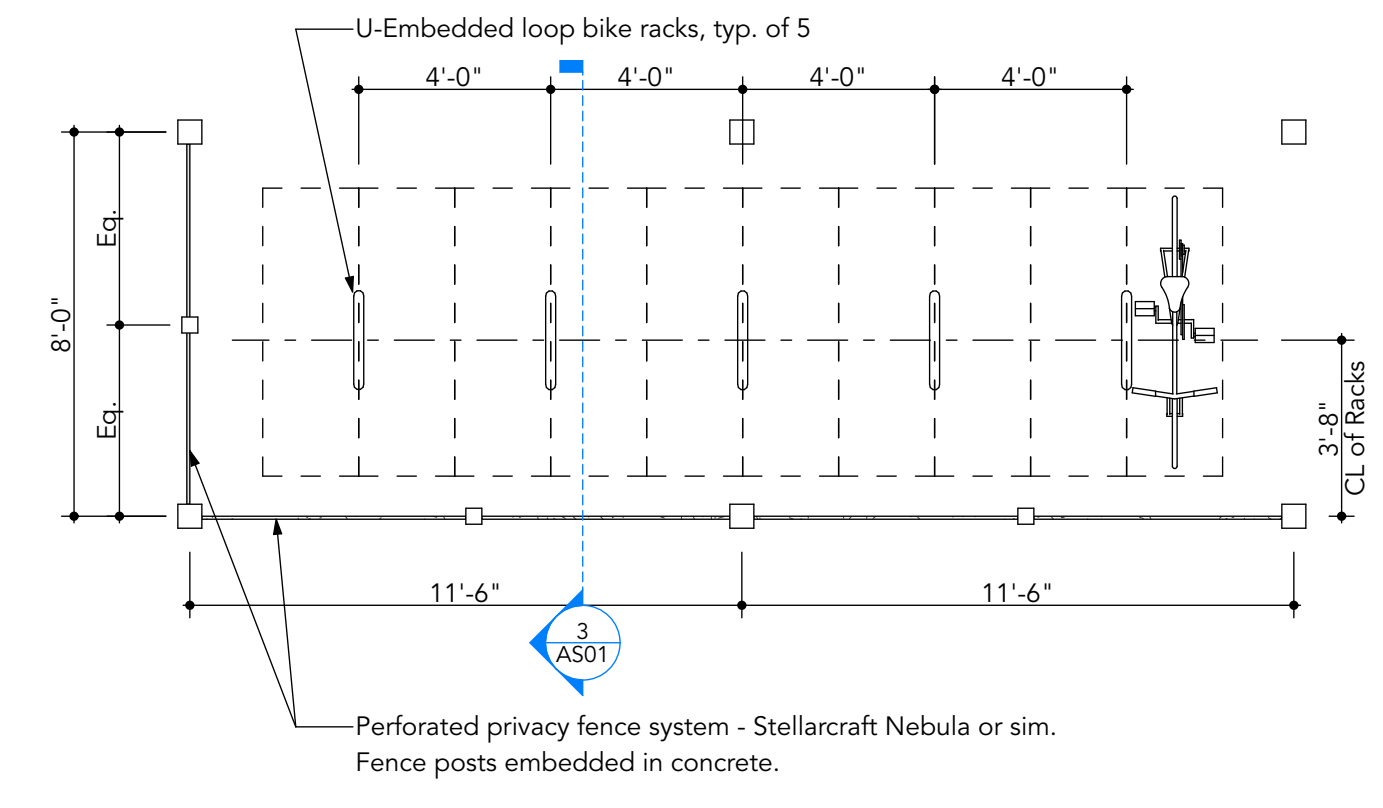
2 Bike Shelter Enlarged Plan AS01 SCALE: 1/4" = 1'-0"
