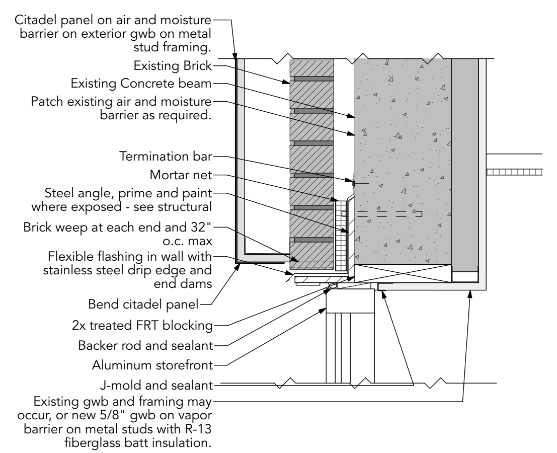
9 Aluminum SF Head at Concrete A301 SCALE: 1 1/2" = 1'-0"
