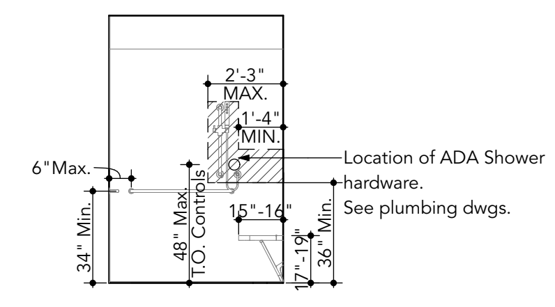
13 ADA Shower 363 East I200 SCALE: 1/4" = 1'-0"
