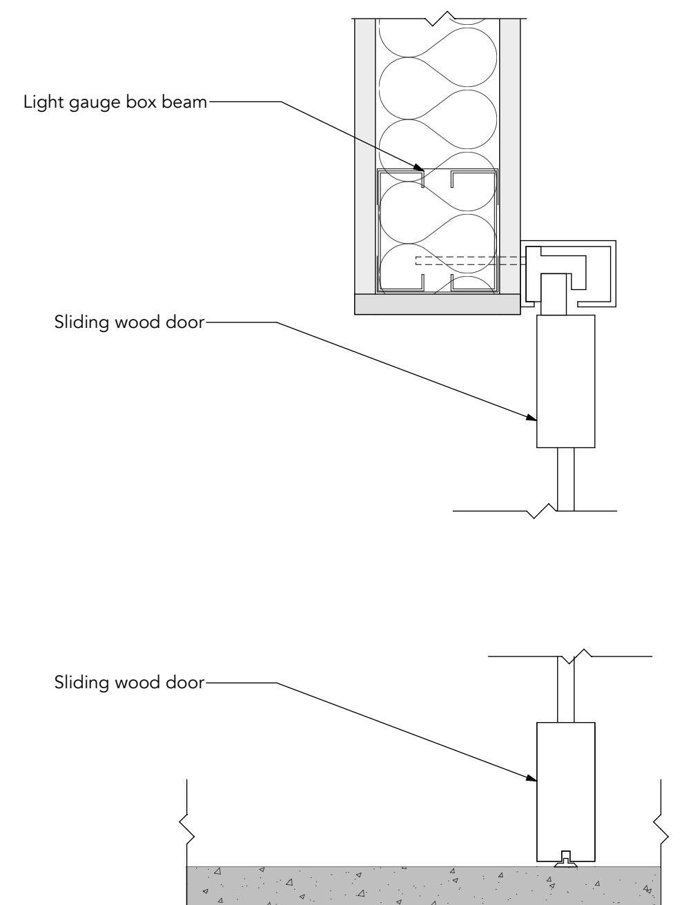
5 Wall Mount Sliding Door Detail A403 SCALE: 3" = 1'-0"
