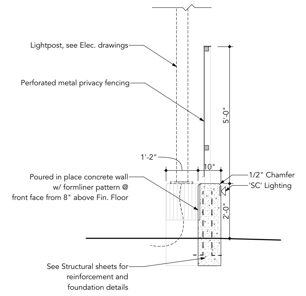
4 Site Wall Section AS01 SCALE: 1/2" = 1'-0"
