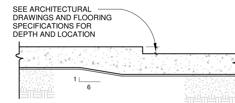
2 S201 TYPICAL RECESSED SLAB DETAIL SCALE: 3/4" = 1'-0"
