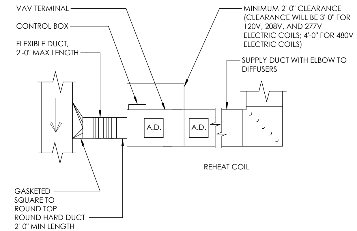
19 DUCT VARIABLE AIR VOLUME TERMINAL WITH REHEAT COIL M501 NOT TO SCALE
