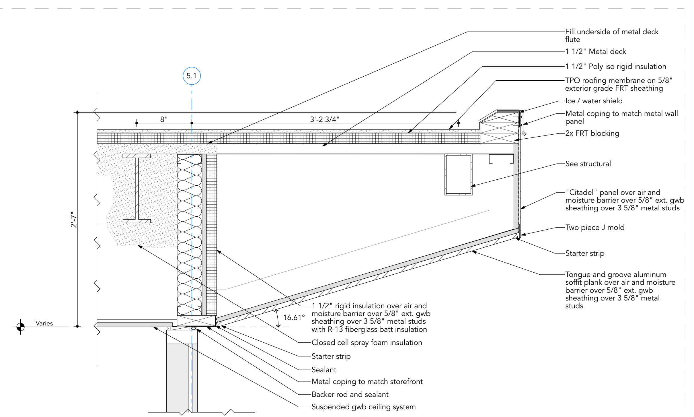
6 Entry Canopy Roof @ Edge Detail A306 SCALE: 1 1/2" = 1'-0"
