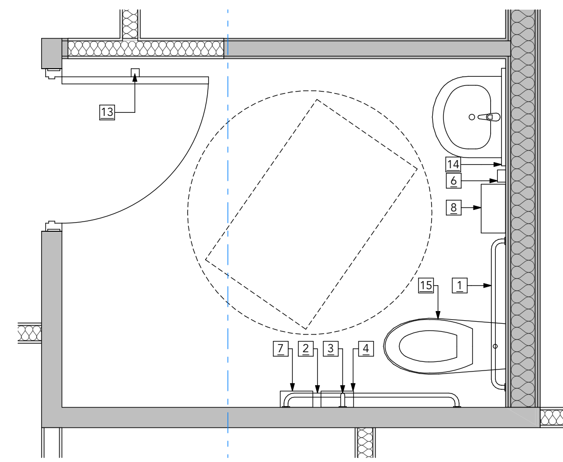
6 Toilet Room #102 A106 SCALE: 1/2" = 1'-0"
