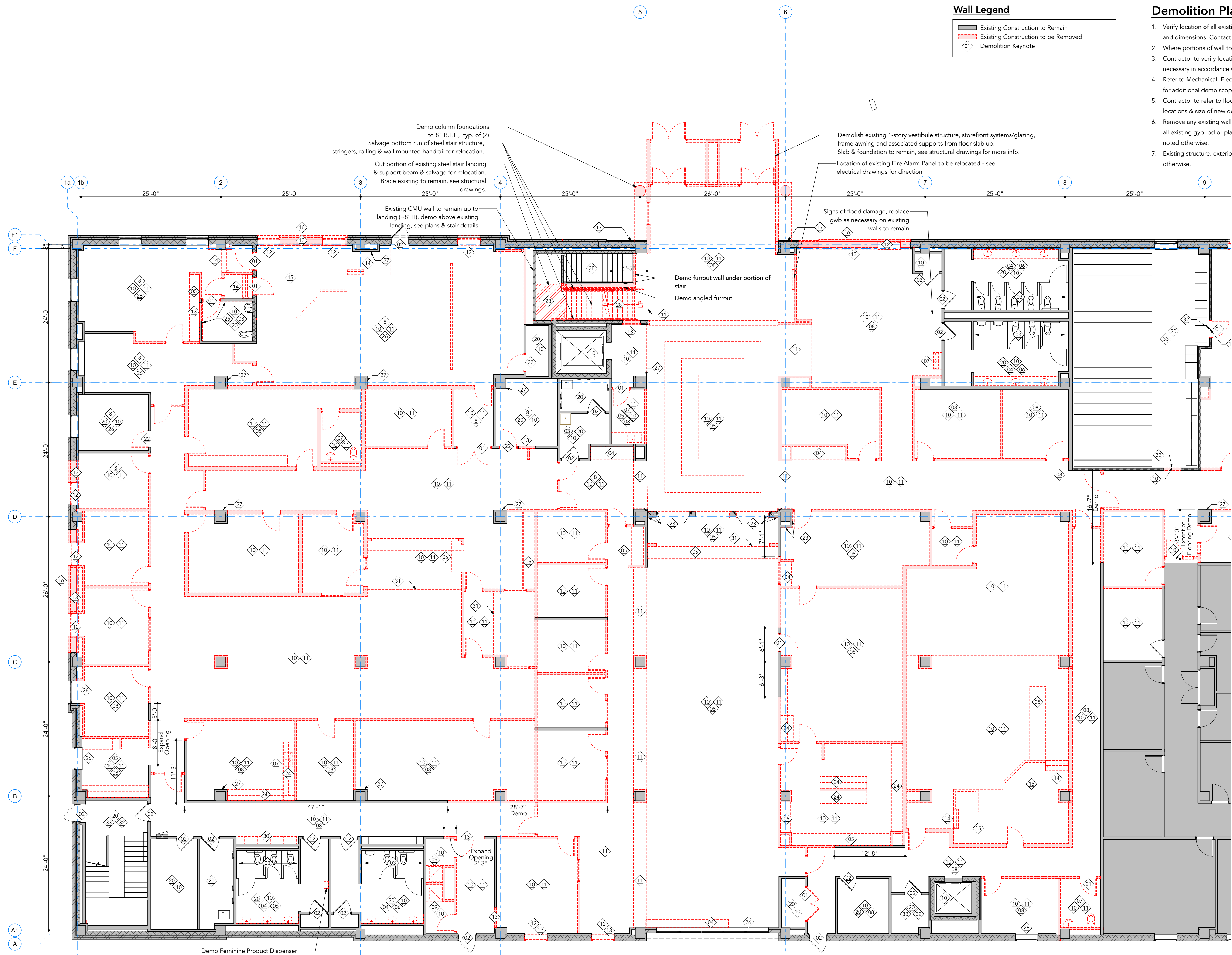
1 A001 Demolition Main Level Plan SCALE: 1/8" = 1'-0"
