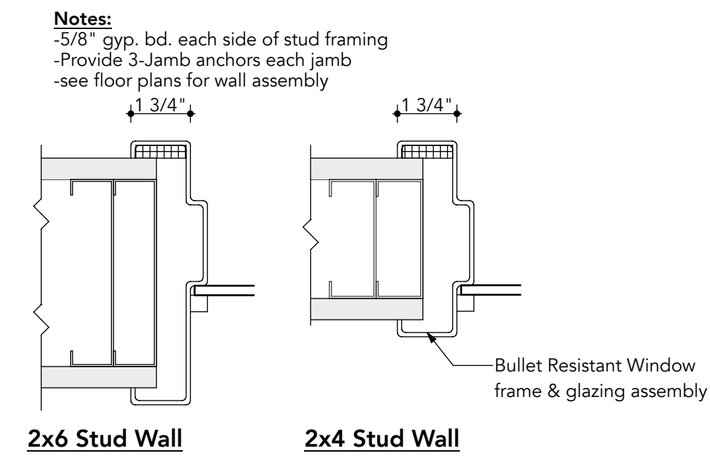
12 Typical HM Window Jamb Interior A403 SCALE: 3" = 1'-0"
