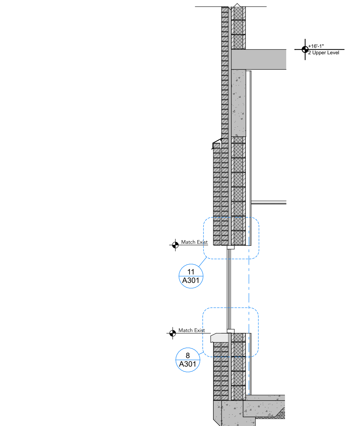
4 Punched Window @ Double Wythe Brick A301 SCALE: 3/8" = 1'-0"
