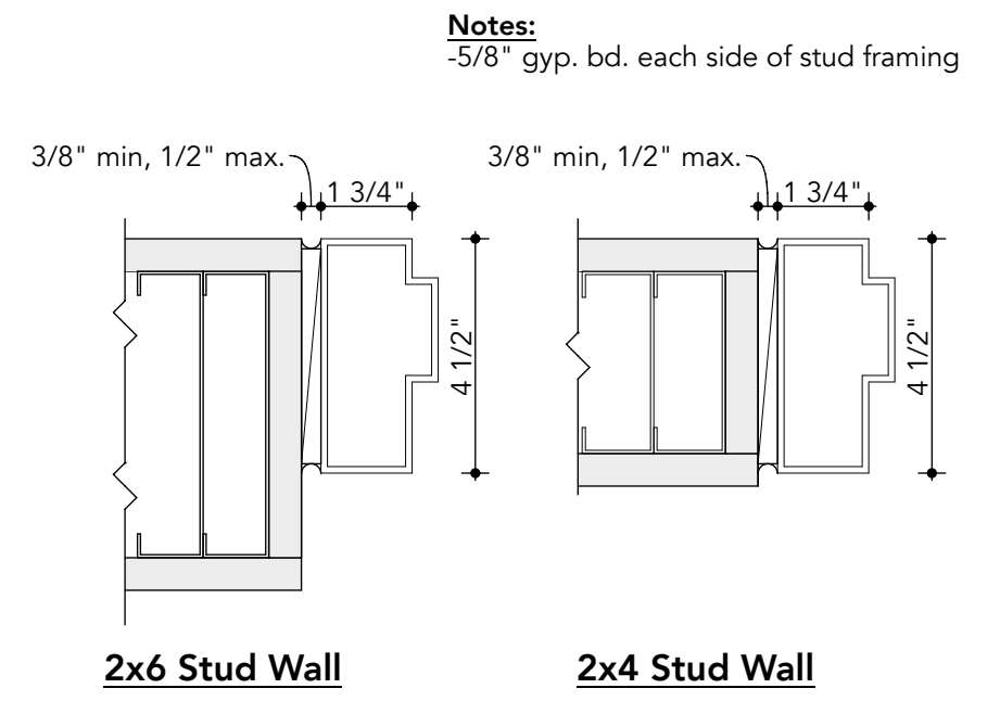
4 Typical Aluminum Frame Jamb Interior A403 SCALE: 3" = 1'-0"
