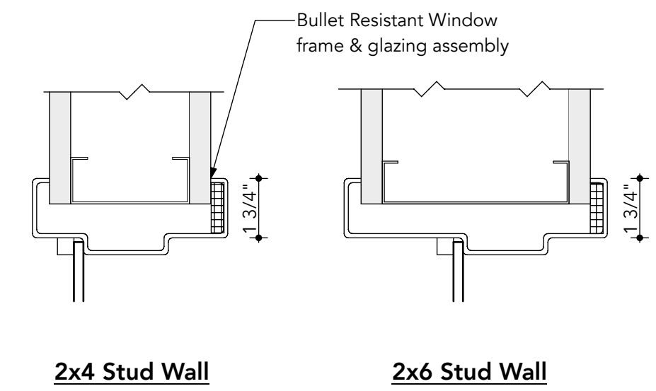
11 Typical HM Window Head Interior A403 SCALE: 3" = 1'-0"
