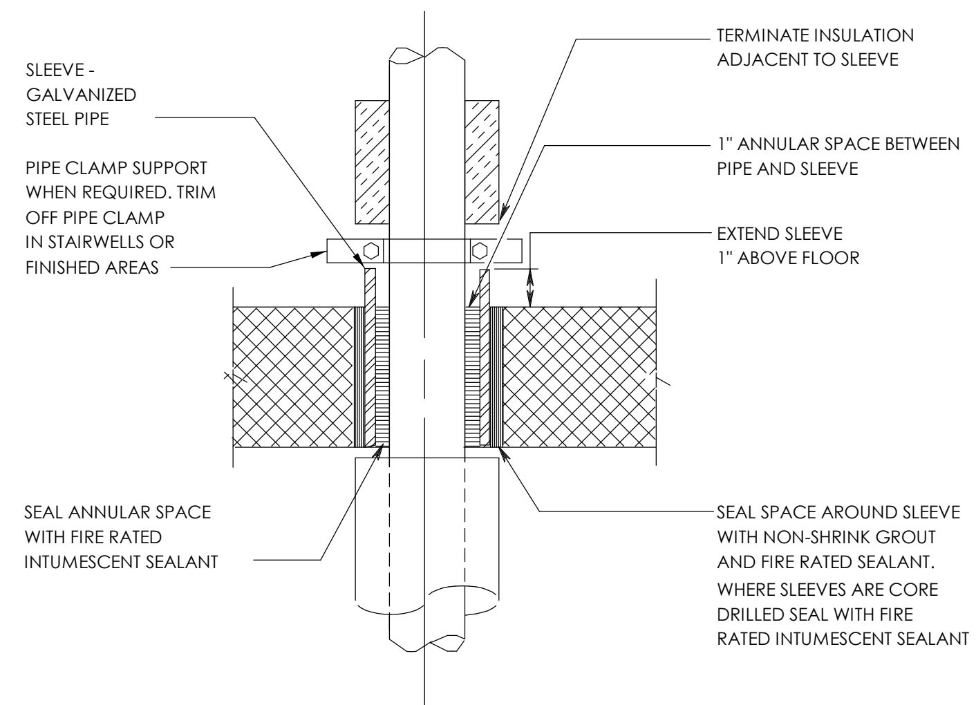
3 P501 PIPE FLOOR SLEEVE DETAIL NOT TO SCALE
