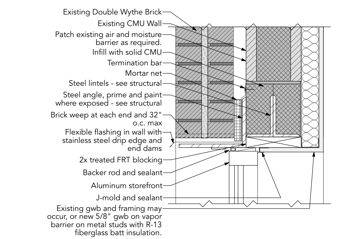
11 FG Fixed Window Head at Double Wythe Brick A301 SCALE: 1 1/2" = 1'-0"
