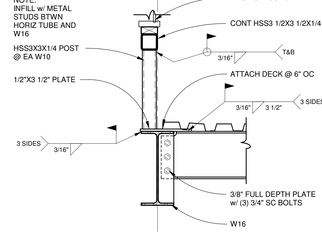
7 S302 FRAMING DETAIL SCALE: 1" = 1'-0"
