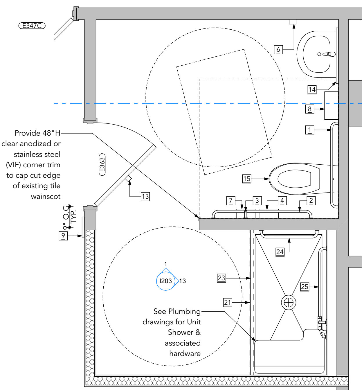
4 Shower Plan #363 - Accessible A106 SCALE: 1/2" = 1'-0"
