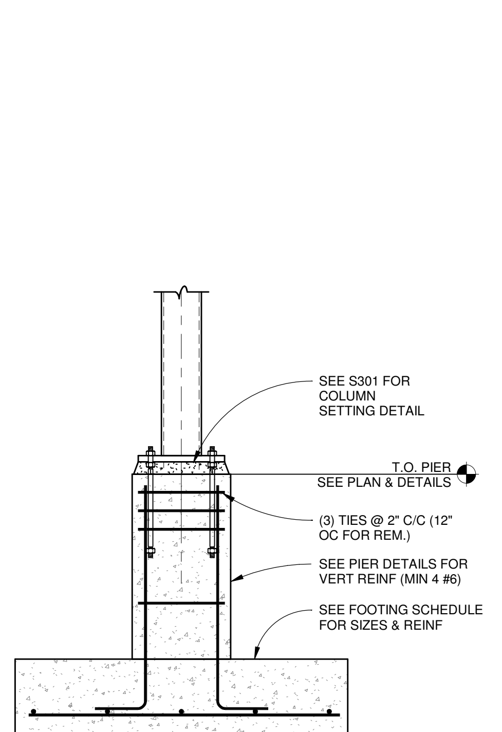
6 S201 PEMB COLUMN DETAIL SCALE: 3/4" = 1'-0"
