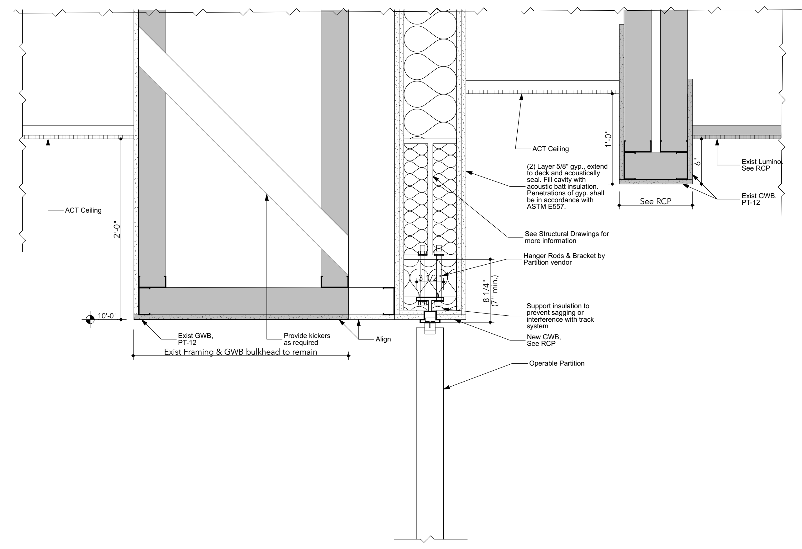
1 Operable Partition Section Detail A114 SCALE: 1 1/2" = 1'-0"
