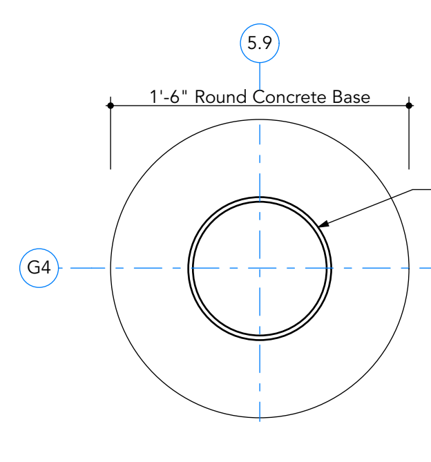
3 Entry Canopy Exterior Column Plan Detail A307 SCALE: 1 1/2" = 1'-0"
