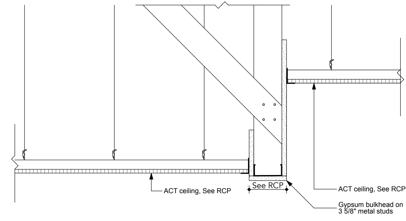
10 Upper Level Lobby to Corridor Transition Detail A113 SCALE: 1 1/2" = 1'-0"
