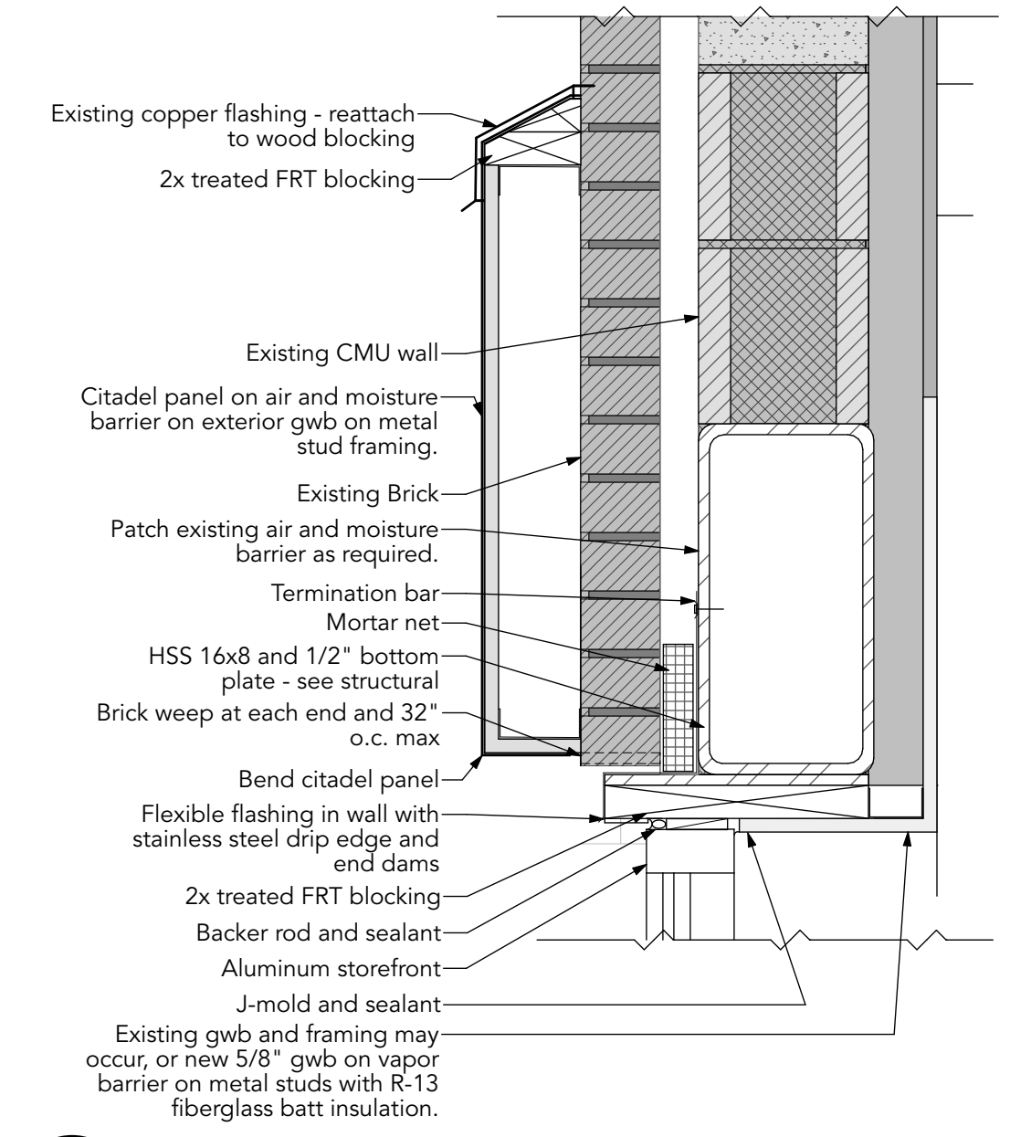
5 Aluminum SF Head at CMU A301 SCALE: 1 1/2" = 1'-0"
