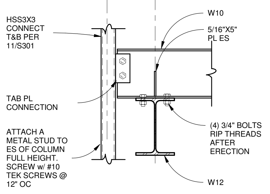
2 S302 FRAMING DETAIL SCALE: 1" = 1'-0"
