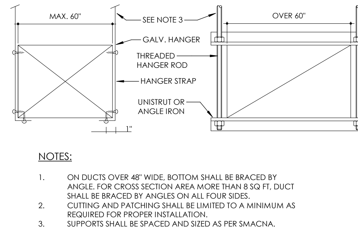
3 DUCT HANGER SUPPORT DETAIL M501 NOT TO SCALE
