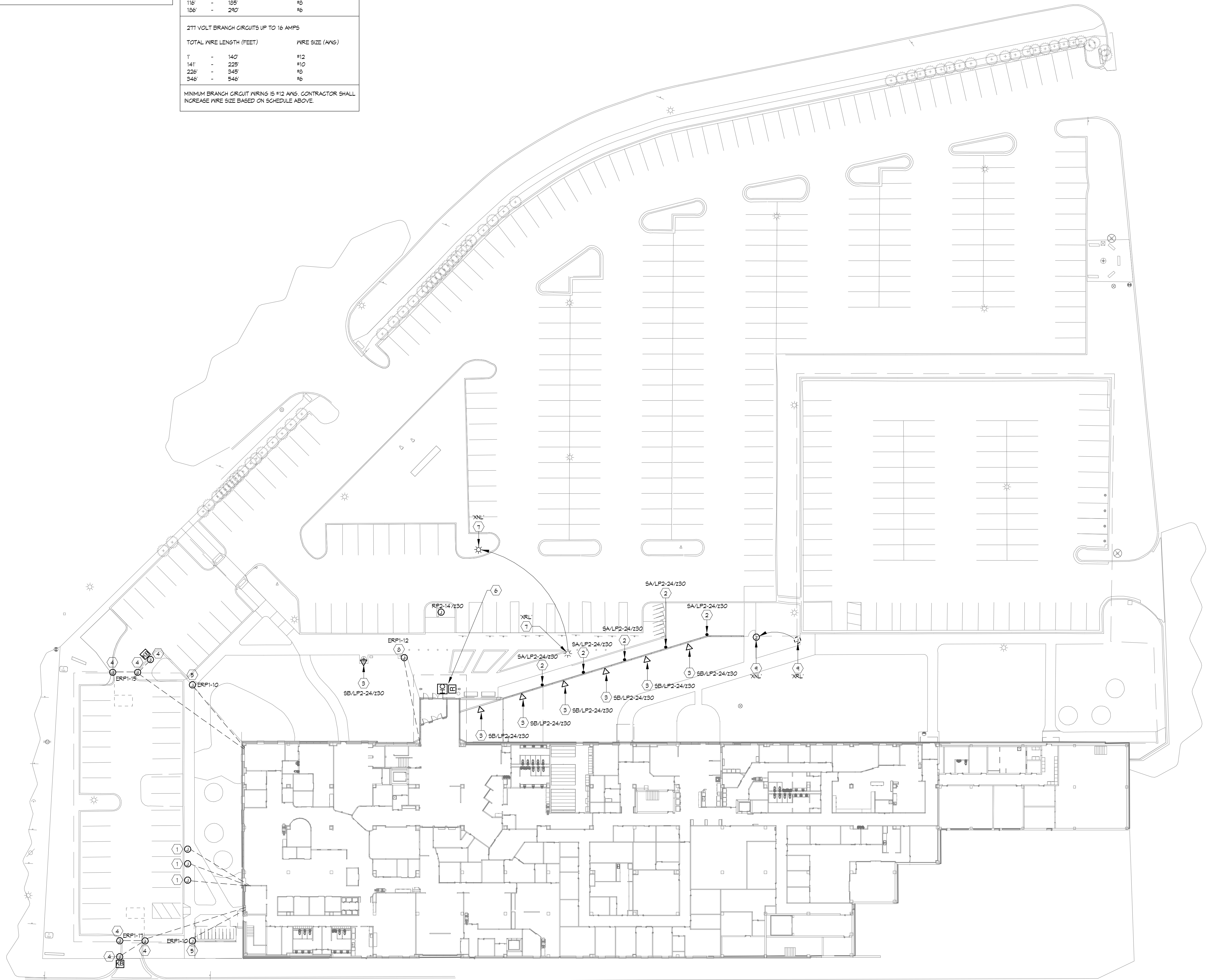
1 ELECTRICAL SITE PLAN ES101 1" = 30'-0"
