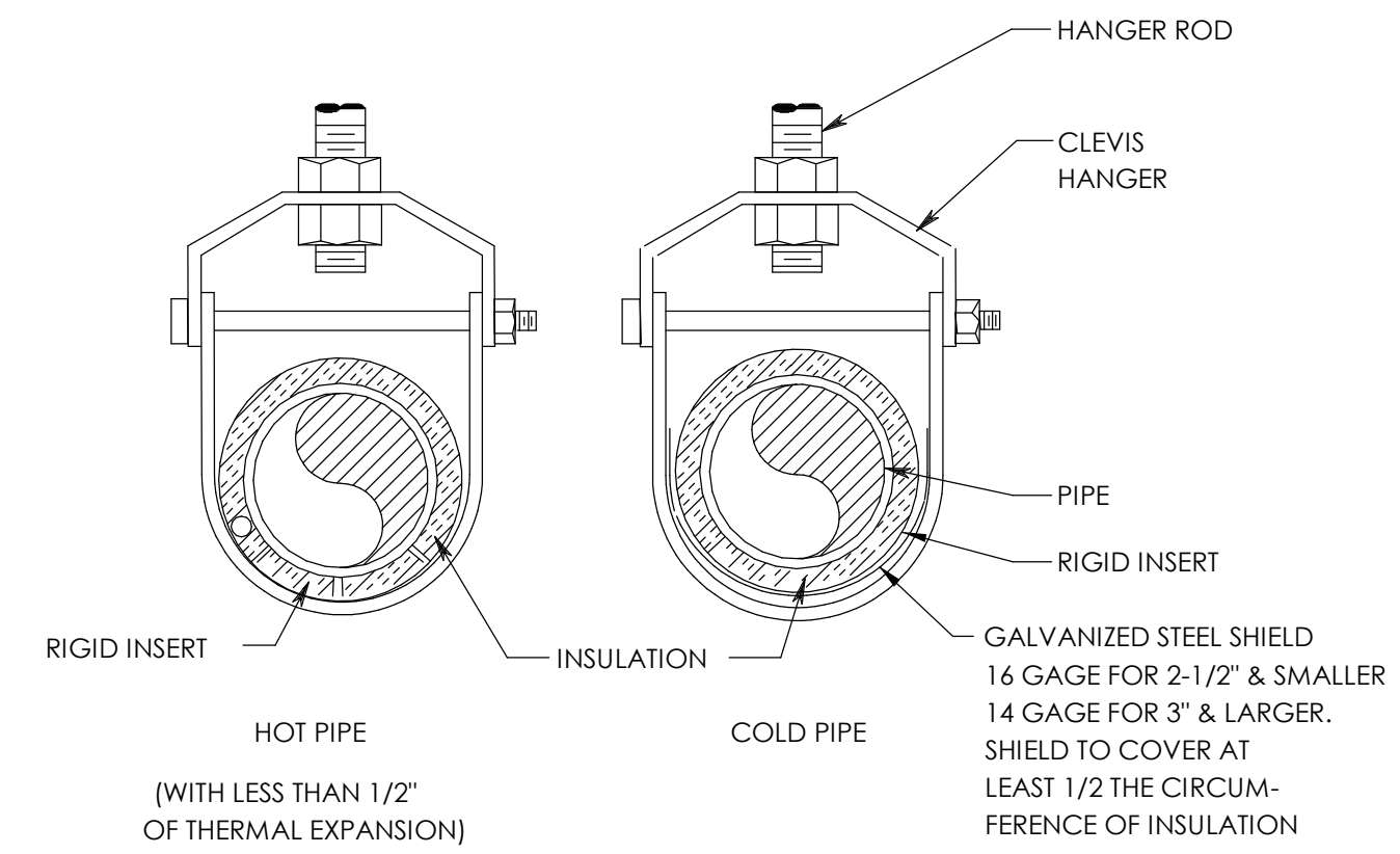
2 P501 INSULATED PIPE HANGER DETAIL NOT TO SCALE
