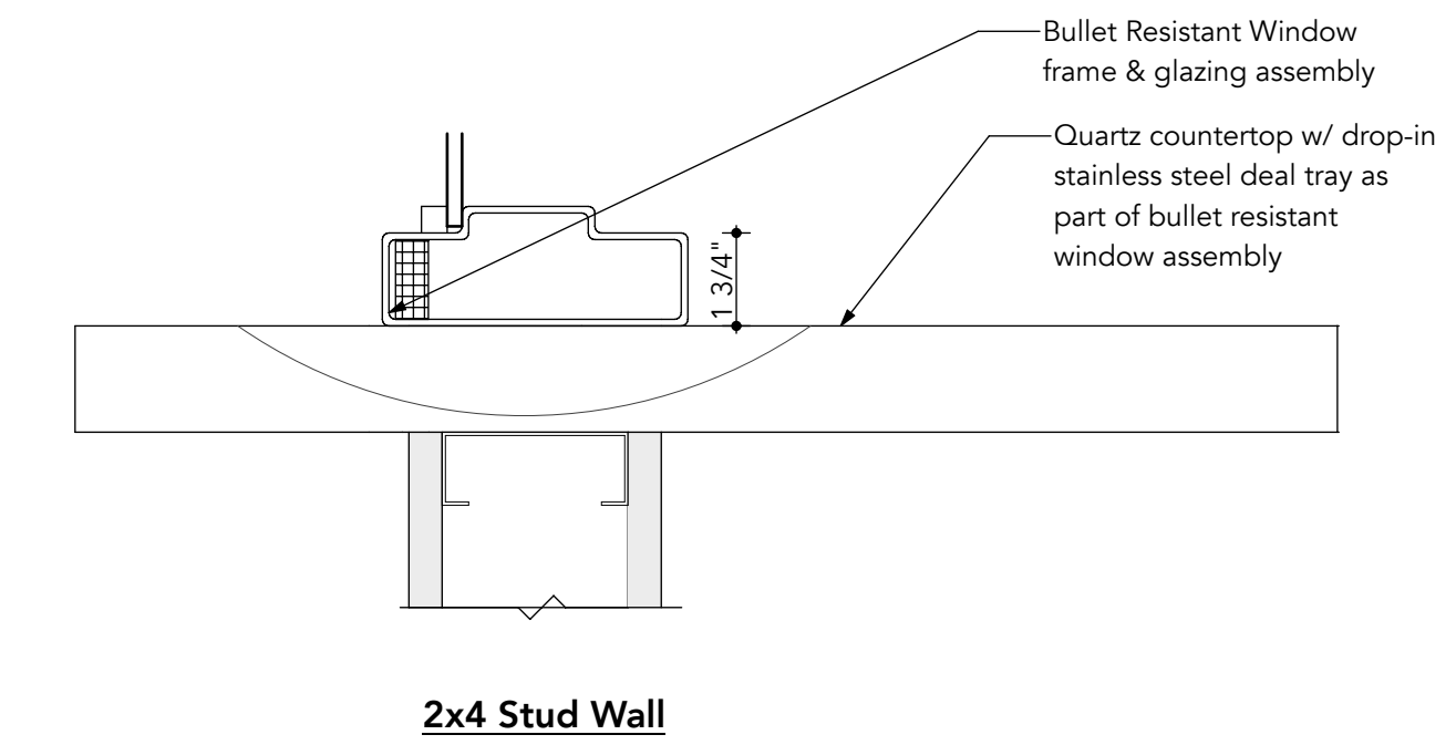
10 Typical HM Window Sill Interior A403 SCALE: 3" = 1'-0"
