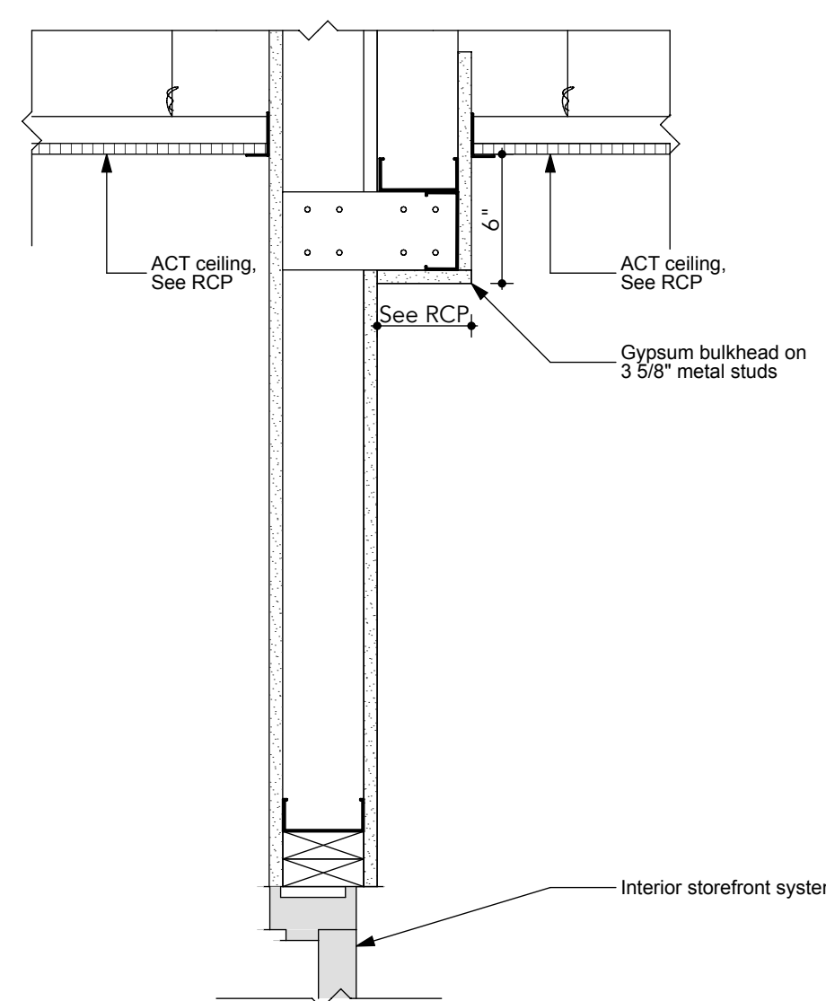
4 Connect 137 to Corridor Transition Detail A113 SCALE: 1 1/2" = 1'-0"
