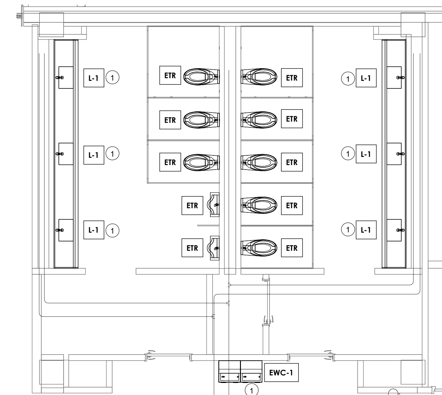
4 UPPER LEVEL CPED NORTH RESTROOM P401 1/4" = 1'-0"
