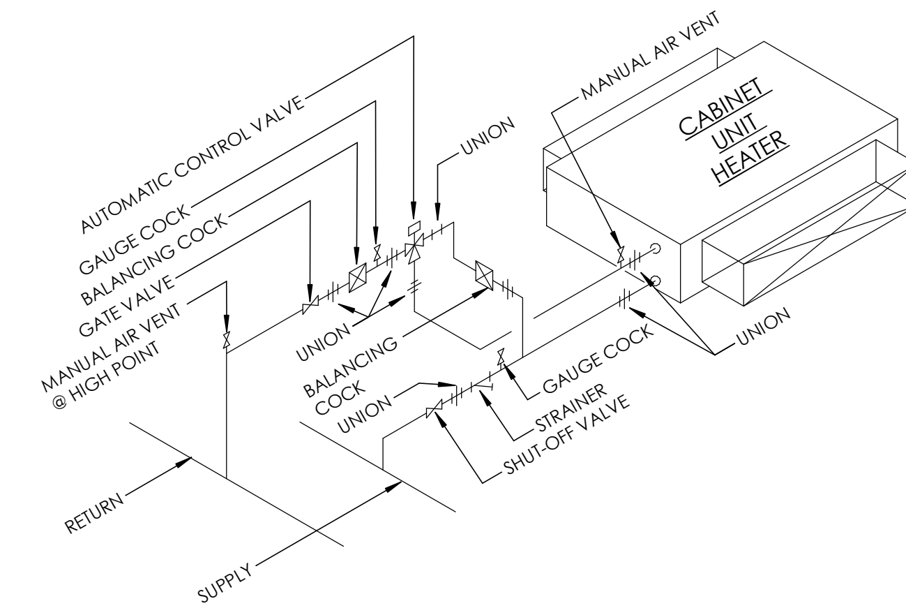
10 CABINET UNIT HEATER PIPING DIAGRAM M501 NOT TO SCALE
