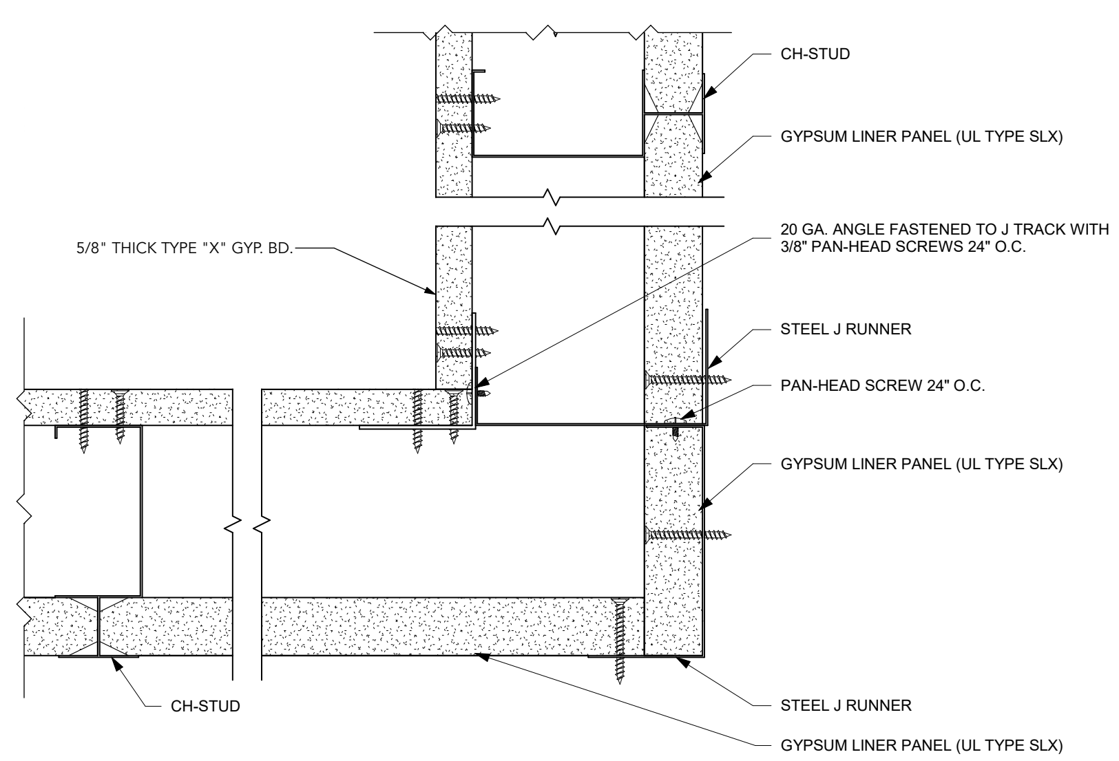
3 Rated Duct Shaft Detail A114 SCALE: 6" = 1'-0"
