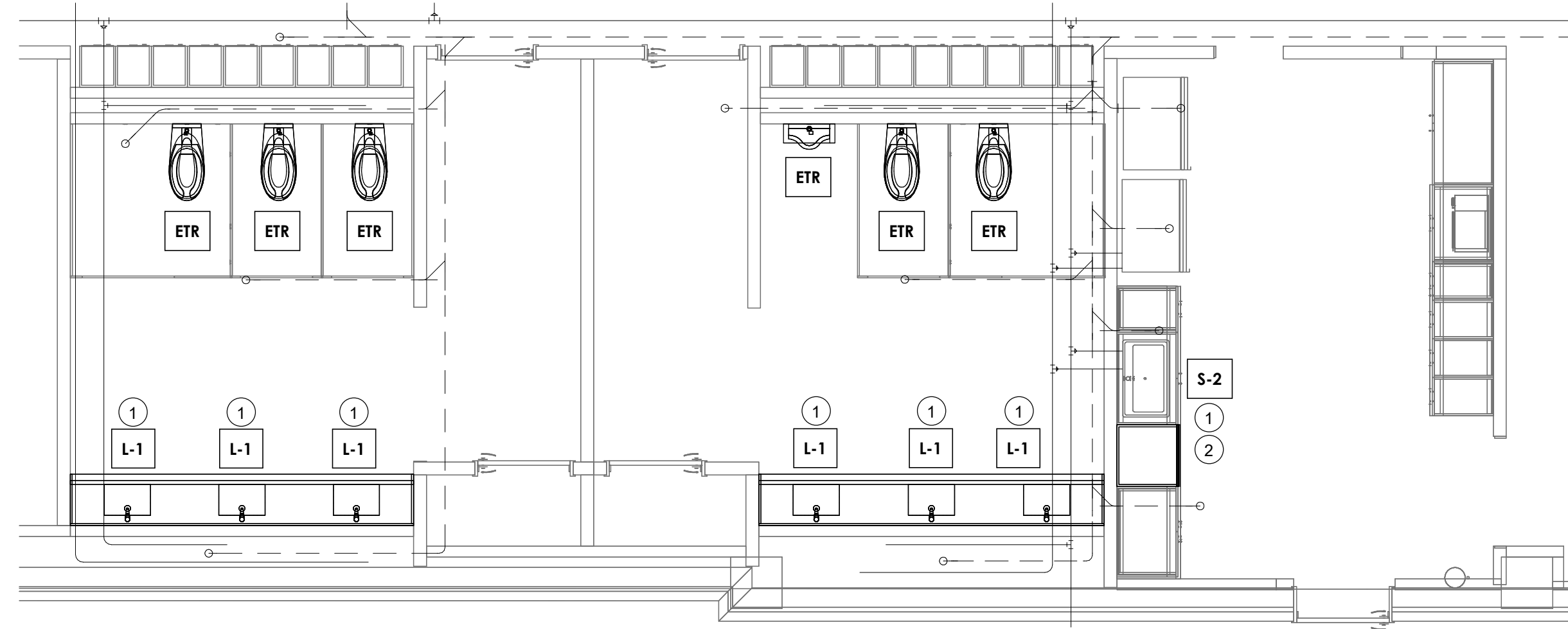
1 MAIN LEVEL CPED SOUTH RESTROOM P401 1/4" = 1'-0"
