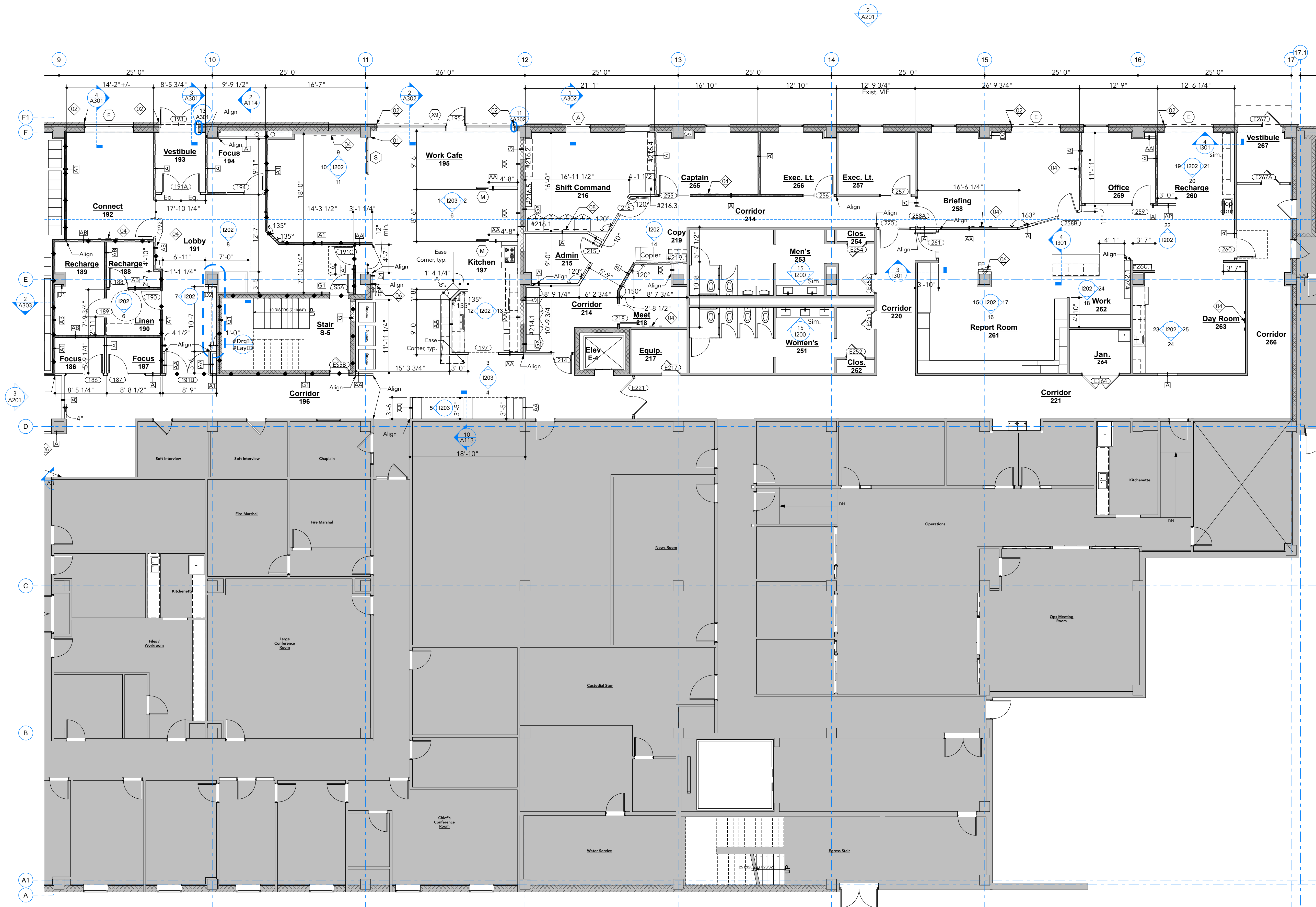
1 Main Level Floor Plan A101 SCALE: 1/8" = 1'-0" N
