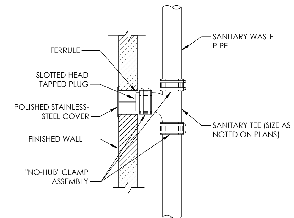
5 P501 WALL CLEANOUT DETAIL 1/8\"/>
