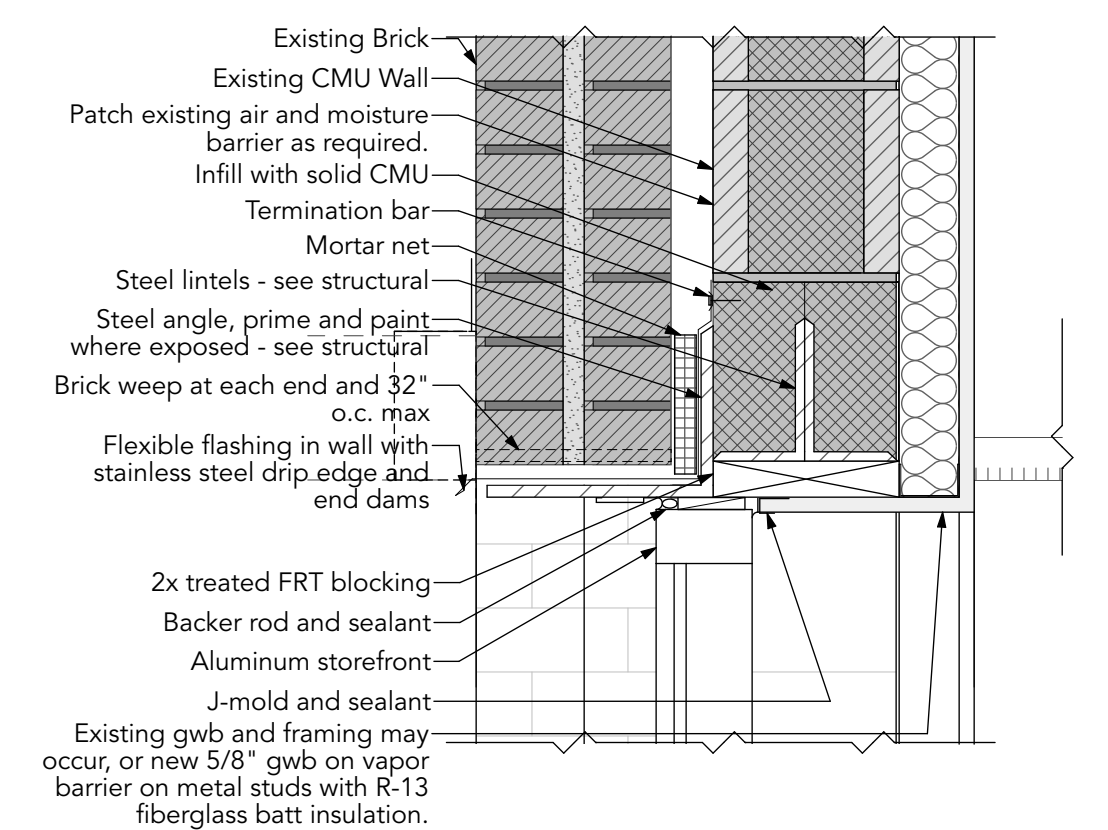
10 Aluminum SF Trans Head A301 SCALE: 1 1/2" = 1'-0"
