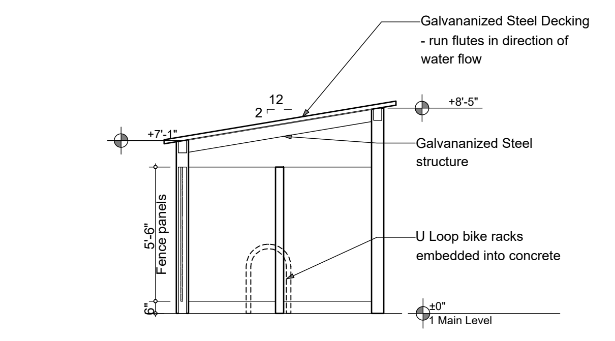
BIKE SHELTER SECTION CS.1 NOT TO SCALE
