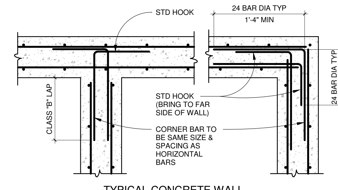
5 S201 TYPICAL CONCRETE WALL CORNER & INTERSECTION REINFORCING DETAILS W/ REINFORCING EA FACE SCALE: 3/4" = 1'-0"
