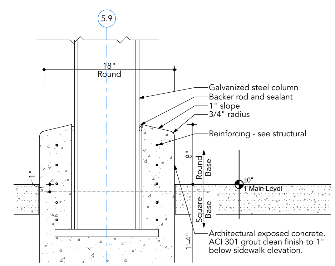
9 Entry Canopy Exterior Column Section Detail A307 SCALE: 1 1/2" = 1'-0"
