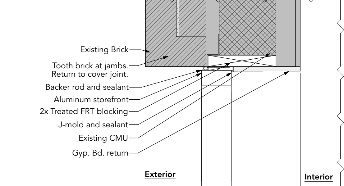
12 Aluminum SF Jamb at Double Wythe Brick A301 SCALE: 1 1/2" = 1'-0"
