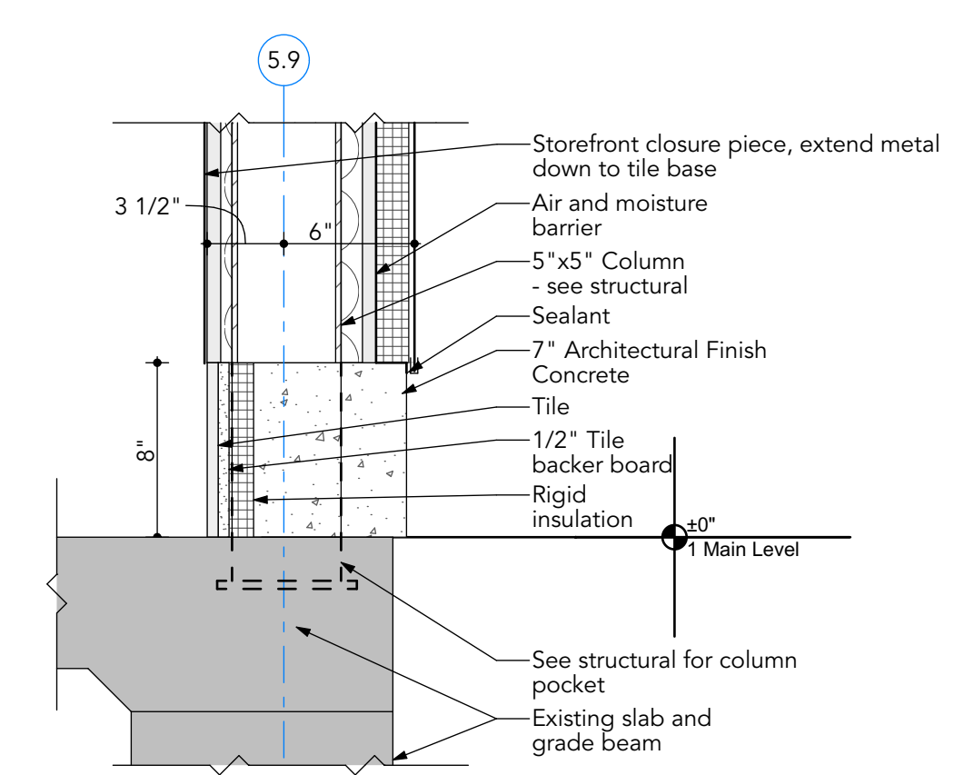
8 Entry Canopy Wall Base @ Column Detail A307 SCALE: 1 1/2" = 1'-0"
