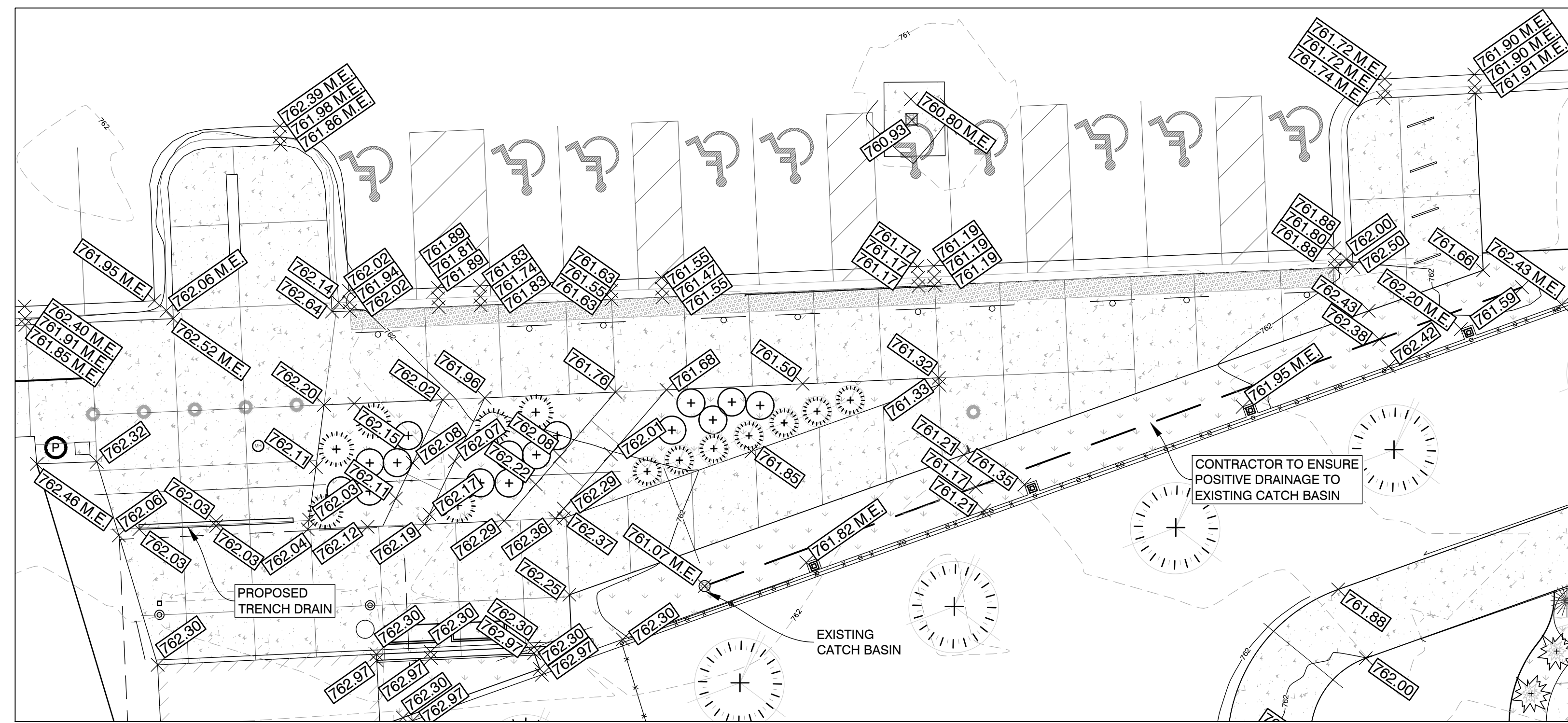
ADA CROSSWALK GRADING DETAIL C3.0 1 INCH = 10 FEET
