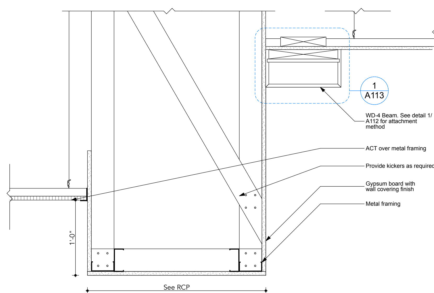
2 Corridor to Lobby Transition Detail A113 SCALE: 1 1/2" = 1'-0"
