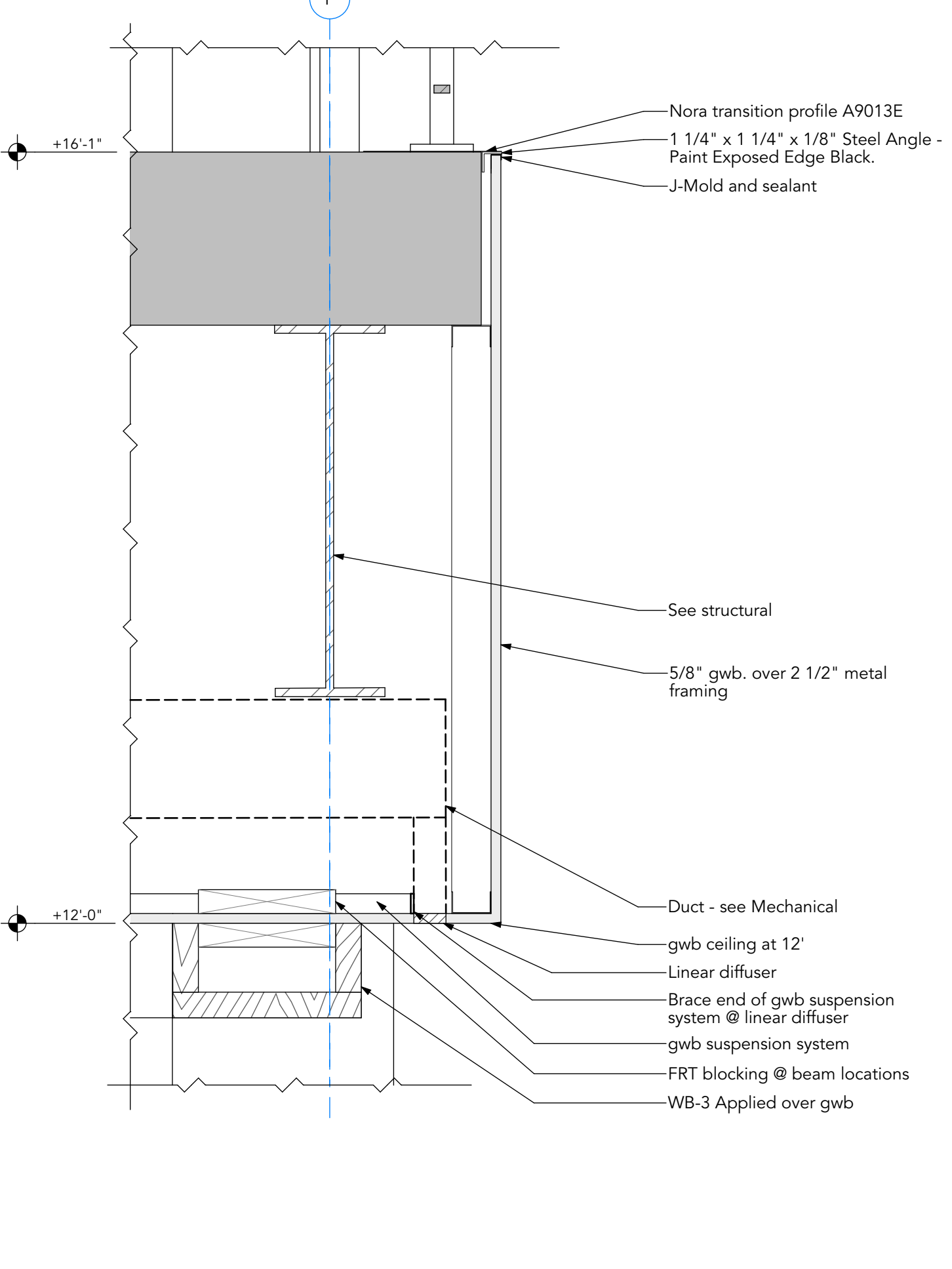
5 Entry Canopy @ Balcony Detail A306 SCALE: 1 1/2" = 1'-0"
