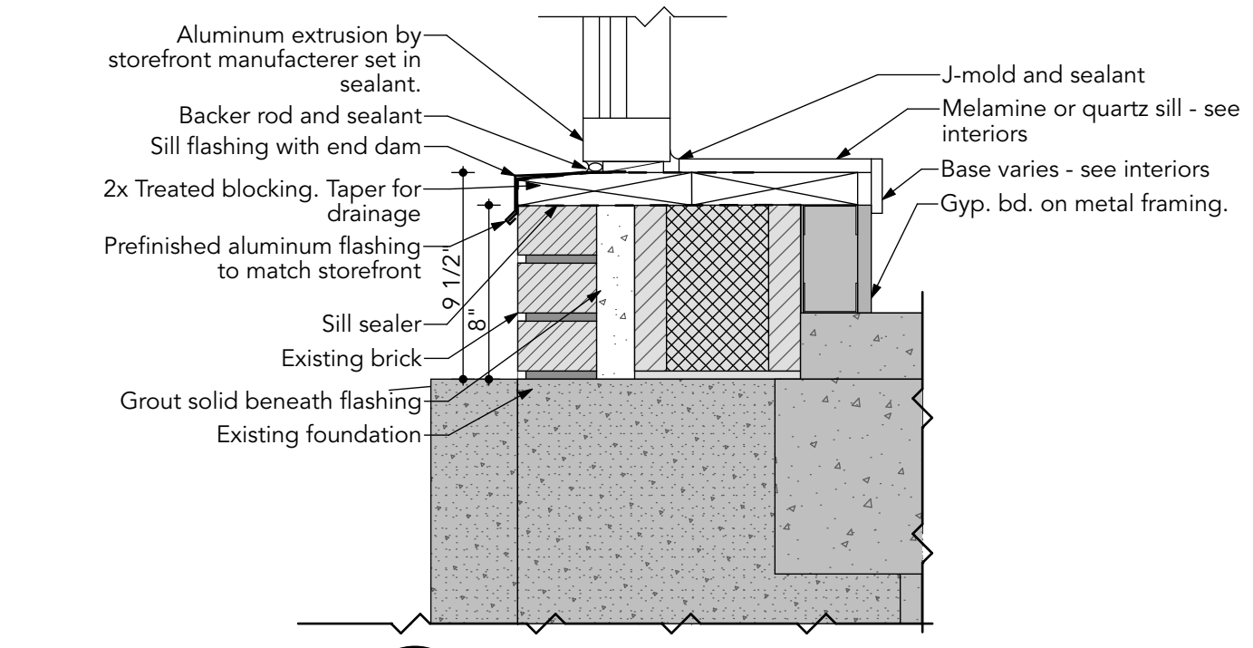
6 Aluminum SF Sill at Floor A301 SCALE: 1 1/2" = 1'-0"
