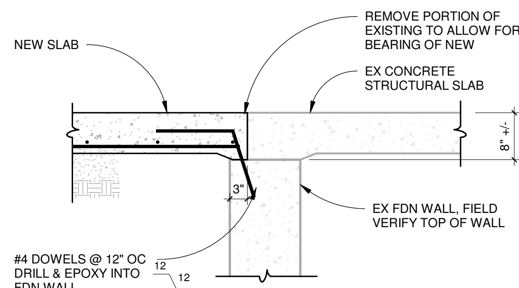
3 S201 DETAIL AT EXISTING WALL SCALE: 3/4" = 1'-0"
