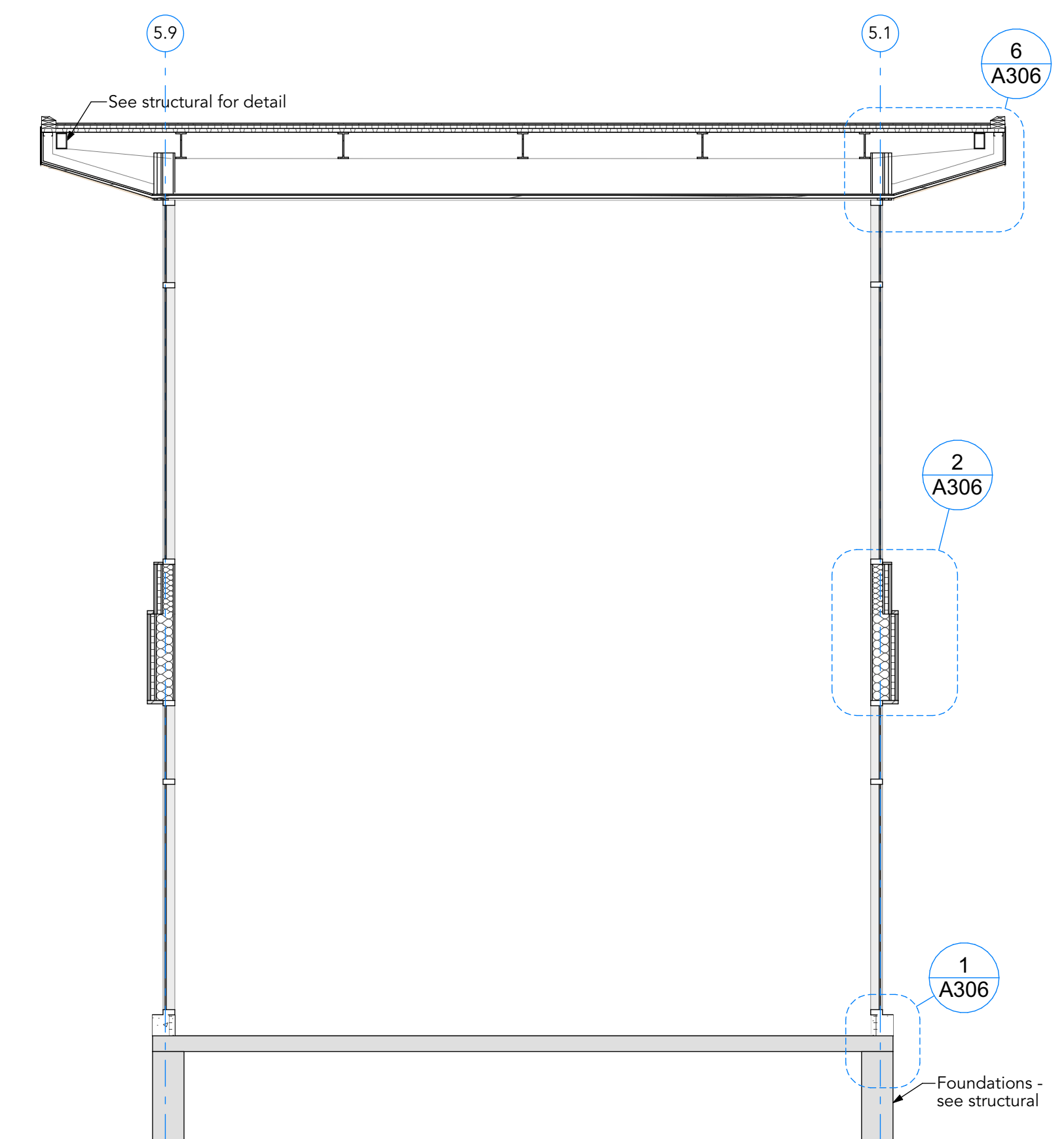
1 Building Section
