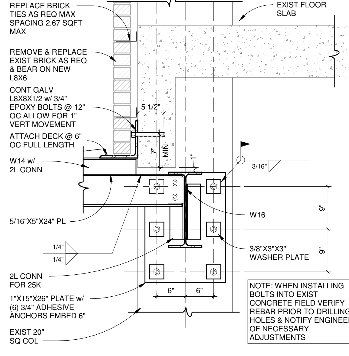
3 S302 FRAMING DETAIL SCALE: 1" = 1'-0"
