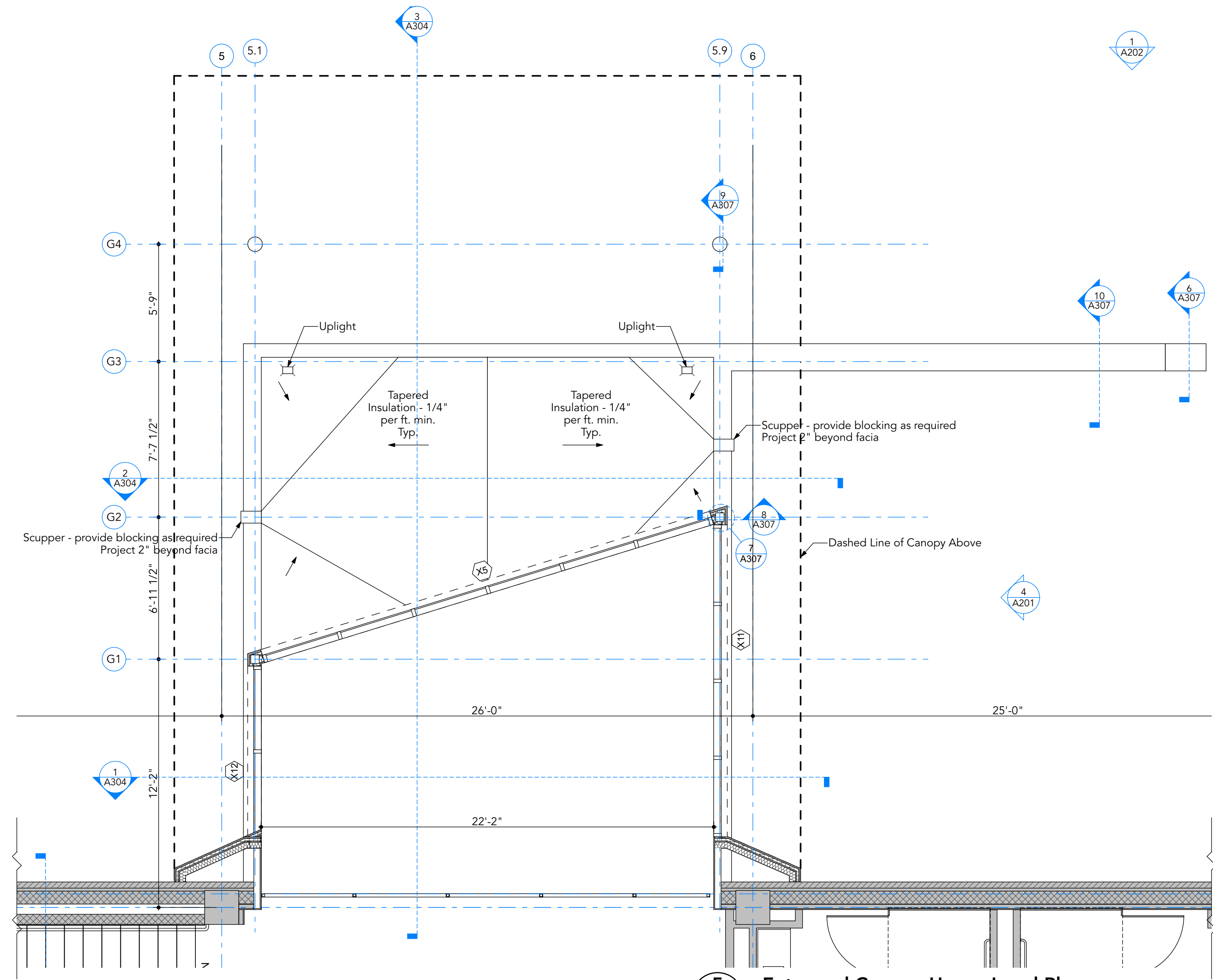
5 Entry and Canopy Upper Level Plan
