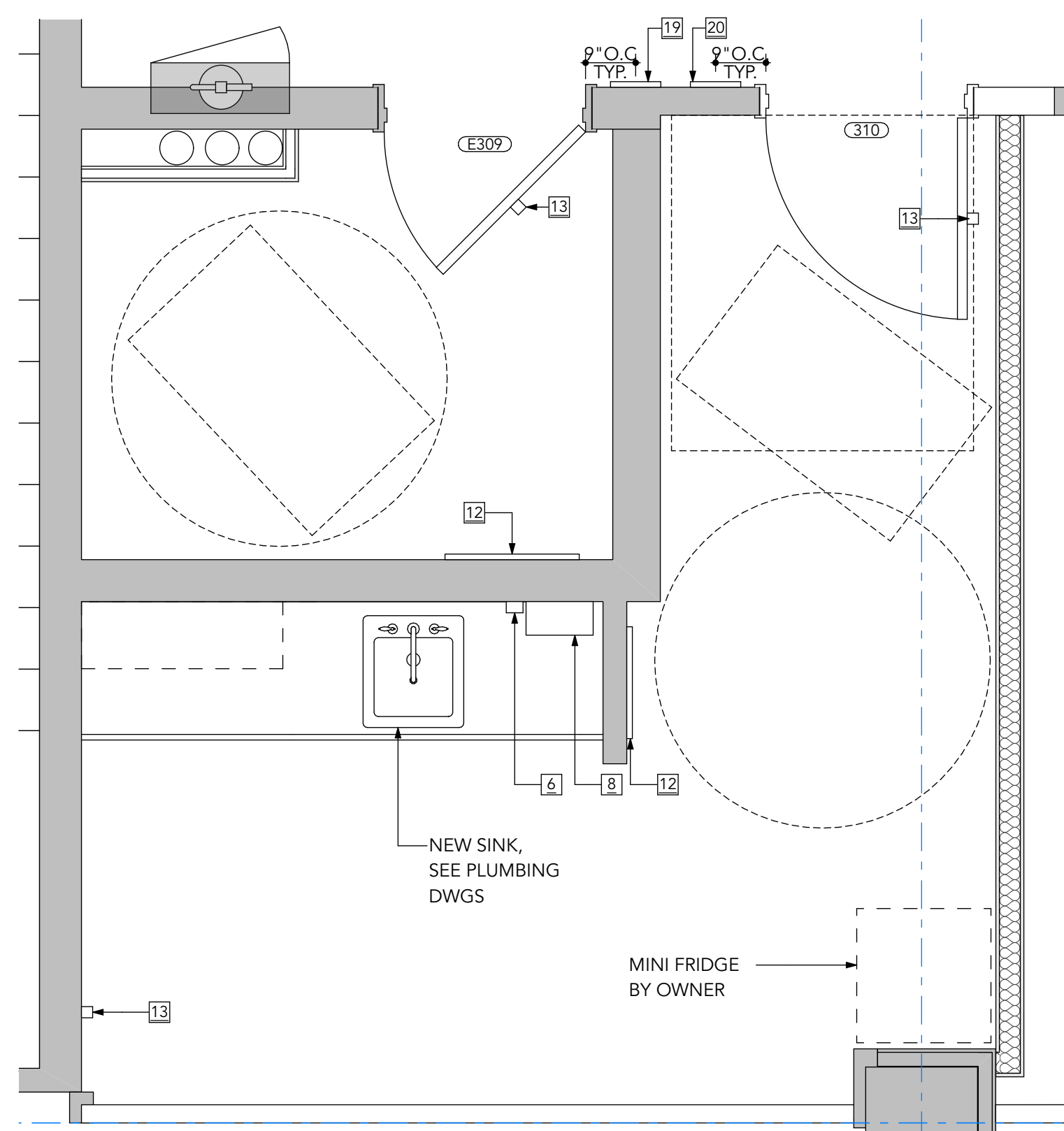
2 Well #309 & Lactation Room #310 A106 SCALE: 1/2" = 1'-0"
