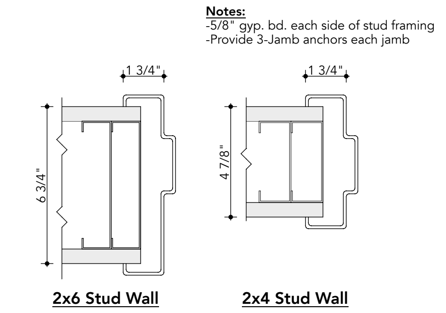
2 Typical HM Frame Jamb Interior A403 SCALE: 3" = 1'-0"
