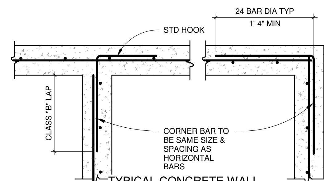
4 S201 TYPICAL CONCRETE WALL CORNER & INTERSECTION REINFORCING DETAILS W/ SINGLE REINFORCING SCALE: 3/4" = 1'-0"
