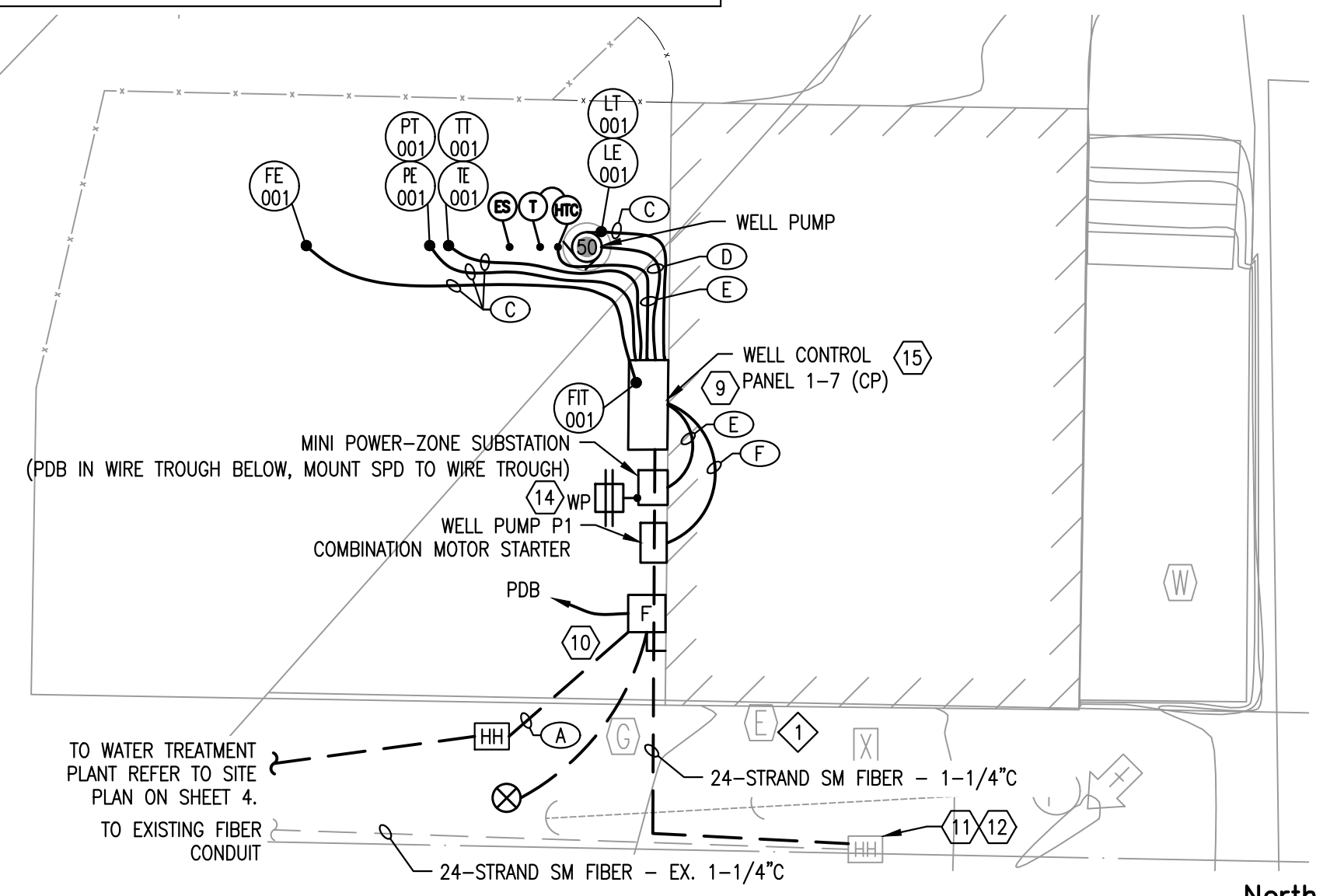
ENLARGED WELLHOUSE ELECTRICAL SITE PLAN - PROPOSED
