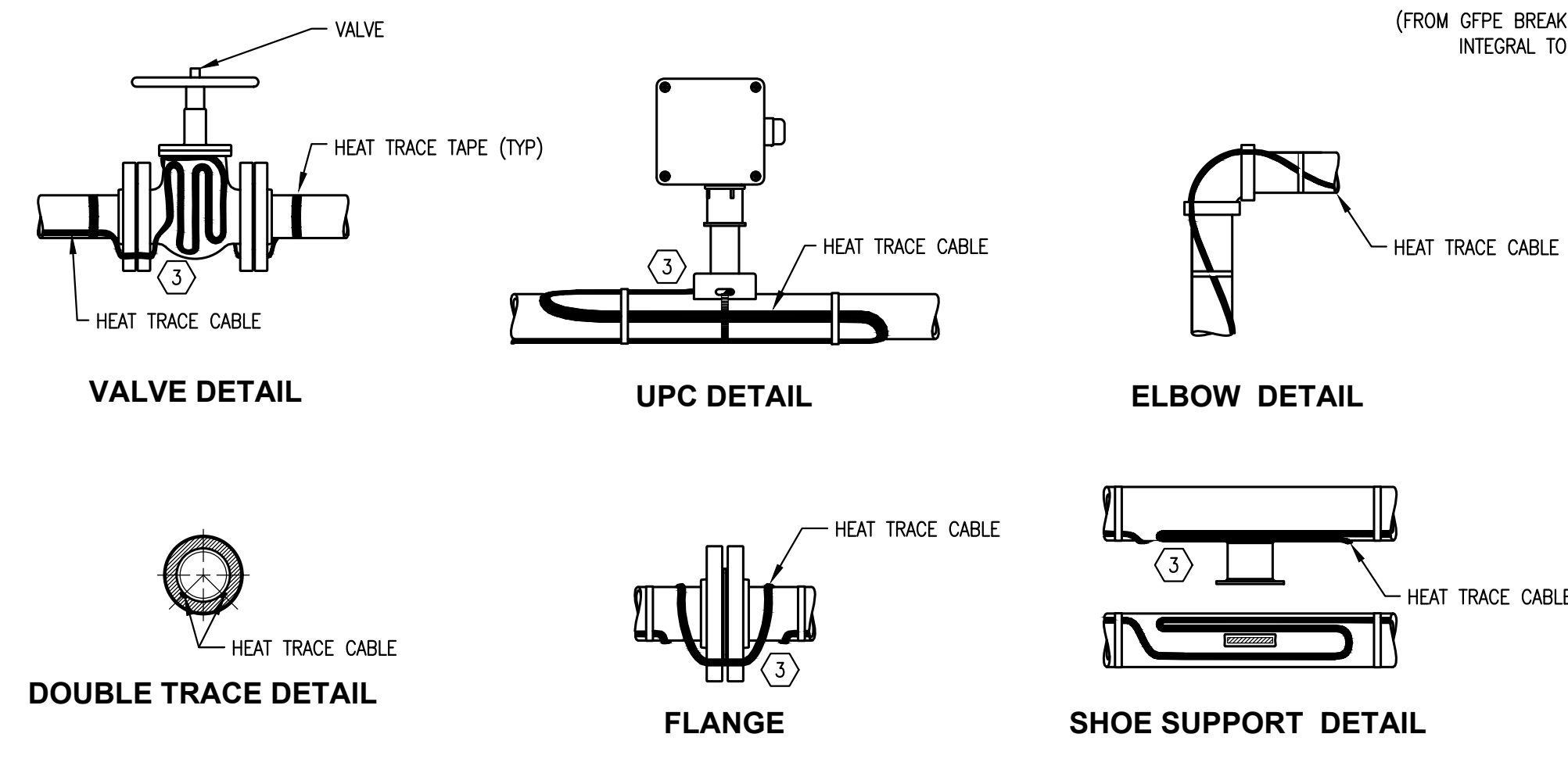
HEAT TRACE INSTALL DETAILS (2/8)
