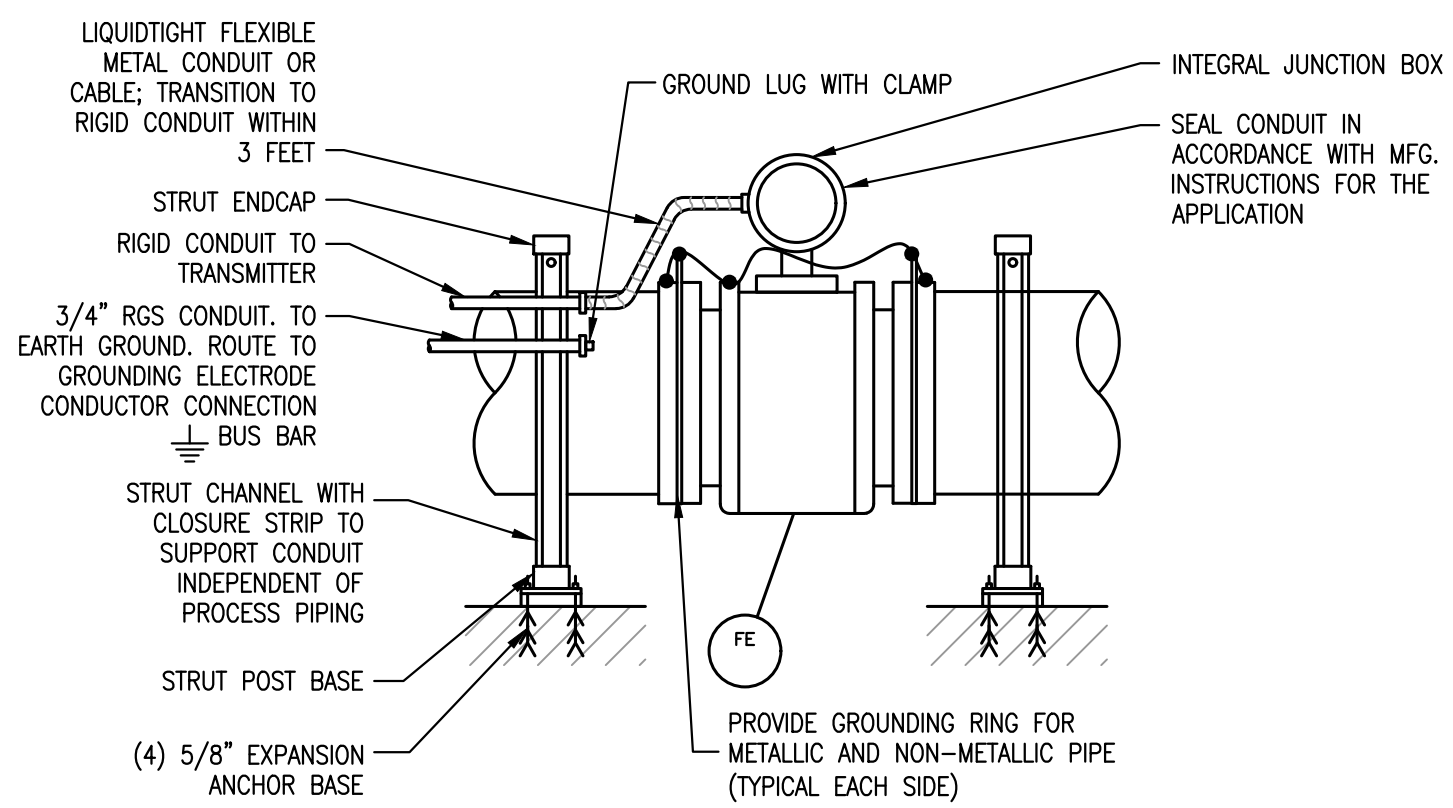
MAGNETIC FLOWMETER INSTALLATION DETAIL (REMOTE TRANSMITTER)
