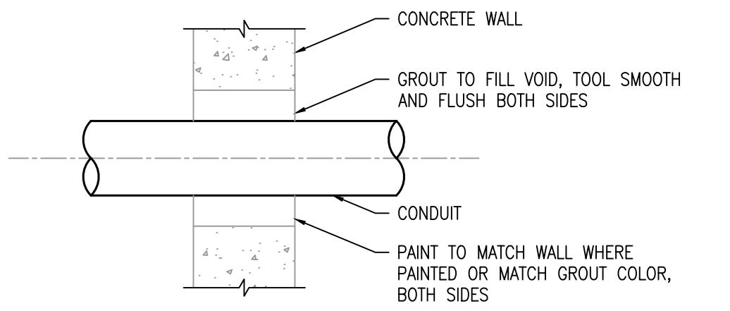
INTERIOR WALL PENETRATION DETAIL SCALE : NONE
