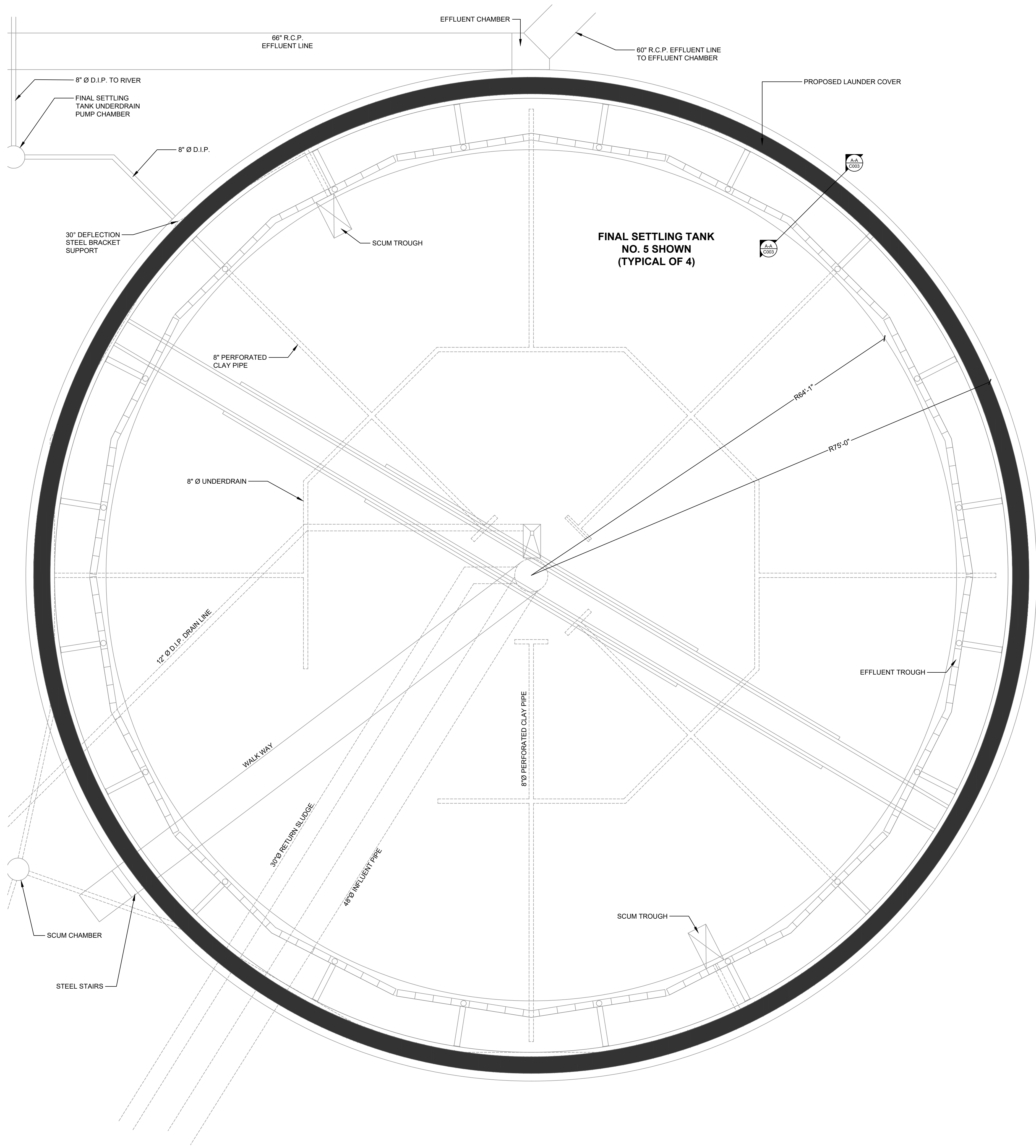
TYPICAL SECONDARY CLARIFIER
