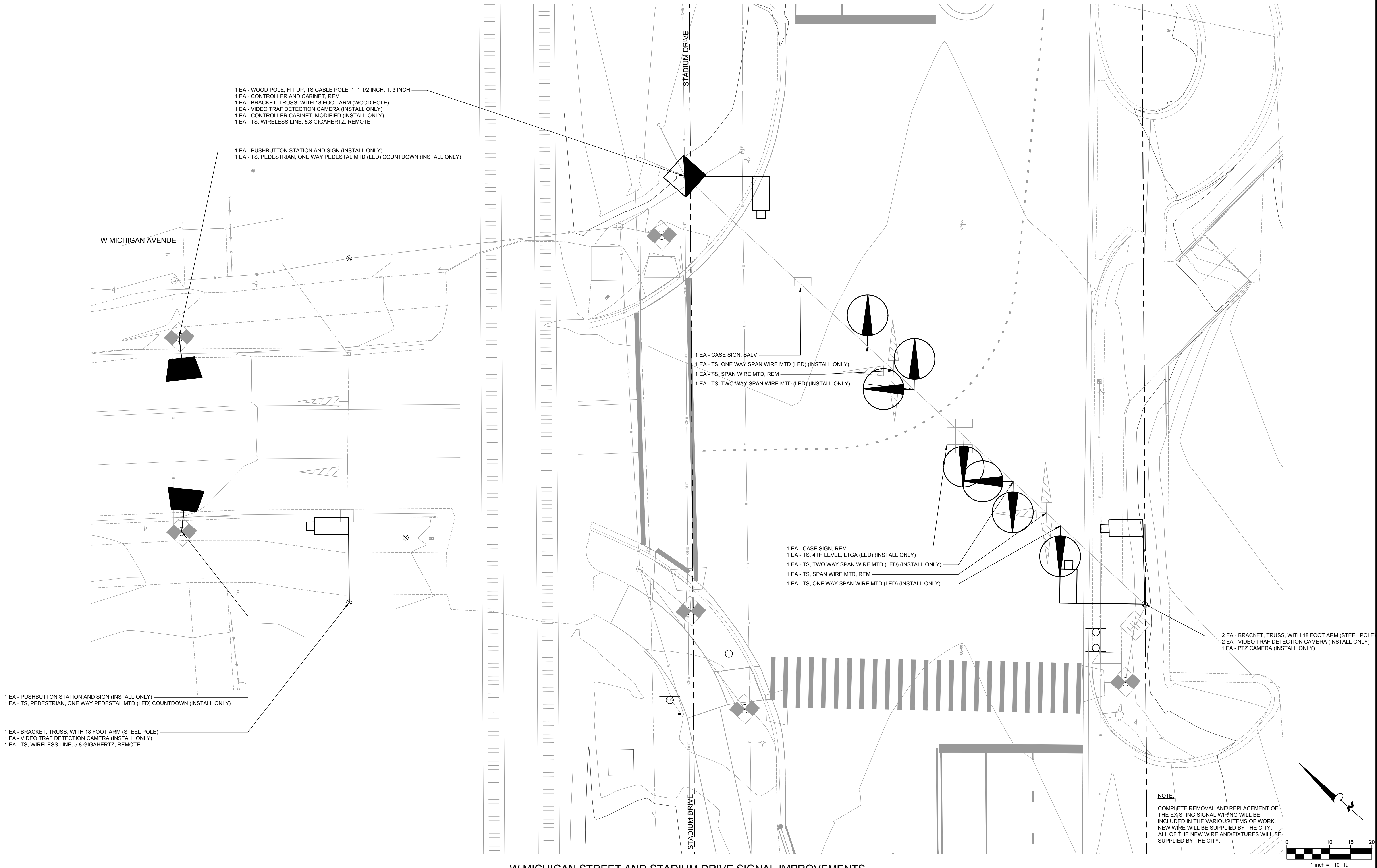
W MICHIGAN STREET AND STADIUM DRIVE SIGNAL IMPROVEMENTS SCALE: 1" = 10'
