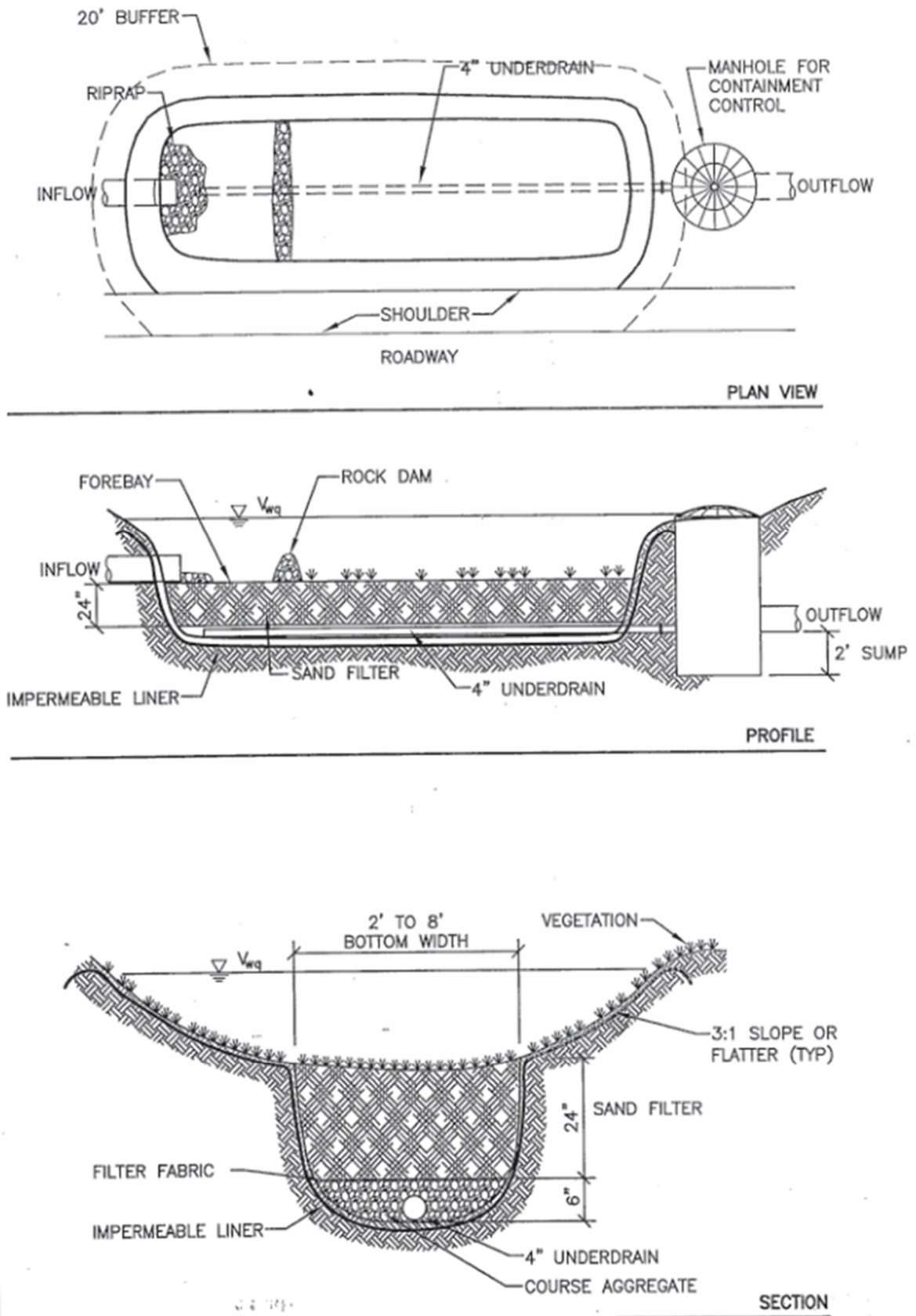
Figure 3: Water Quality Swale
